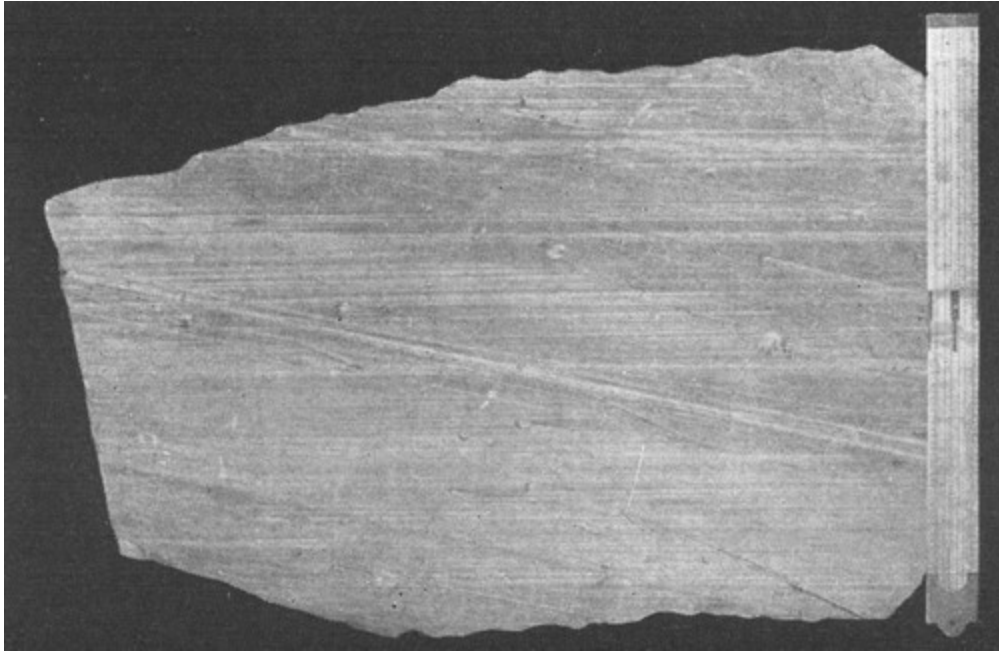
By permission of the American Museum of Natural History Glacial striæ on Lower Helderberg limestone
