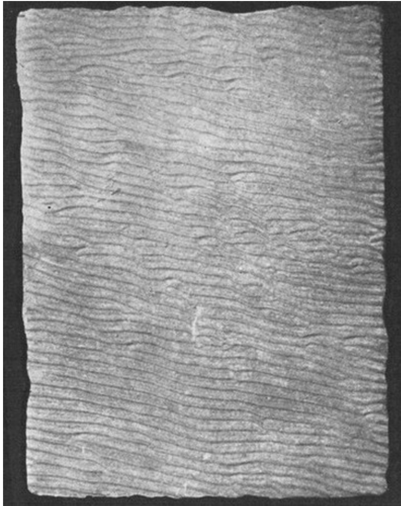
Potsdam sandstone showing ripple marks
