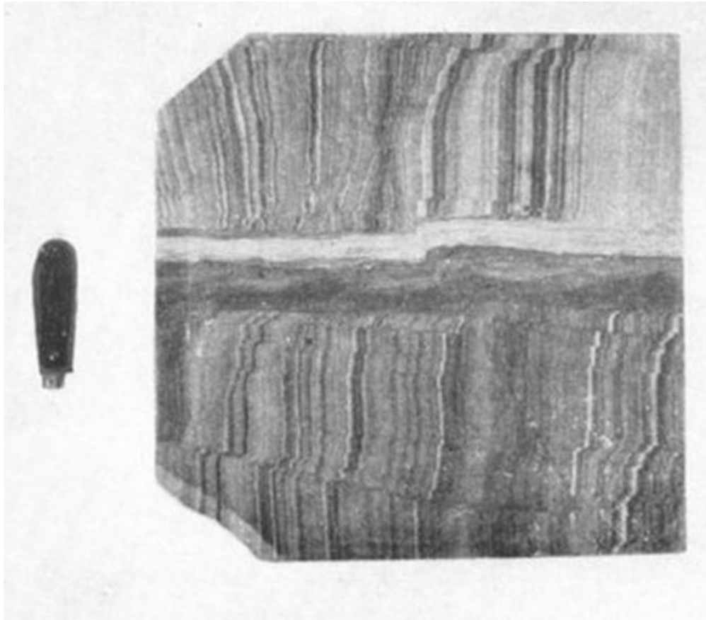
Banded sandstone from Calico Cañon, South Dakota
