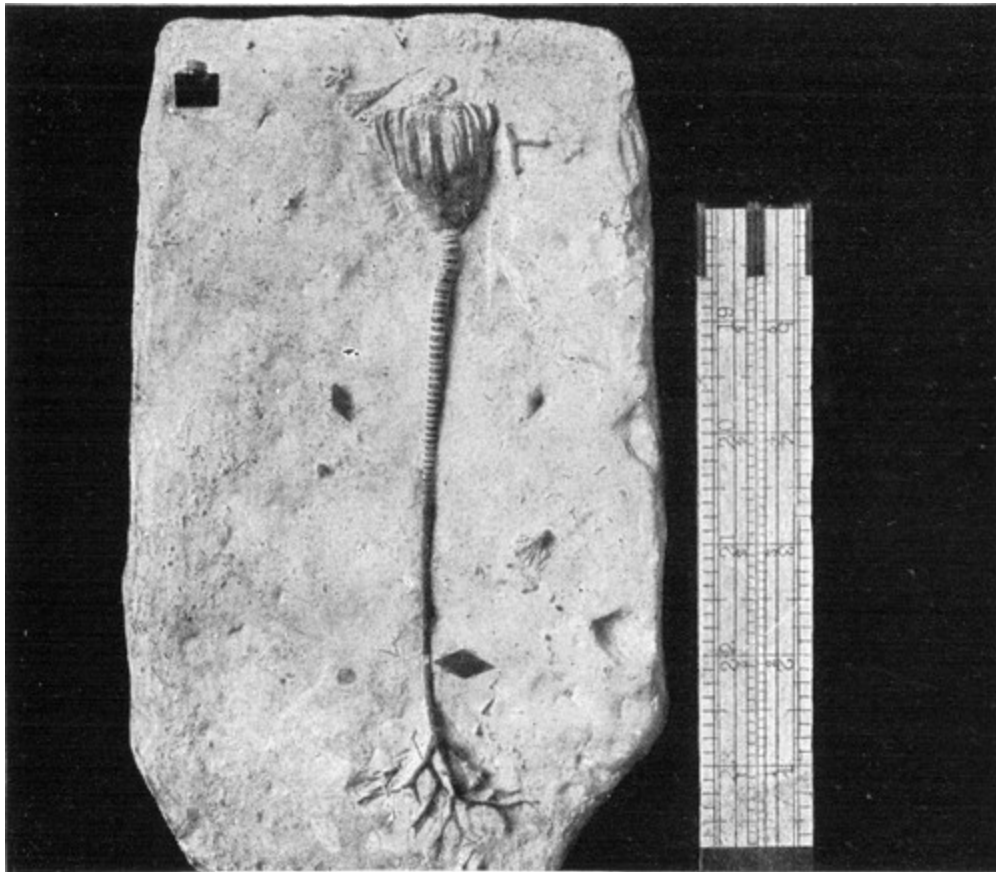
Crinoid from Indiana
