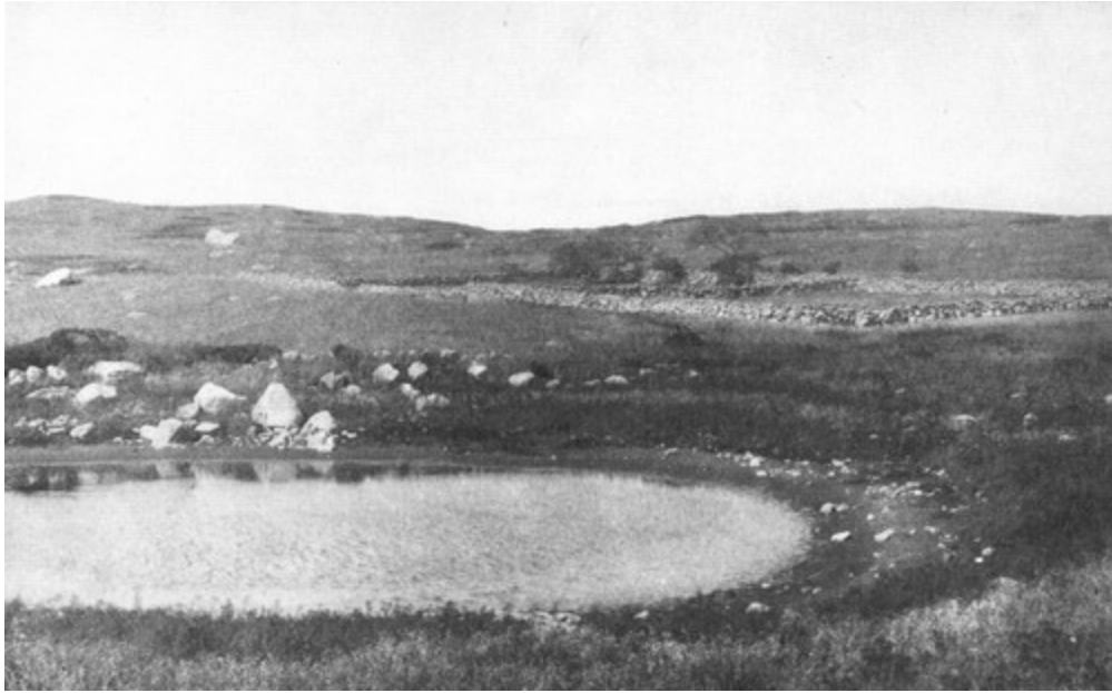
This little pond is a basin hollowed by the same glacier that scattered the stones and rounded the hills
