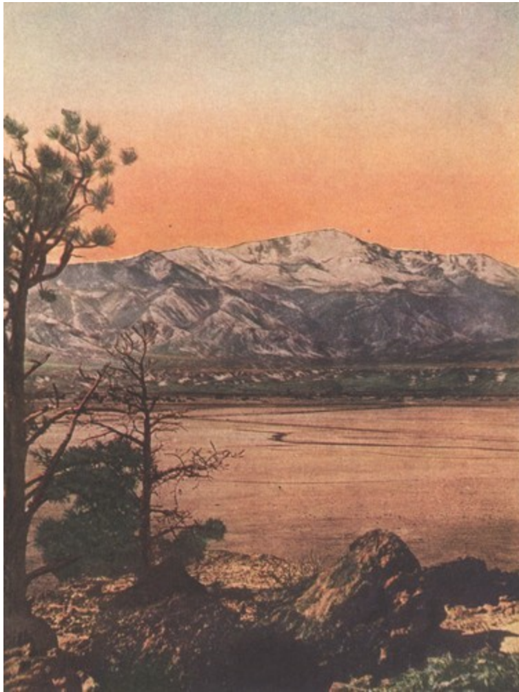
Pike's Peak, Colorado
