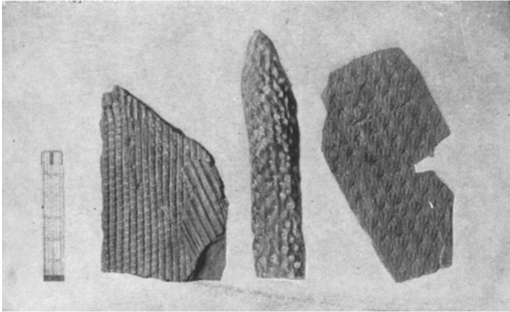
Sigillaria, Stigmaria and Lepidodendron
