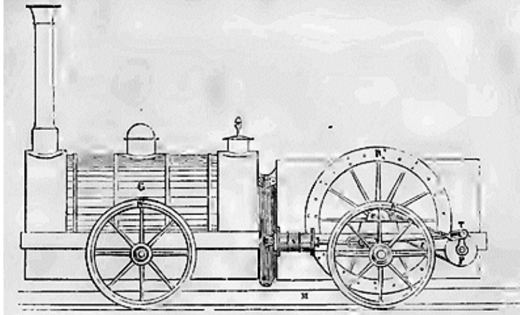
Fig 1.--Elévation de la locomotive.
