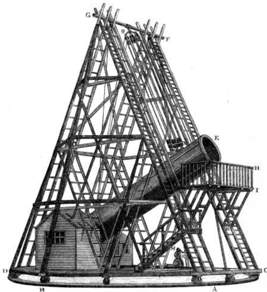
SIR WILLIAM HERSCHEL'S FORTY-FOOT TELESCOPE AT SLOUGH. [To face page 29.]
