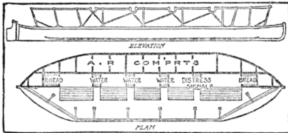
CHAMBERS COLLAPSIBLE LIFE RAFT
