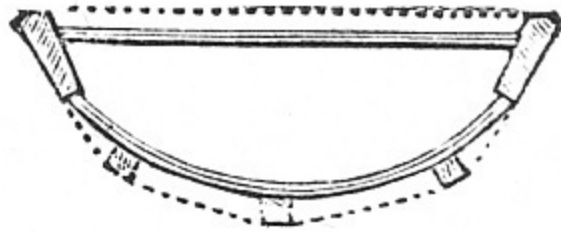
SECTION OF THE KAIKAK (The dotted line represents the skin.)
