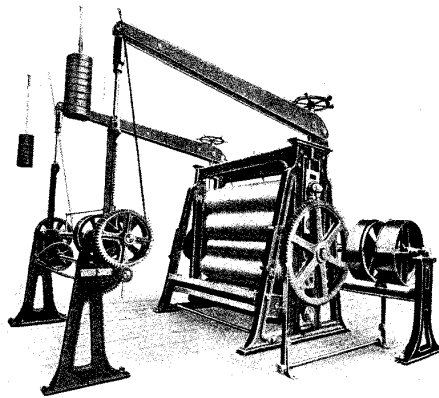
FIG. 44 CALENDAR
