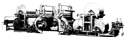
FIG. 31 DRESSING MACHINE FOR PREPARING TWO WARPS SIMULTANEOUSLY
