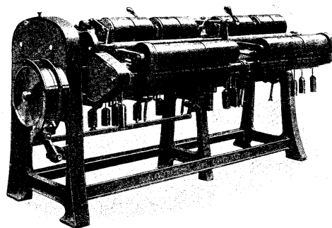
Fig. 17 PUSH-BAR DRAWING FRAME
