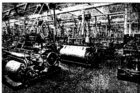
FIG. 35 WEAVING SHED WITH BELT-DRIVEN LOOMS
