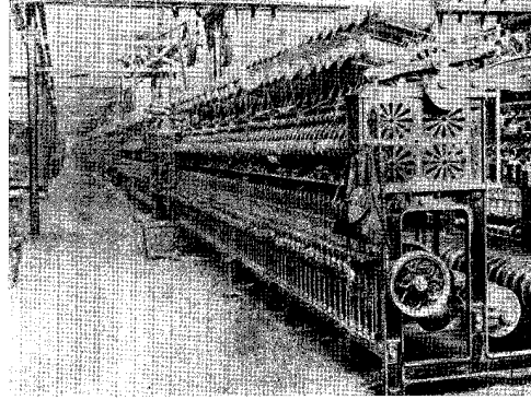
FIG. 21 A LINE OF SPINNING FRAMES
