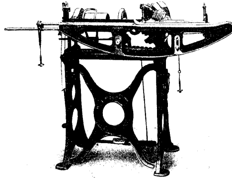
FIG. 49 OVERHEAD (LAING) SACK SEWING MACHINE
