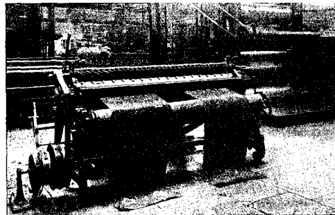
FIG. 41 CROPPING MACHINE AT WORK
