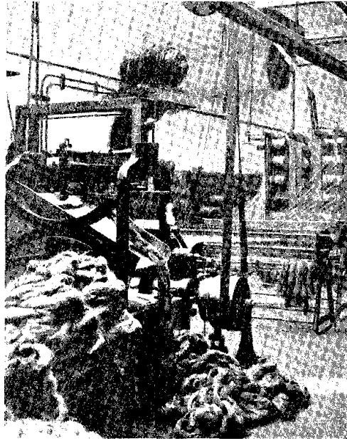
FIG. 28 POWER CHAIN OF WARP LINKING MACHINE
