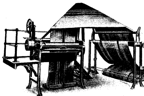
FIG. 47 CRISPING, CREASING OR RIGGING MACHINE
