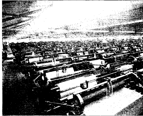
FIG. 36 LOOMS DRIVEN WITH INDIVIDUAL MOTORS
