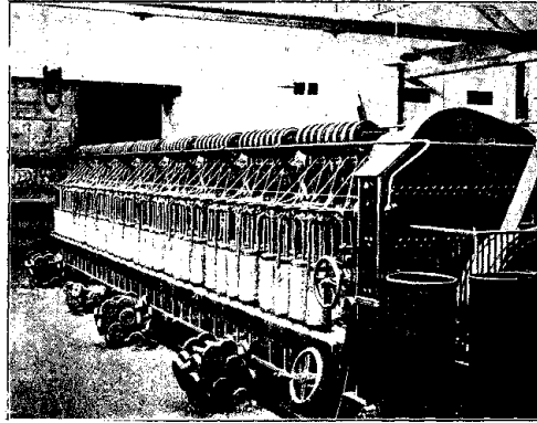
FIG. 19 ROVING FRAME FAIRBAIRN'S ROVING FRAME IN WORK
