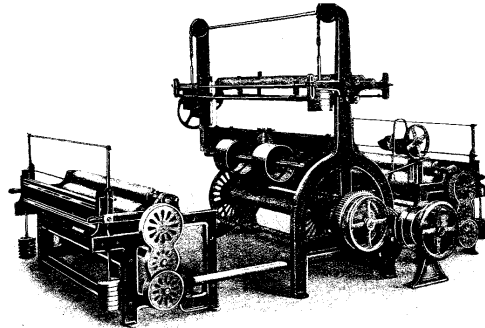
FIG. 29 WINDING-ON OR DRY BEAMING MACHINE
