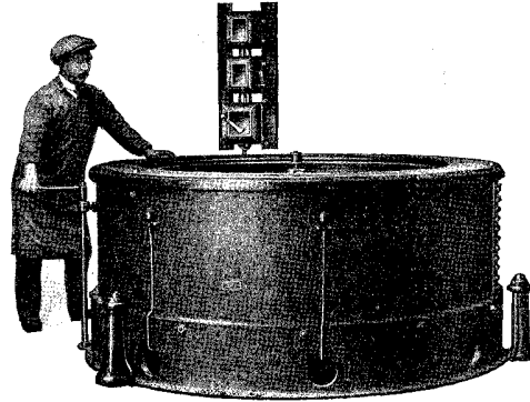
72" Electrically-Driven Hydro-Extractor.—Type No. 4
