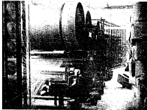
FIG. 30 A MODERN YARN DRESSING MACHINE WITH SIX STEAM-HEATED CYLINDERS
