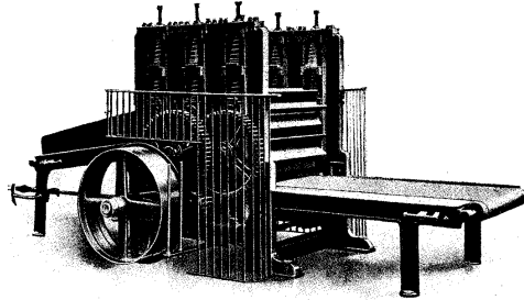
FIG. 8 BALE OPENER
