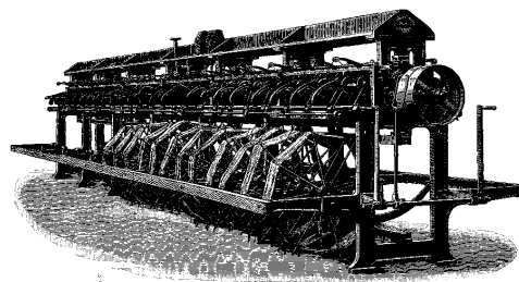
FIG. 22 BOBBIN WINDING MACHINE WITH HANKS
