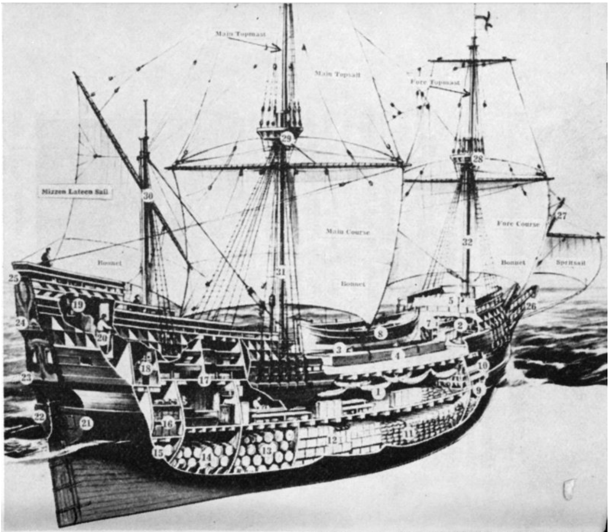
A CUTAWAY DRAWING of the original Mayflower by John Seamans of Weymouth, Mass., from plans drawn by William A. Baker, Hingham marine architect and authority on ancient ships.
