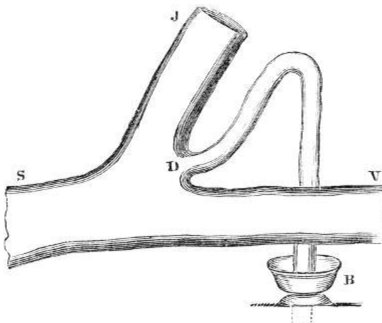
SHOWING PRINCIPLE OF VENTURI.
