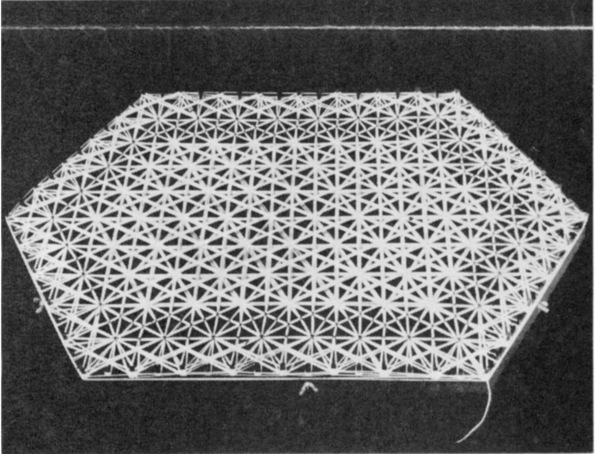
Frame completely wound—for twelve-petal daisy design. (This illustration shows frame extended for buffet or vanity set centerpieces—or centerpieces for luncheon set.)
