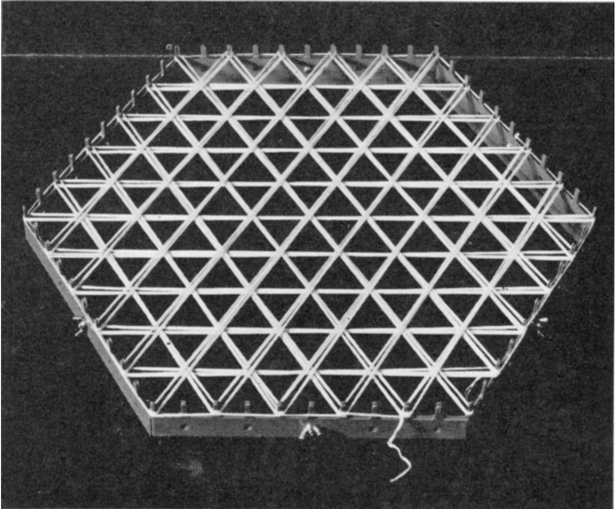
STEP ONE —in winding frame for twelve-petal daisy design.
