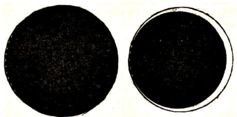
In a total Eclipse
