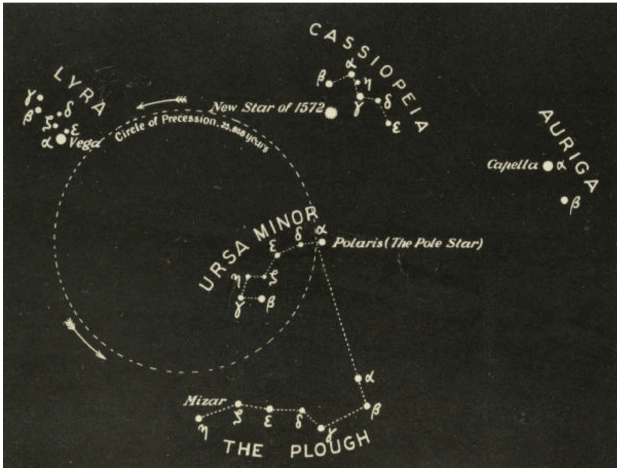
PLATE XIX. THE SKY AROUND THE NORTH POLE
