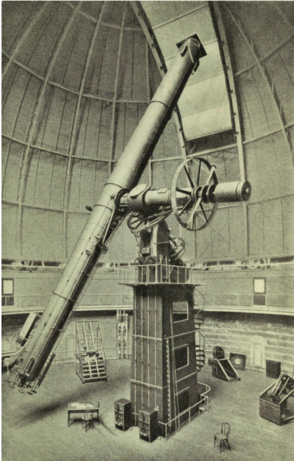
PLATE IV. THE GREAT YERKES TELESCOPE
