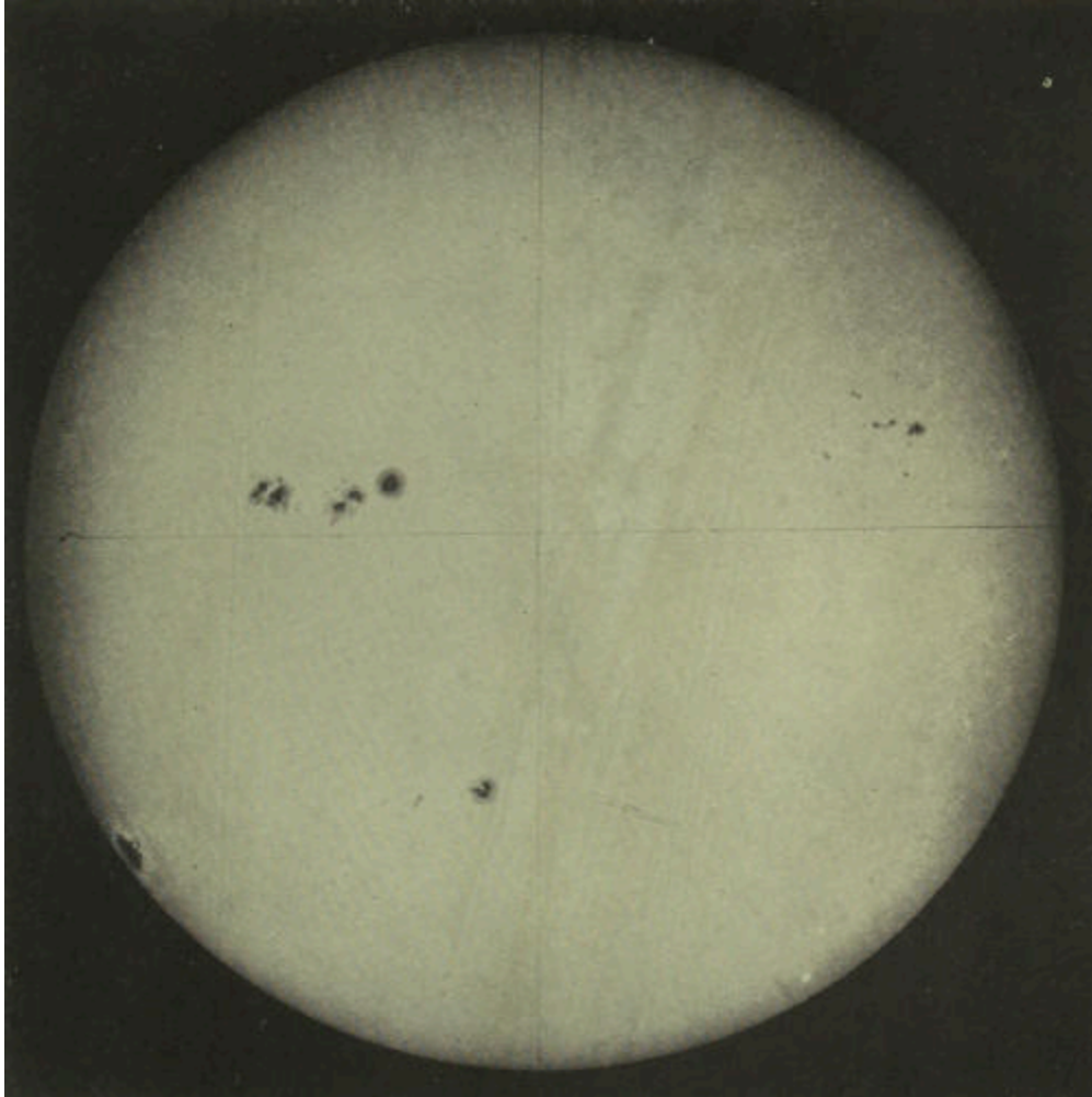
PLATE V. THE SUN, SHOWING SEVERAL GROUPS OF SPOTS
