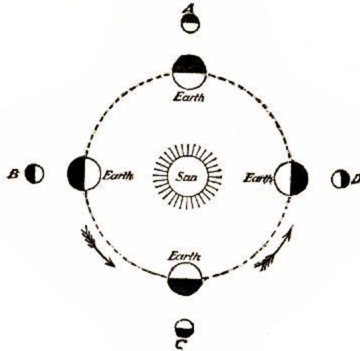
Various positions of Laplace's "Moon" with regard to the earth and sun during the course of a year.
