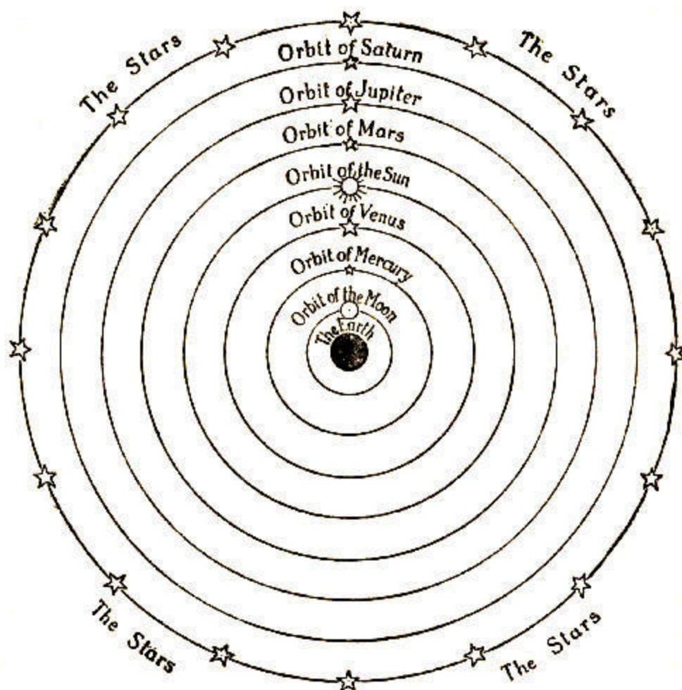
FIG. 1.—The Ptolemaic idea of the Universe.
