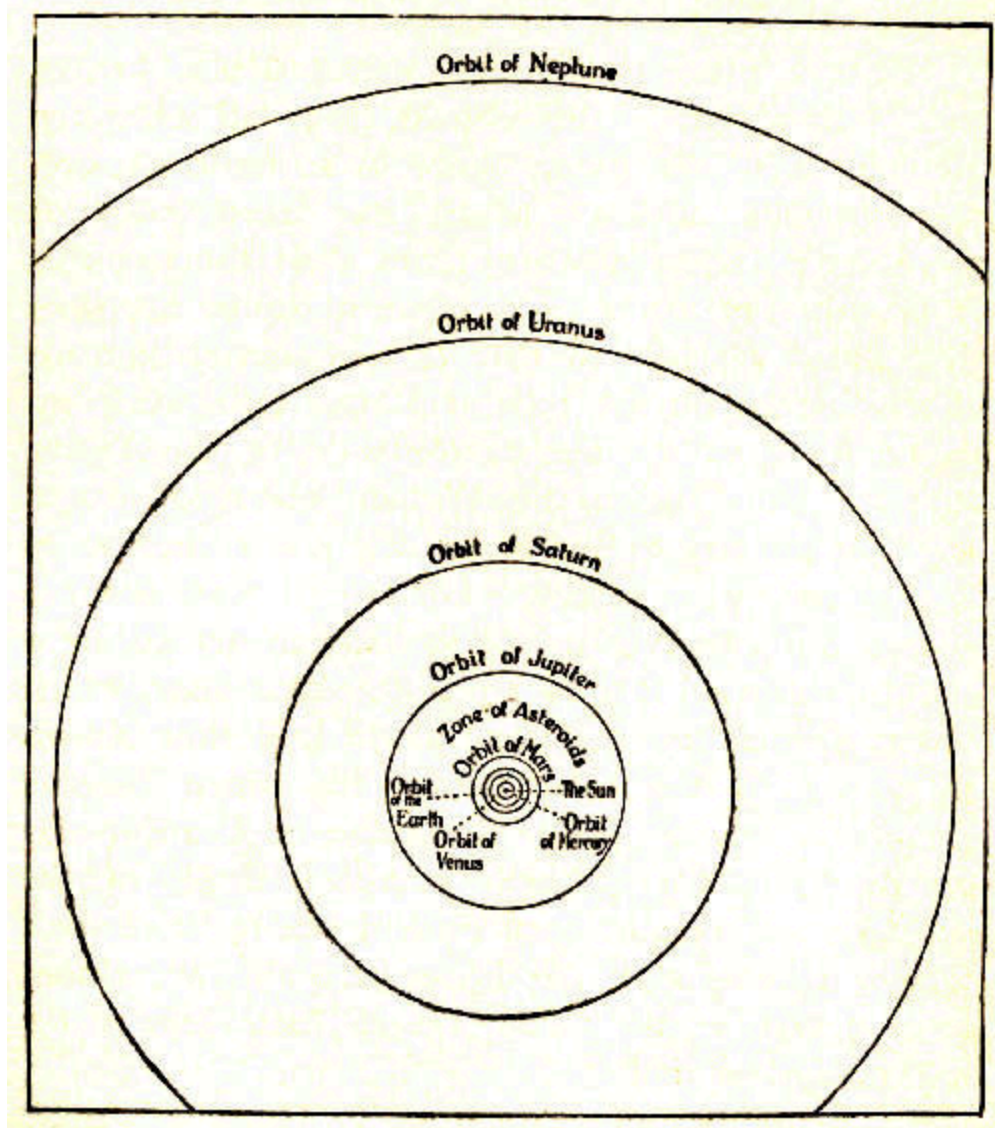
FIG. 2.—The Copernican theory of the Solar System.
