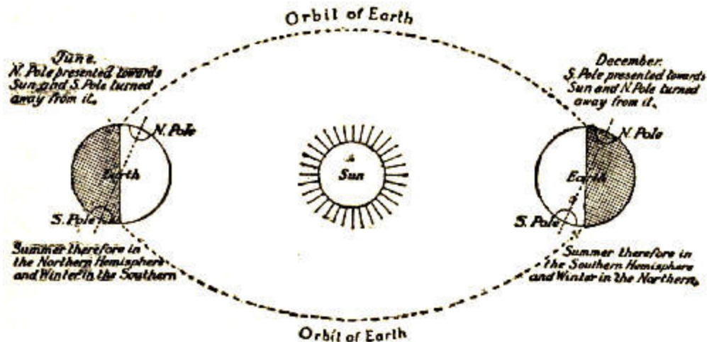
FIG. 13.—Summer and Winter.
