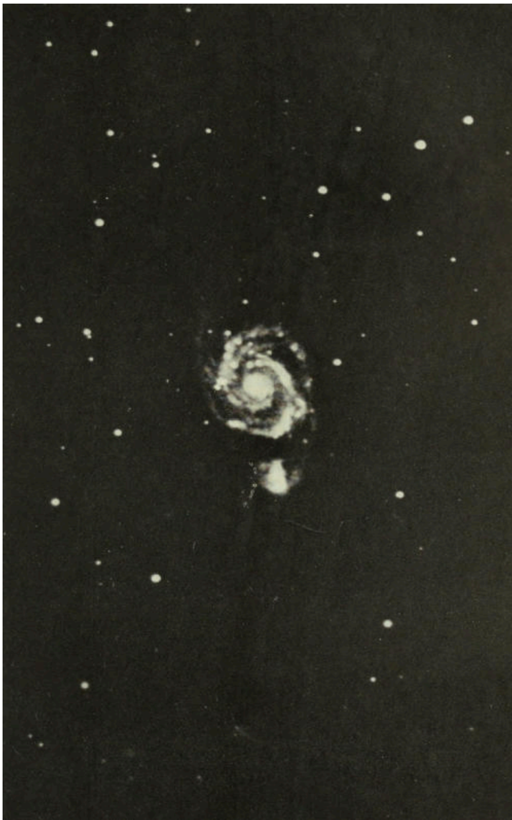
PLATE XXII. SPIRAL NEBULA IN THE CONSTELLATION OF CANES VENATICI From a photograph by the late Dr. W.E. Wilson, D.Sc., F.R.S.
