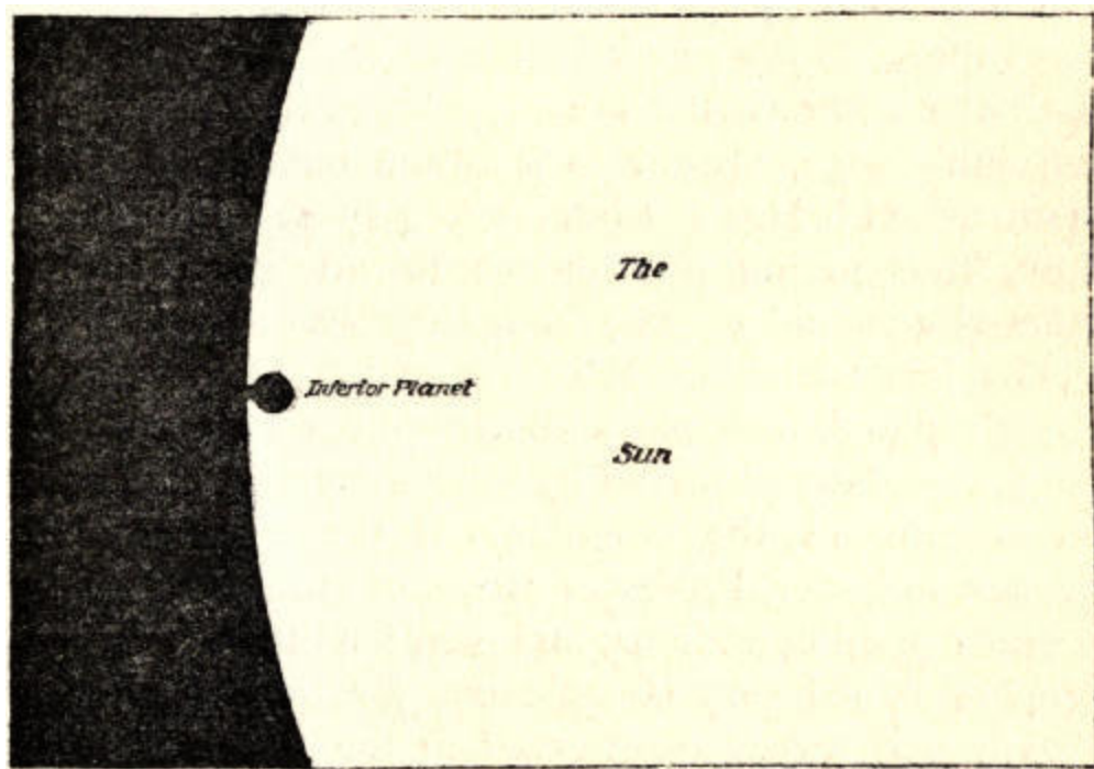
FIG. 12.—The "Black Drop."
