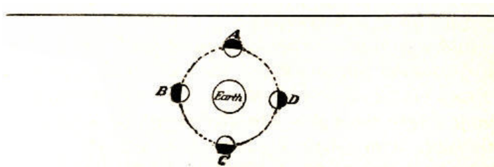
The same positions of Laplace's "Moon," arranged around the earth, show that it would make only one revolution in a year.
