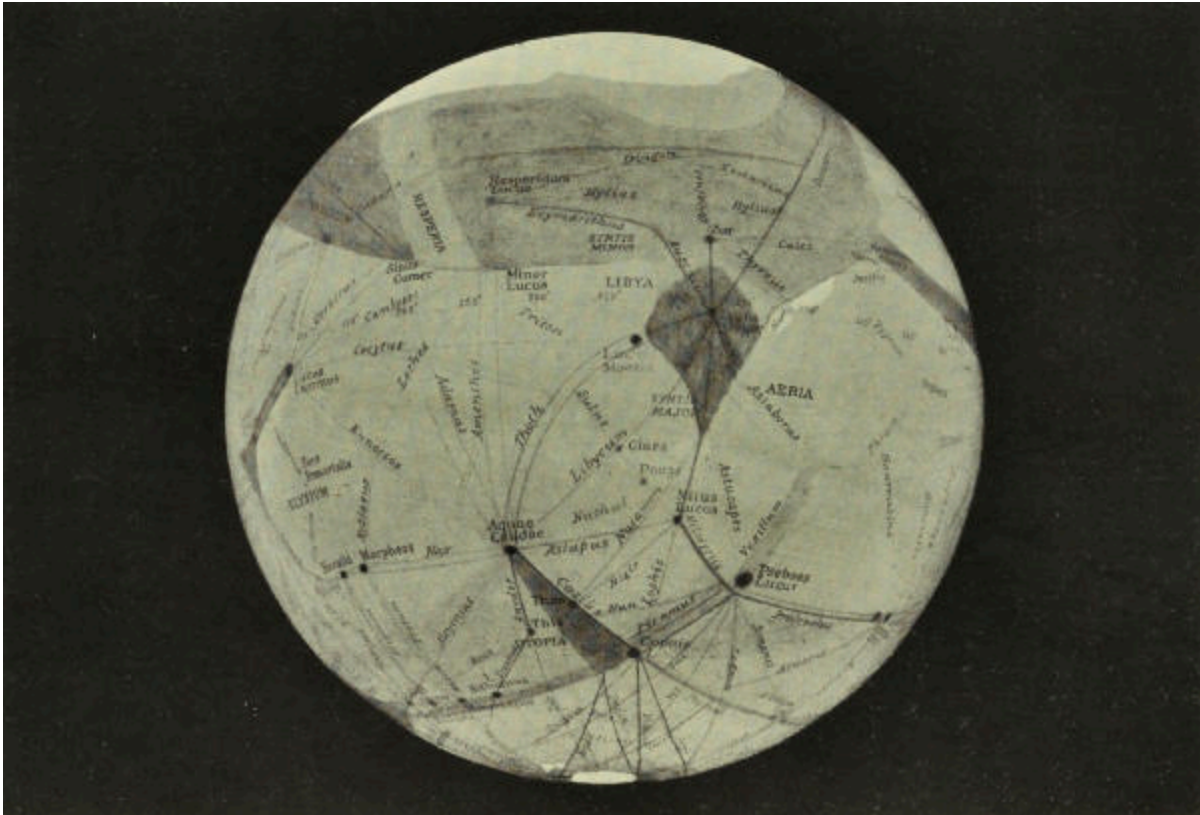
PLATE XII. A MAP OF THE PLANET MARS
