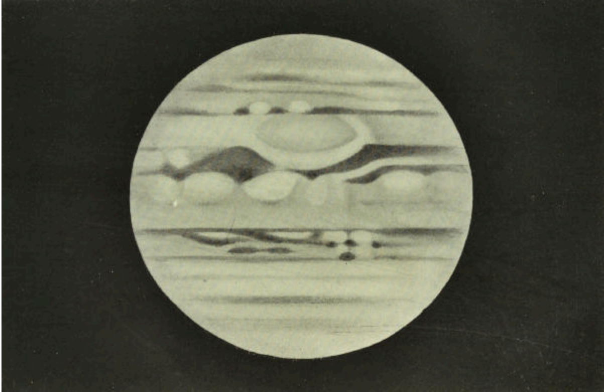
PLATE XIV. THE PLANET JUPITER
