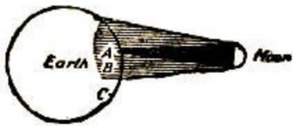
(i.) Total Eclipse of the Sun.
