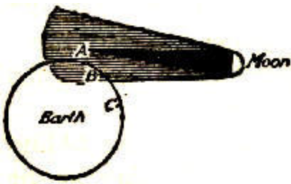
(ii.) Partial Eclipse of the Sun.
