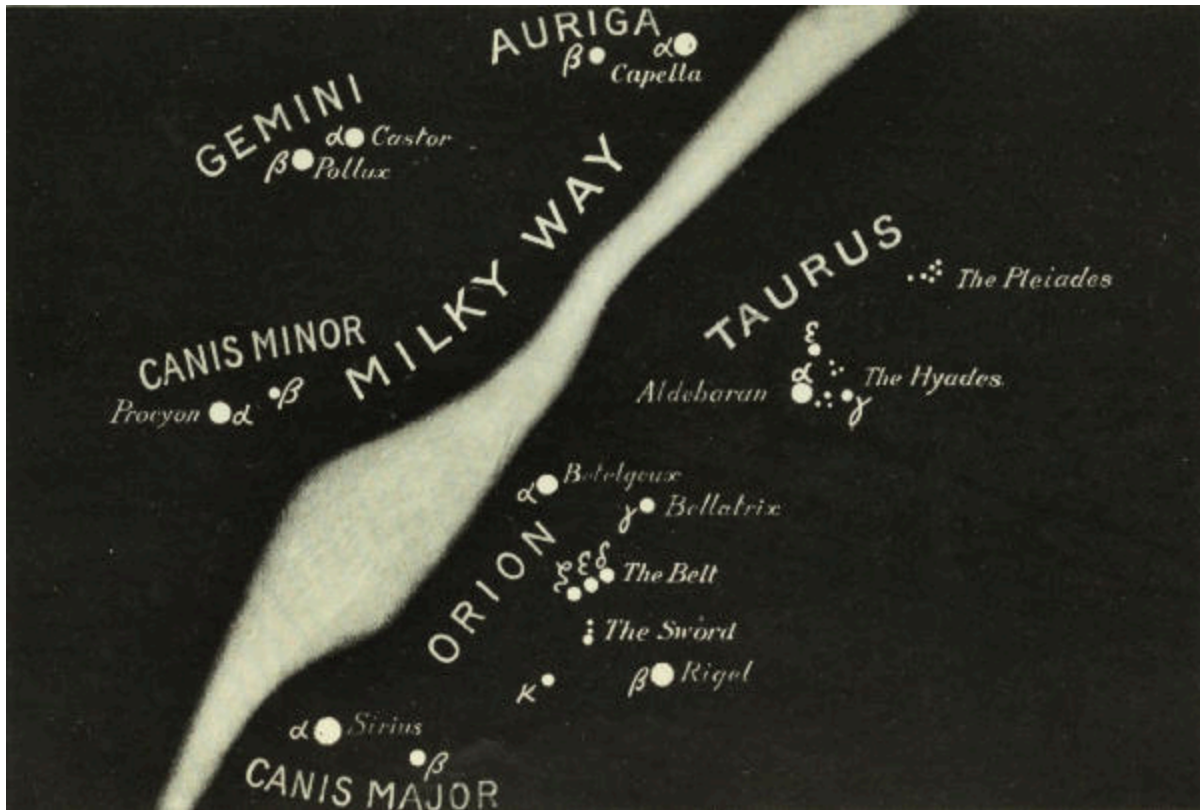
PLATE XX. ORION AND HIS NEIGHBOURS
