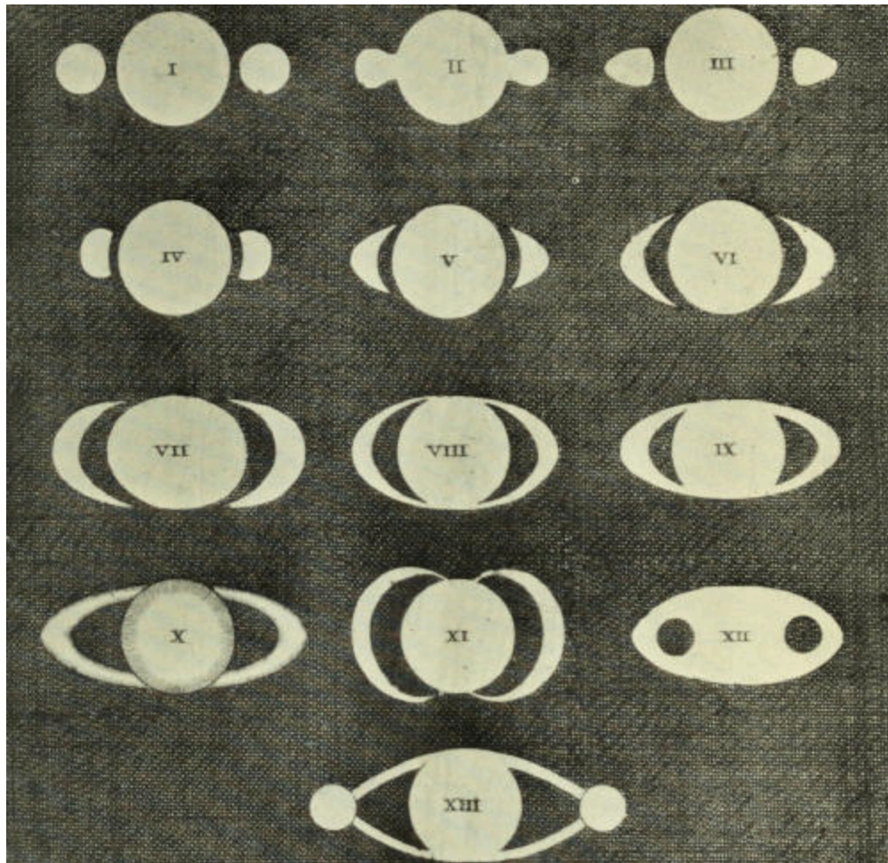
PLATE XVI. EARLY REPRESENTATIONS OF SATURN From an illustration in the Systema Saturnium of Christian Huyghens. ( Page 242 )
