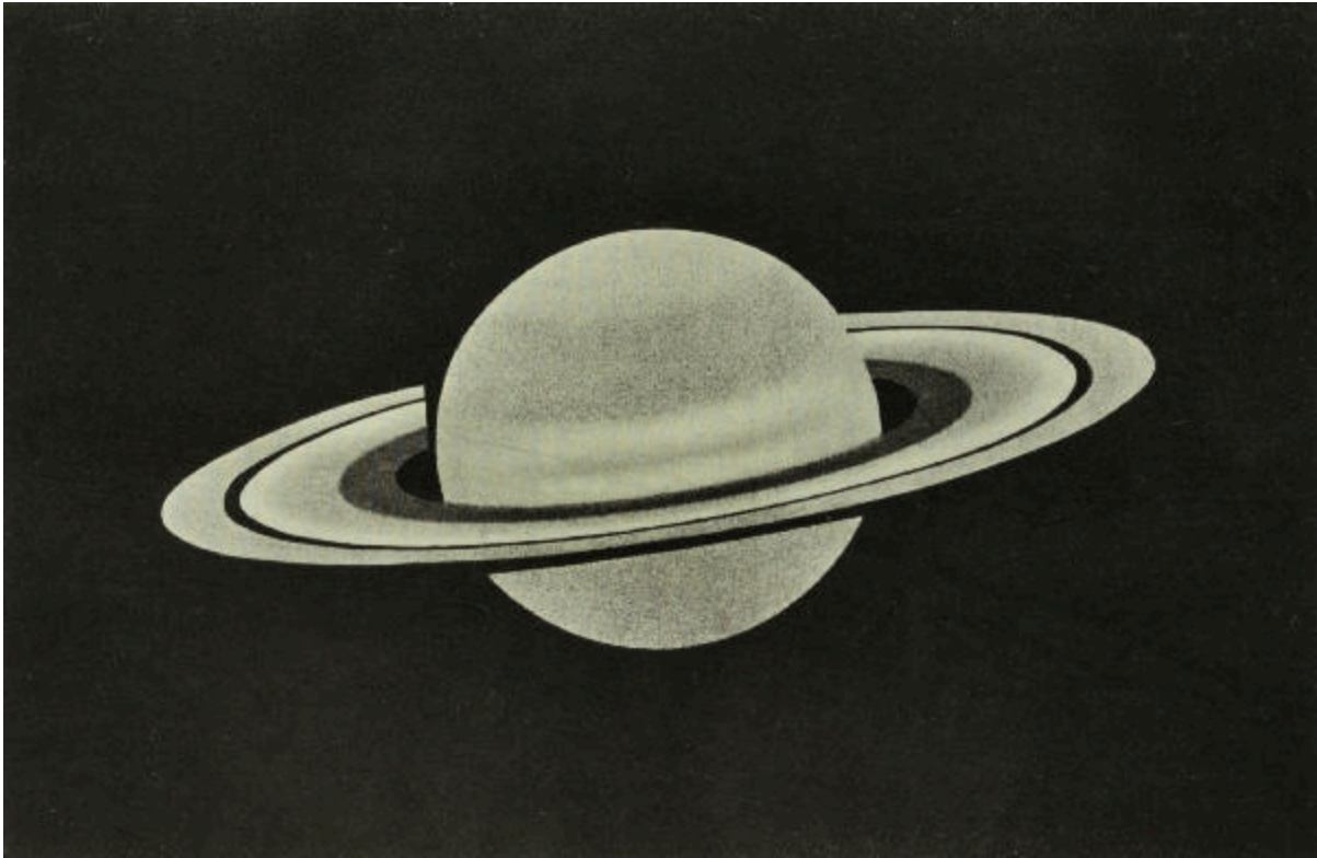
PLATE XV. THE PLANET SATURN
