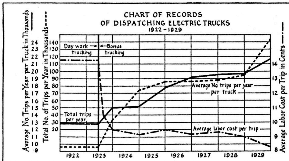
CHART OF RECORDS OF DISPATCHING ELECTRIC TRUCKS 1922-1929
