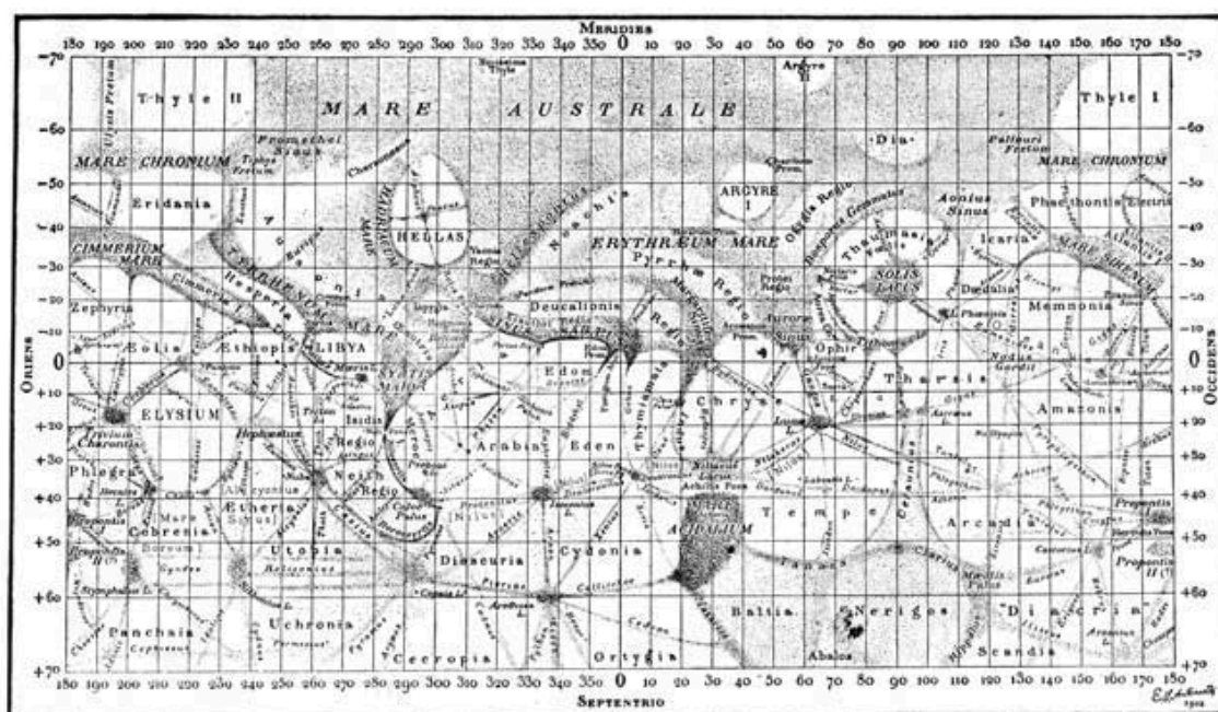
Memoirs of the British Astronomical Association. MAP OF MARS.
