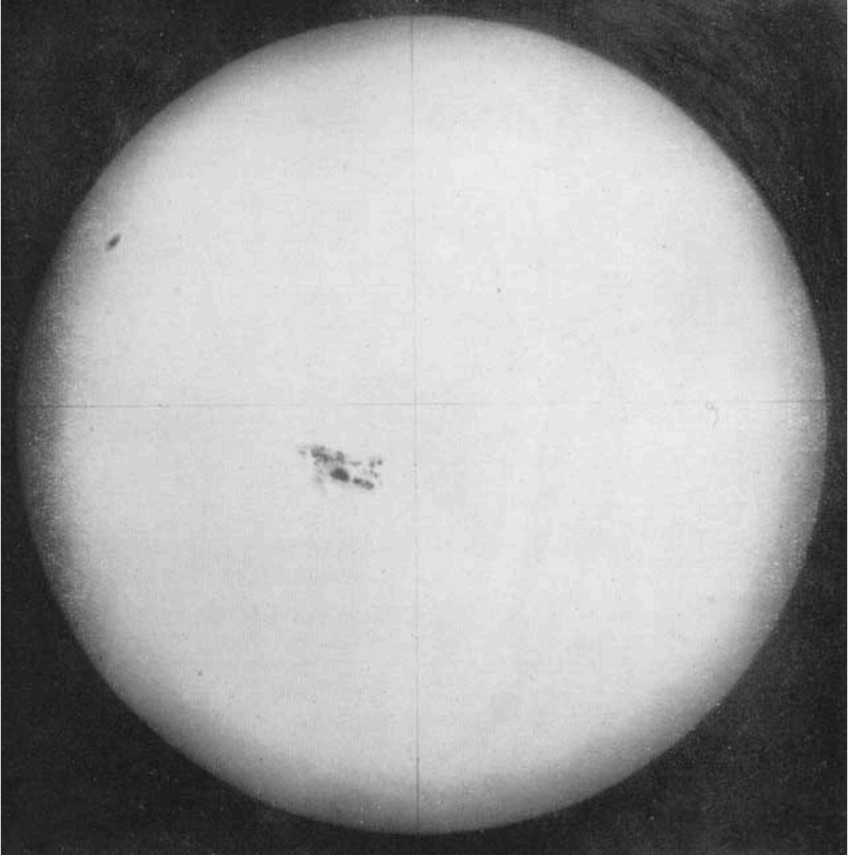
Royal Observatory, Greenwich. SUN-SPOTS.
