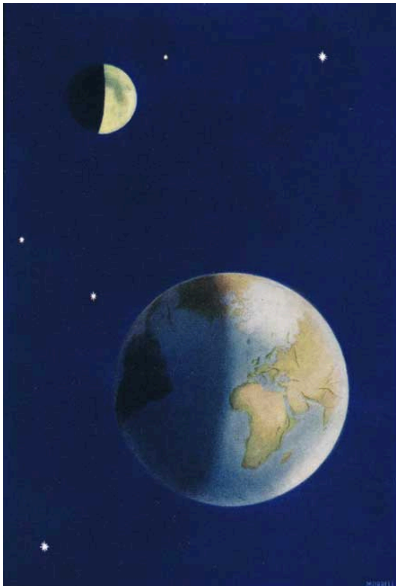
THE EARTH AND MOON HANGING IN SPACE
