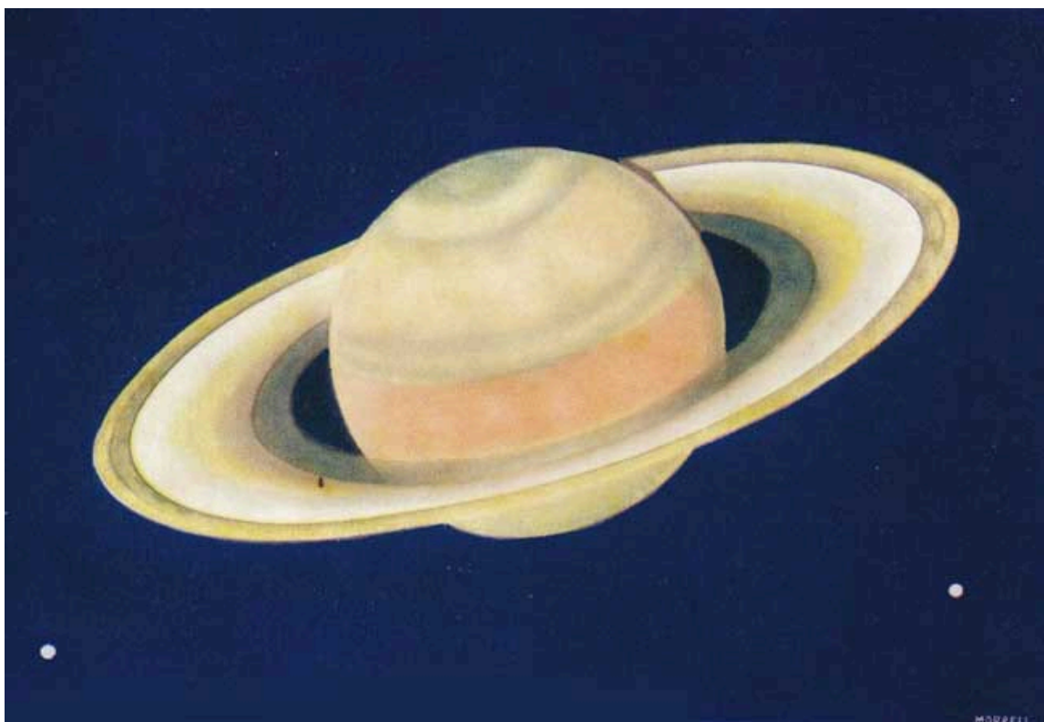
THE PLANET SATURN WITH TWO OF HIS MOONS.
