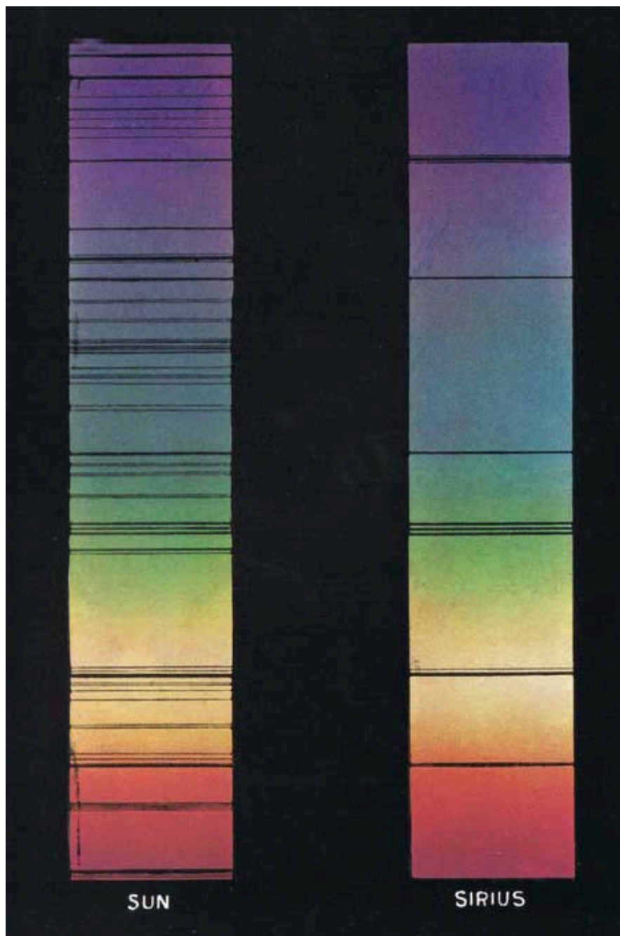
THE SPECTRUM OF THE SUN AND SIRIUS.
