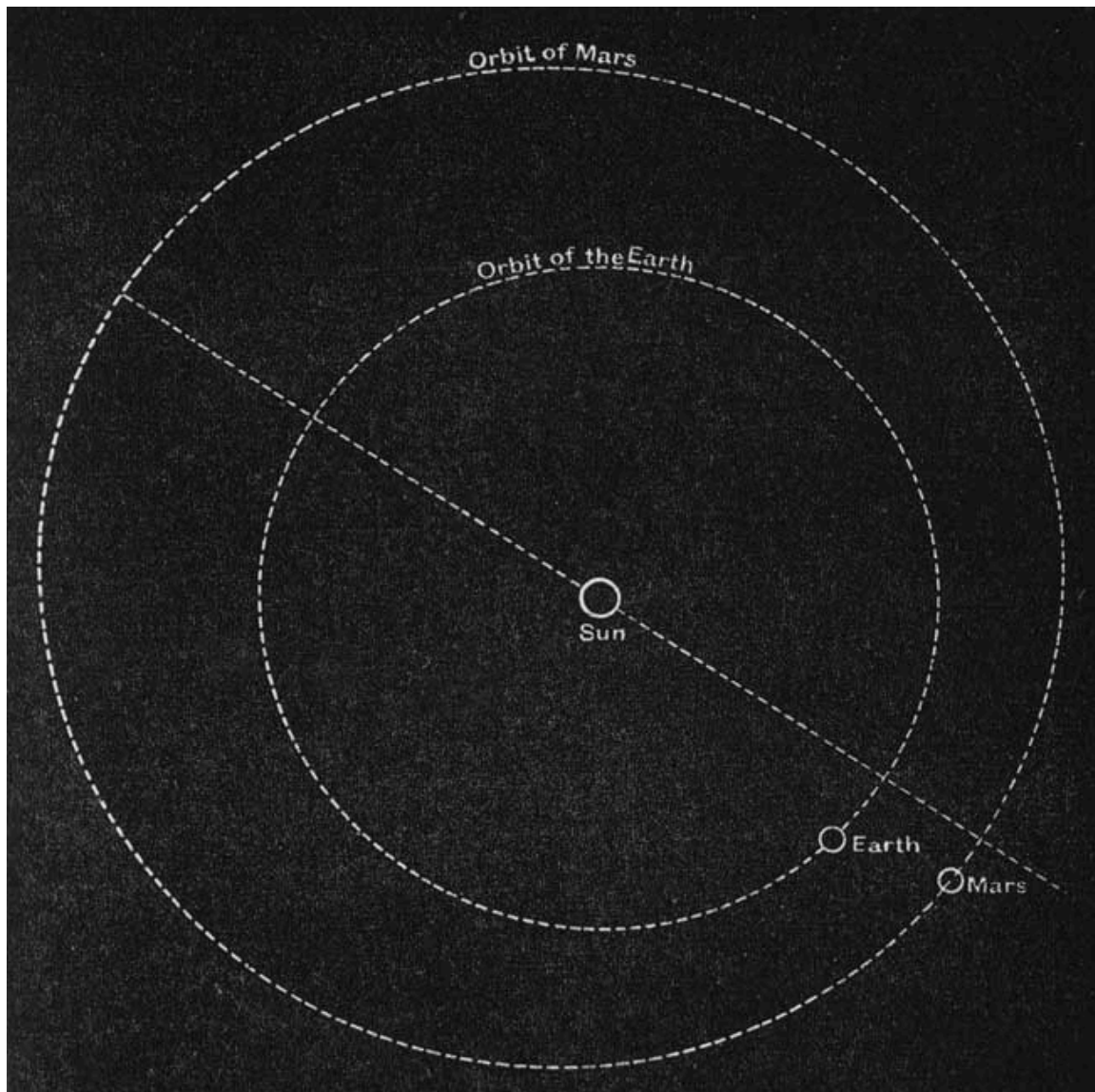
ORBITS OF THE EARTH AND MARS.
