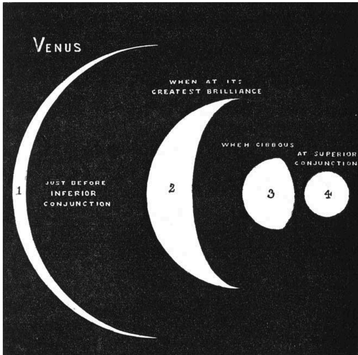
DIFFERENT PHASES OF VENUS.
