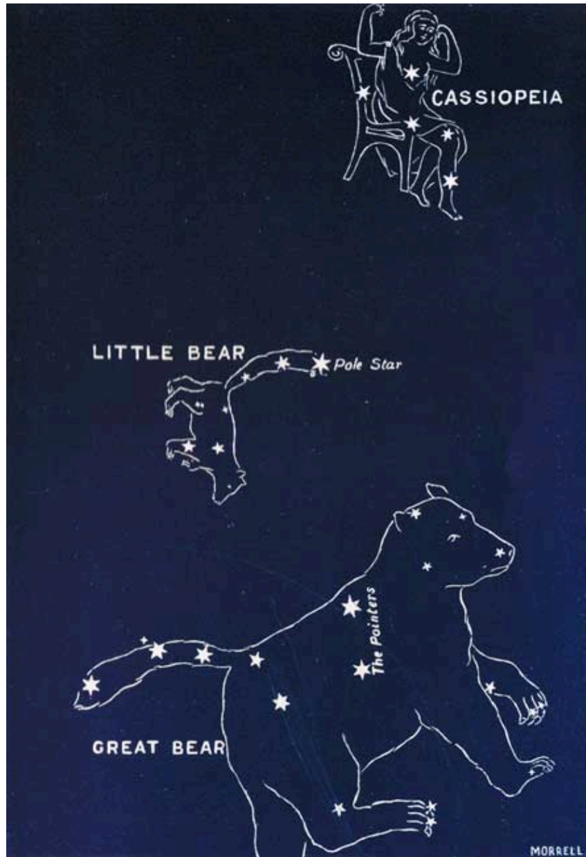
CONSTELLATIONS NEAR THE POLE STAR.
