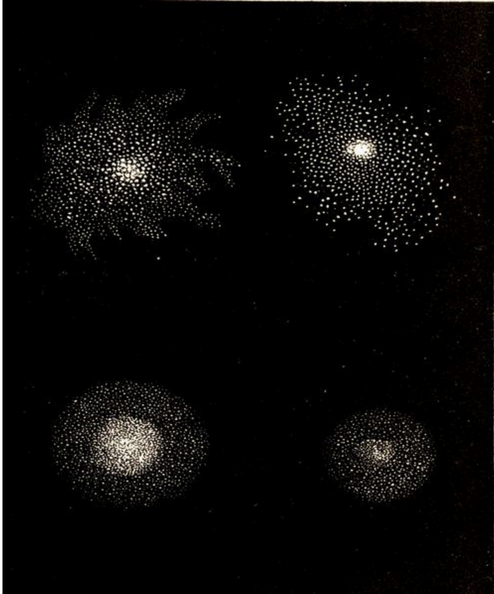
Figures 70, 71, 72, 73. CLUSTERS OF STARS AND NEBULÆ.
