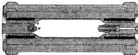
FIG. 7. Explosion Vessel.
