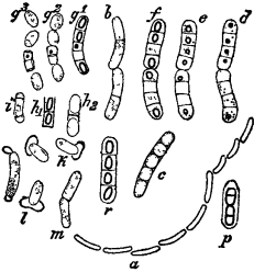
FIG. 6.— Bacillus megaterium . (After de Bary.)
