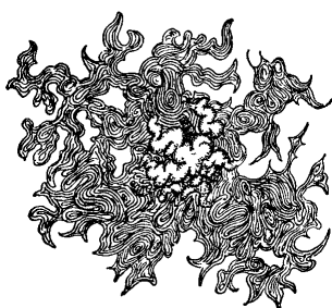
FIG. 21.—A plate-culture colony of a species of Bacillus-Proteus (Hauser)—on the fifth day. The flame-like processes and outliers are composed of writhing filaments, and the contours are continually changing while the colony moves as a whole. Slightly magnified. (H. M. W.)
