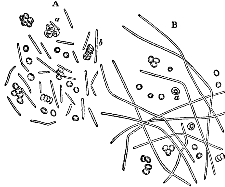
FIG. 7.— Bacillus anthracis . (After Koch.)
