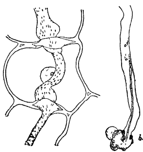
FIG. 15.—Invasion of leguminous roots by bacteria.
