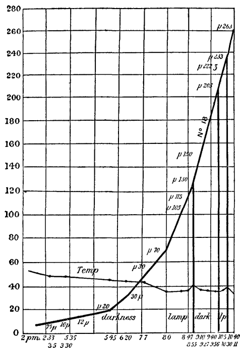
FIG. 8.—Curve of growth of a filament of Bacillus ramosus (Fraenkel), constructed from data such as in fig. 4. The abscissae represent intervals of
