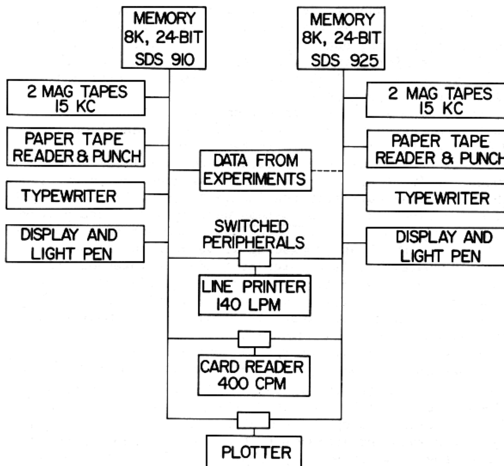
FIGURE 8 The two-central-processor system of Rutgers-Bell.
