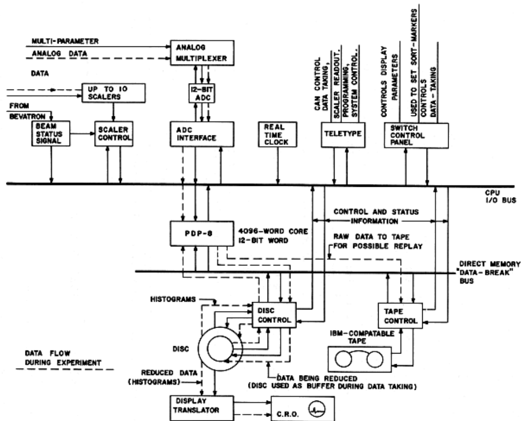
FIGURE 4 PDP-8 data-acquisition system at Lawrence Radiation Laboratory.
