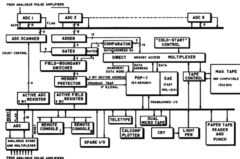
FIGURE 2 PDP-7 data-acquisition system at Lawrence Radiation Laboratory
