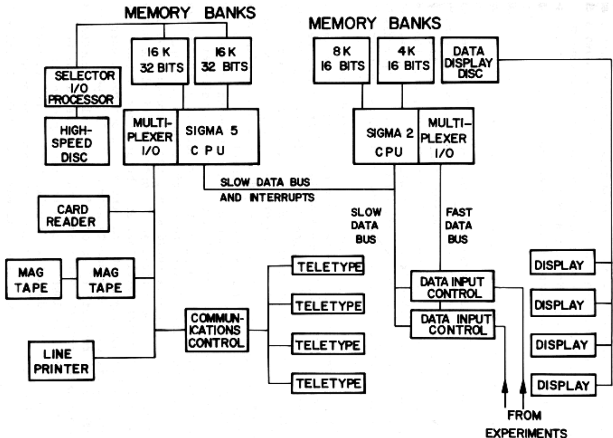
FIGURE 9 The new Rutgers-Bell Sigma 2-Sigma 5 system.
