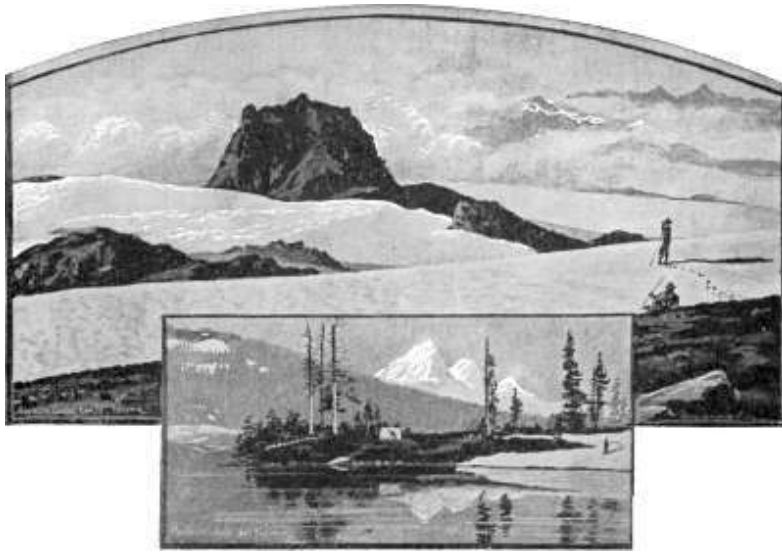
GLACIERS ON MOUNT TACOMA.
