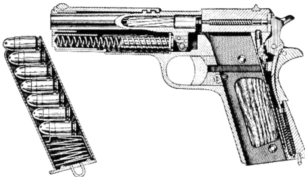
PLATE 14. UNITED STATES ARMY REGULATION .45 COLT AUTOMATIC PISTOL. SECTIONAL VIEW
