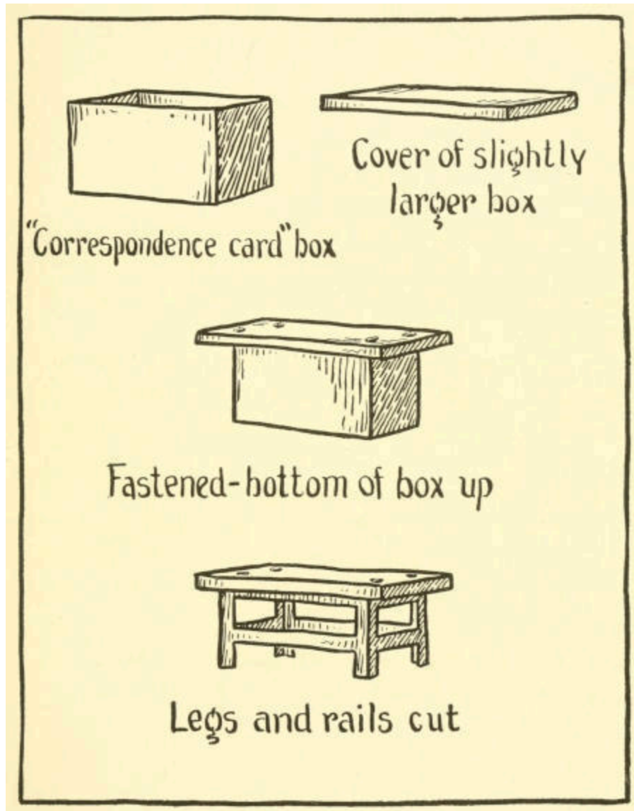
Details of Dining Table.
