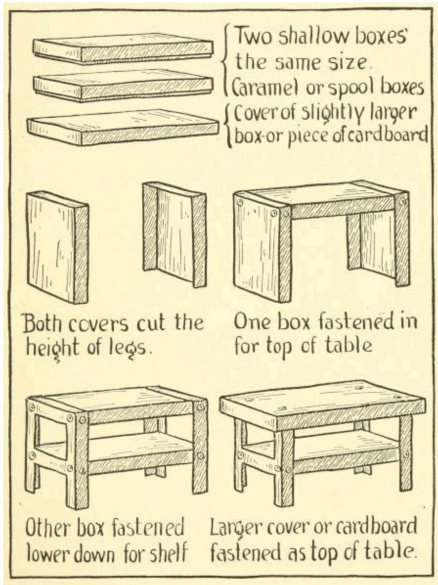
Details of Library Table.
