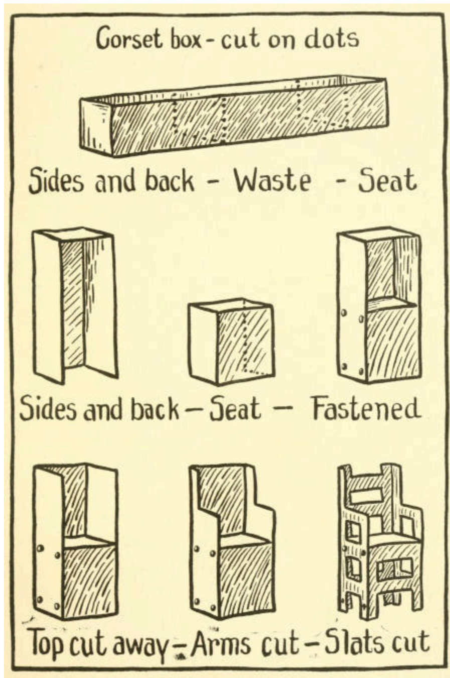
Details of Arm Chair.
