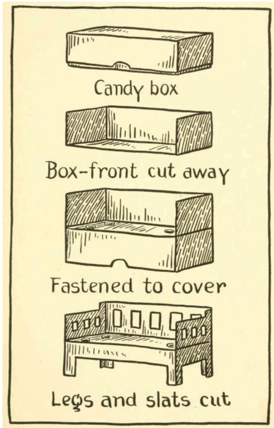
Details of Divan.
