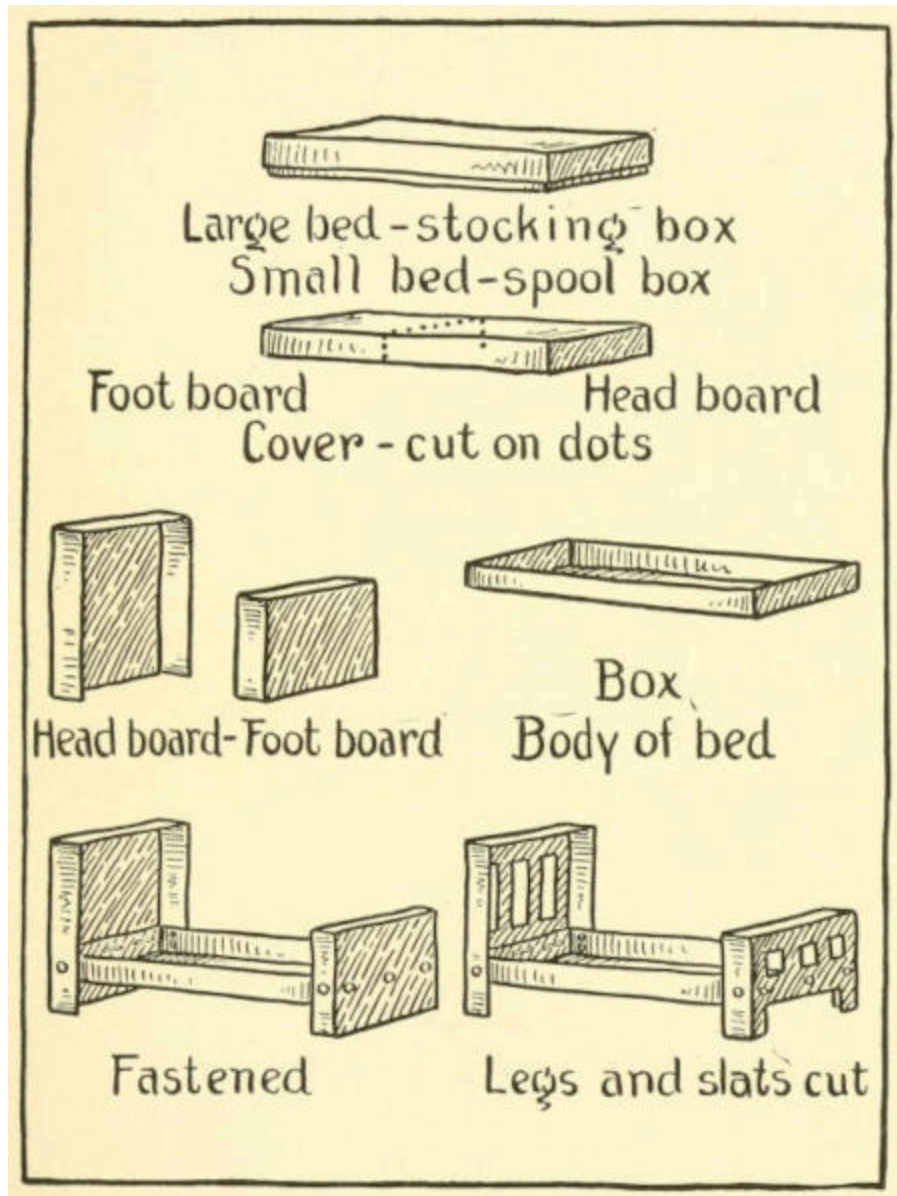
Details of Bed.
