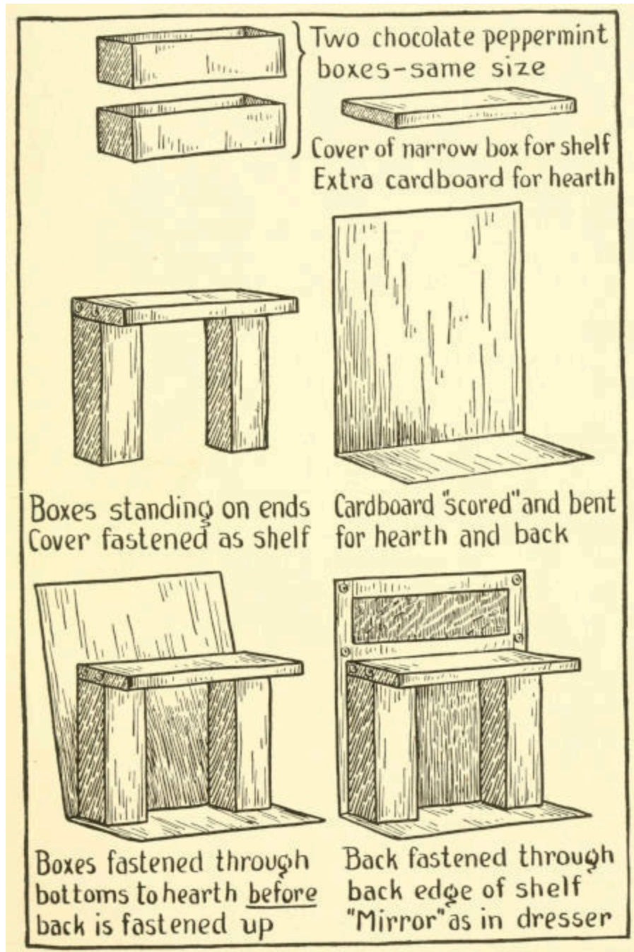
Details of Fireplace.
