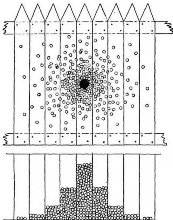
ORIGIN OF A NORMAL PROBABILITY CURVE
