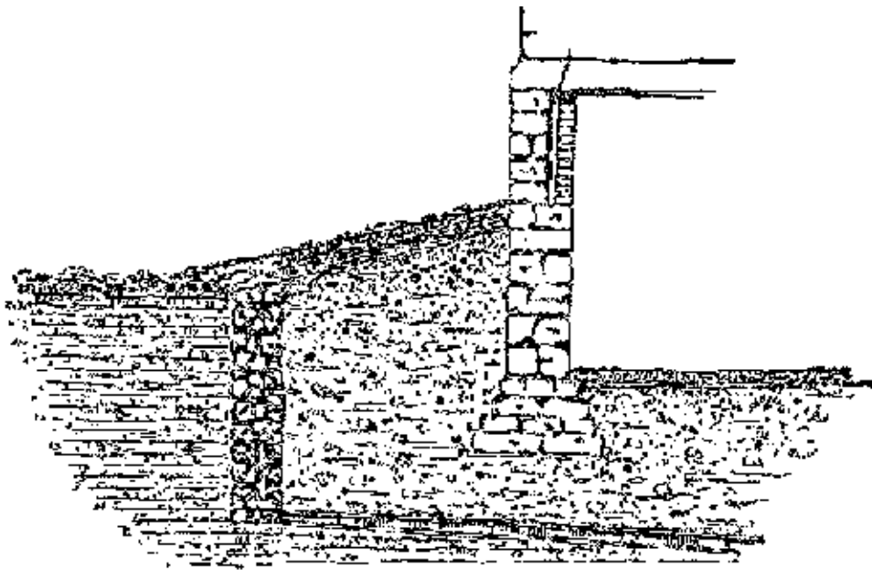
THE PROTECTING "CUT-OFF". To List
