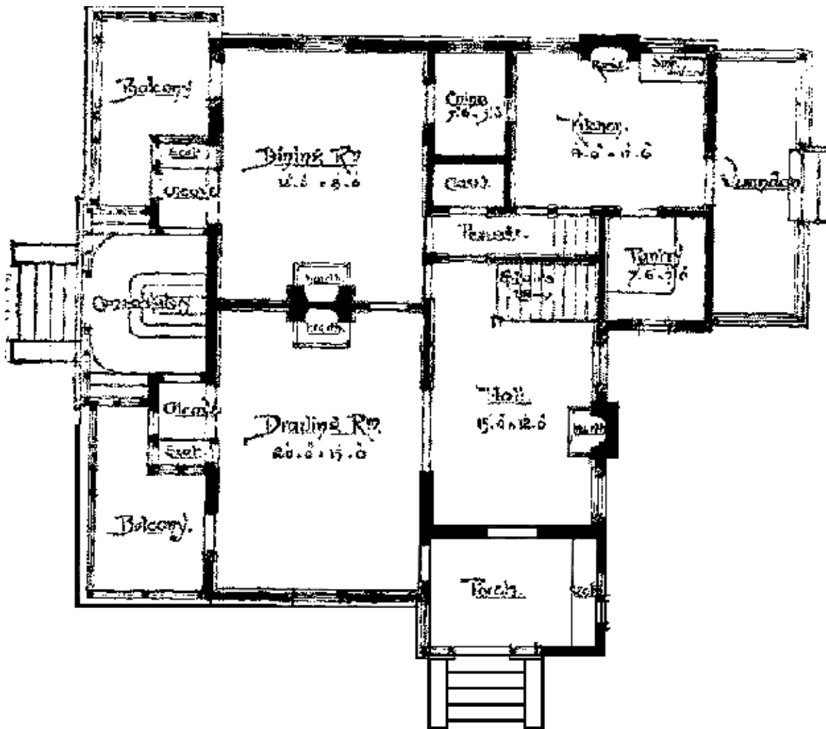
THE ATTORNEY'S FLOOR PLAN. To List
