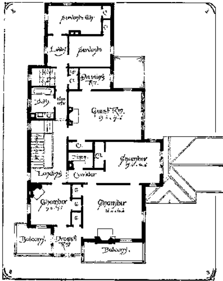
THE SECOND FLOOR OF THE HOUSE THAT JILL BUILT. ToList
