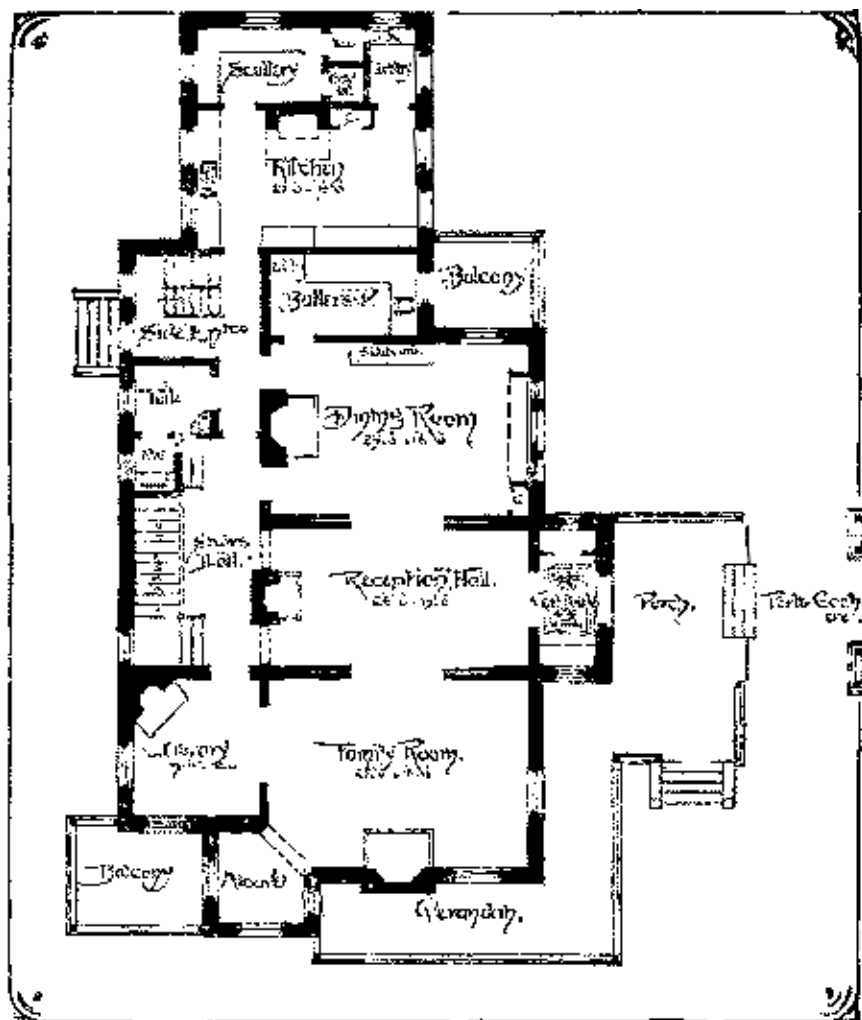
THE FIRST FLOOR OF THE HOUSE THAT JILL BUILT. To List
