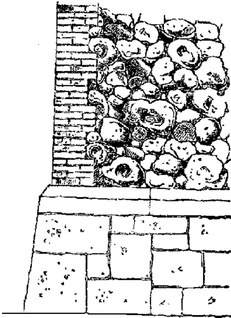
BRICKS AND BOULDERS ON GRANITE UNDERPINNING. To List
