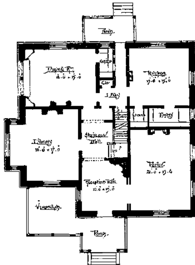
FIRST FLOOR OF THE PROMISE. To List
