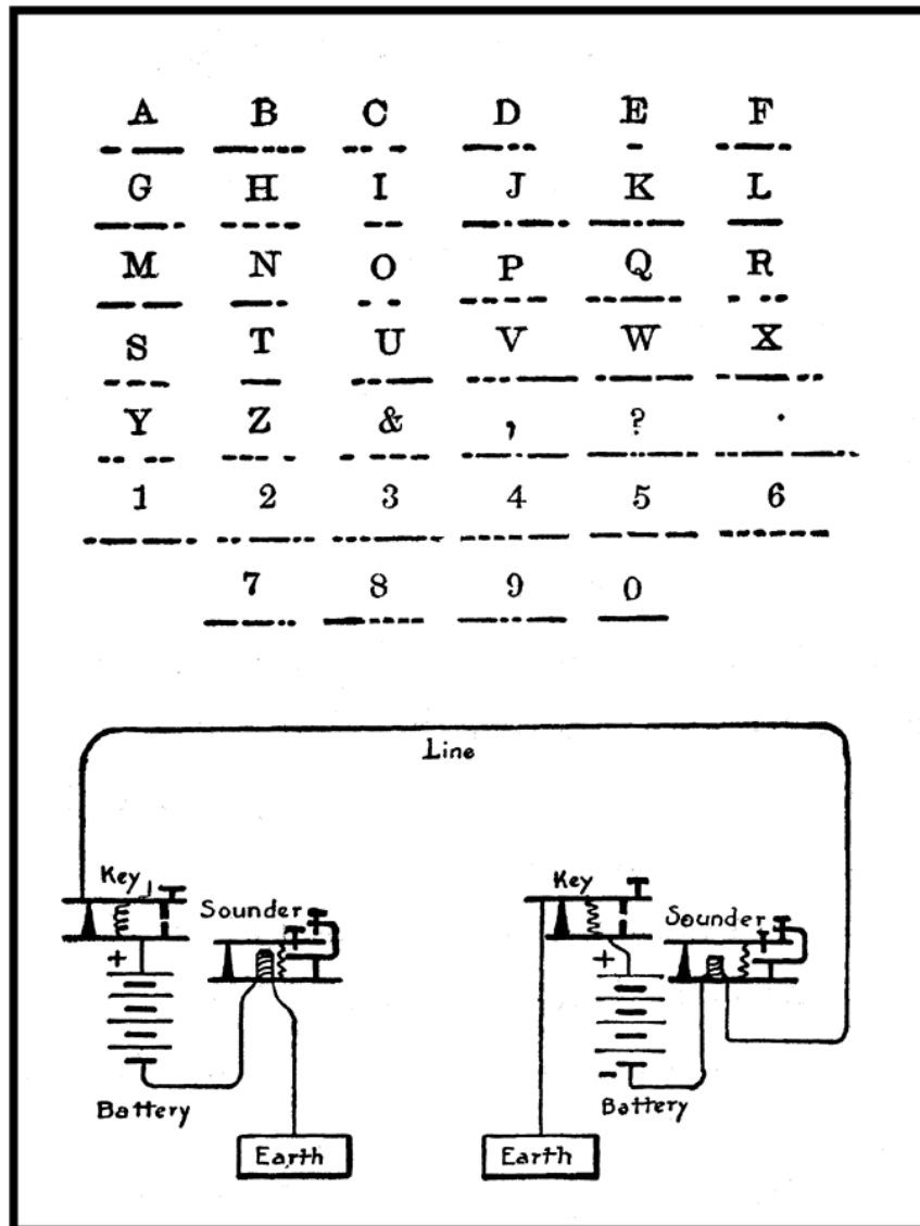
DIAGRAM SHOWING THE MORSE ALPHABET AND ARRANGEMENT OF THE TELEGRAPH LINE.
