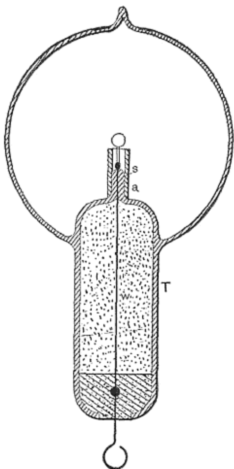
FIG. 21.—IMPROVED BULB WITH NON-CONDUCTING BUTTON.
