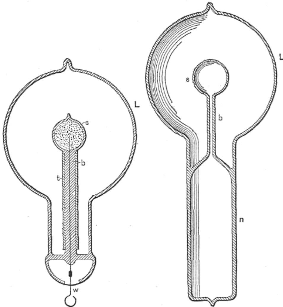
FIG. 12. FIG. 13. BULBS FOR PRODUCING ROTATING BRUSH.
