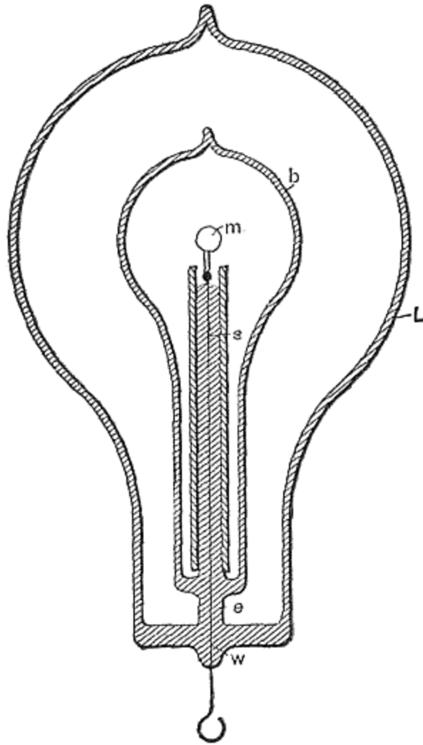
FIG. 29.—LAMP WITH INDEPENDENT AUXILIARY BULB.
