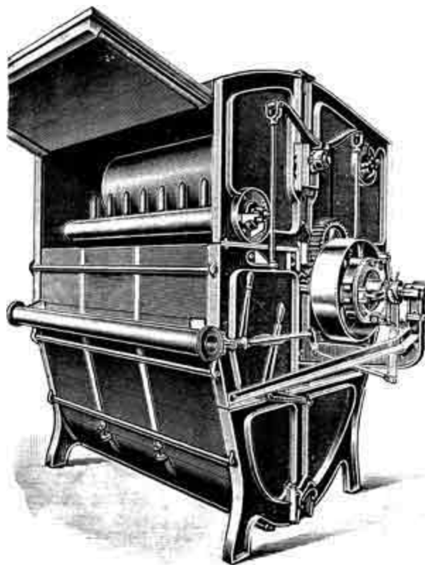
FIG. 34.—Cloth-washing Machine.
