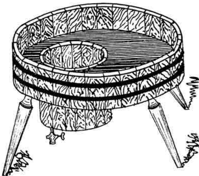
FIG. 27.—Dye-tub for Paranitroaniline Red.
