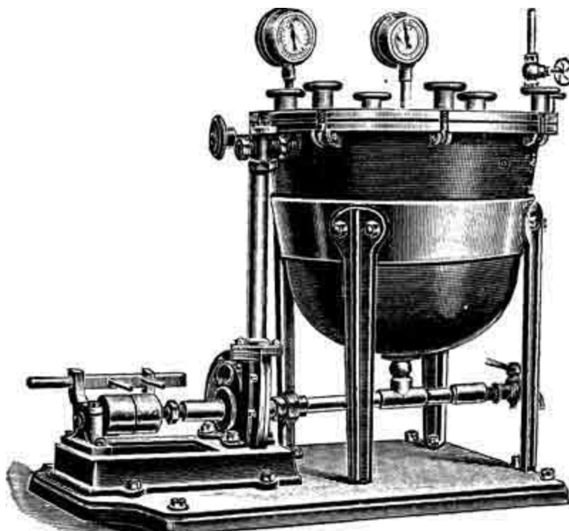
FIG. 15.—Beaumont's Cop-dyeing Machine.
