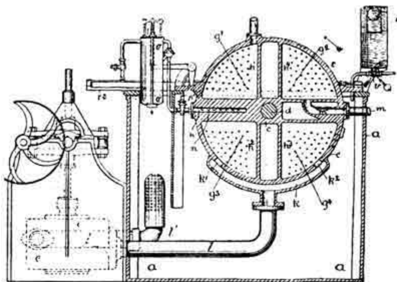
FIG. 14.—Graemiger Cop-dyeing Machine.
