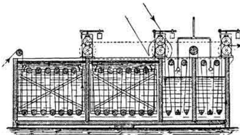
FIG. 36.—Washing and Soaping Vats.
