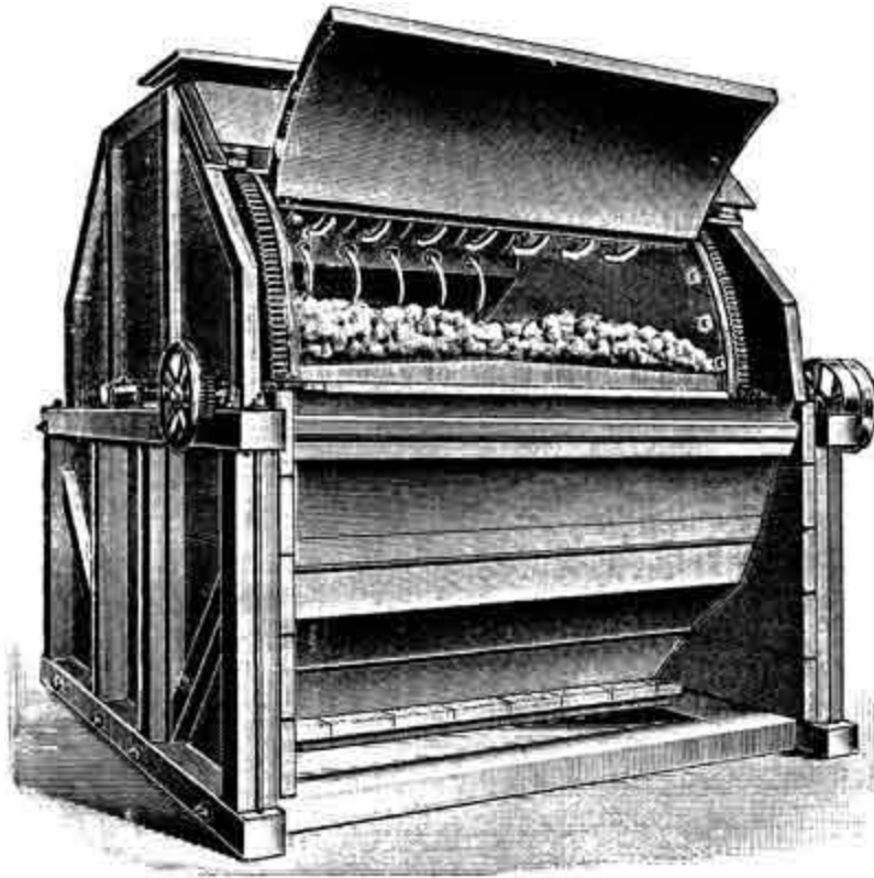
FIG. 9.—Delahunty's Dyeing Machine.
