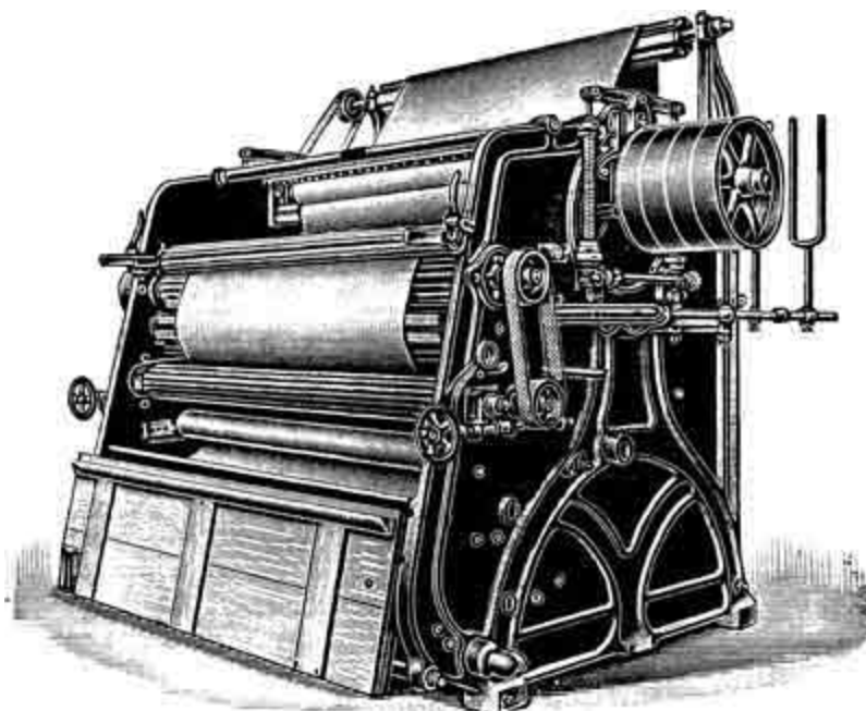
FIG. 35.—Cloth-washing Machine.
