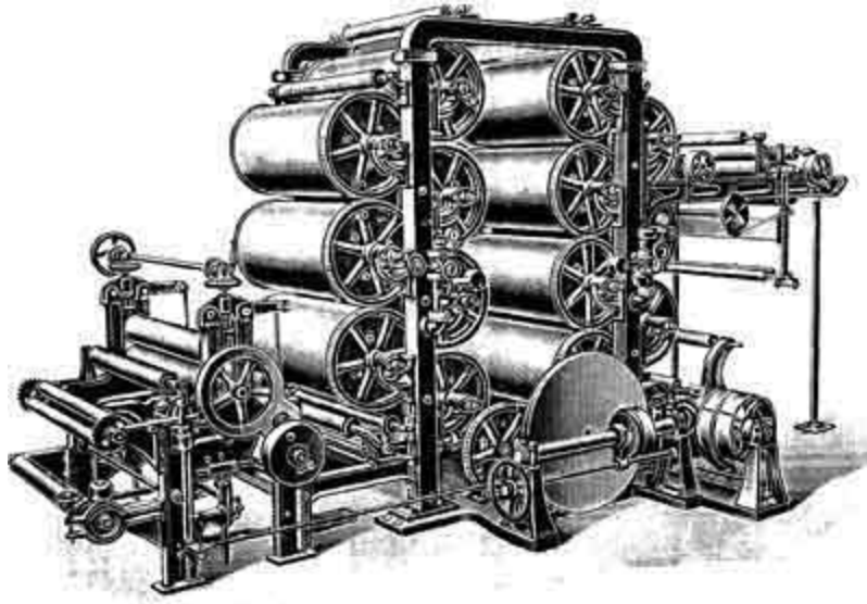
FIG 43.—Drying Cylinders.
