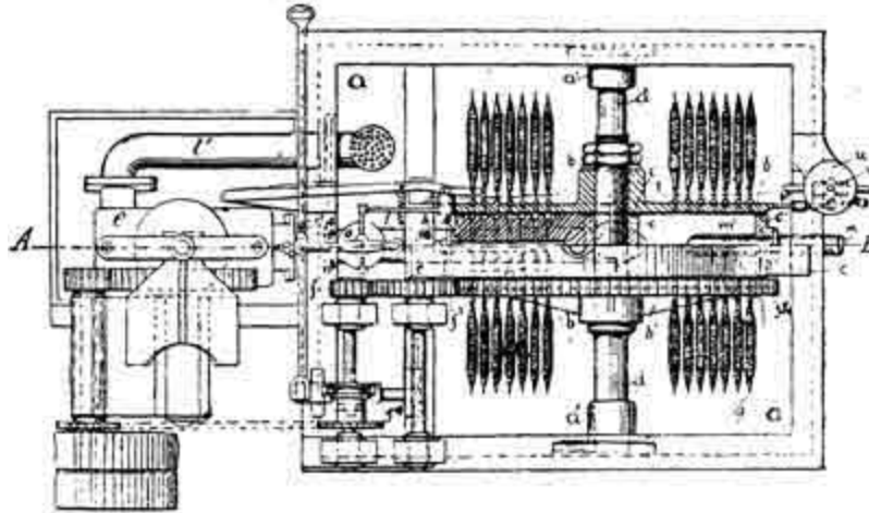
FIG. 13.—Graemiger Cop-dyeing Machine.
