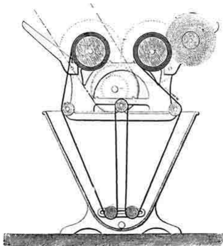
FIG. 19.—Dye-jigger.
