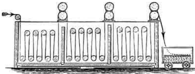
FIG. 16.—Warp-dyeing Machine.
