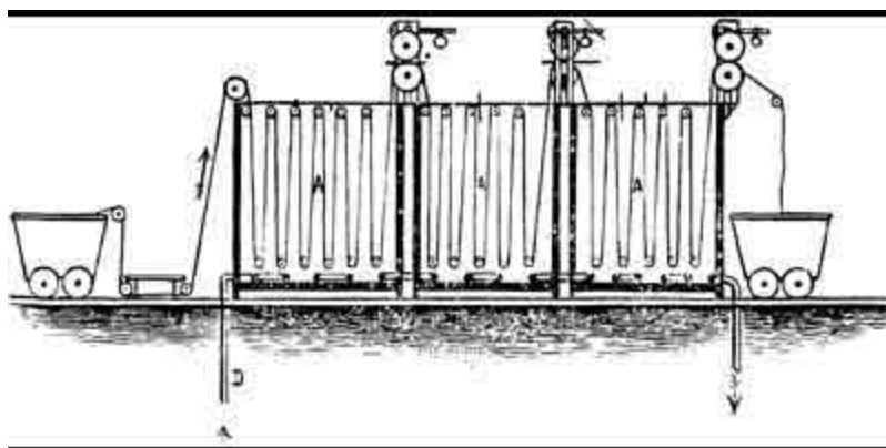
FIG. 24.—Continuous Dyeing Machine.
