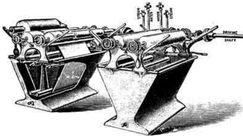
FIG. 18.—Dye-jiggers.
