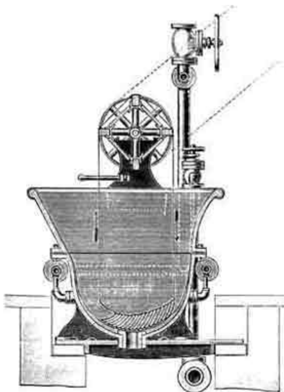
FIG. 22.—Dye Beck.
