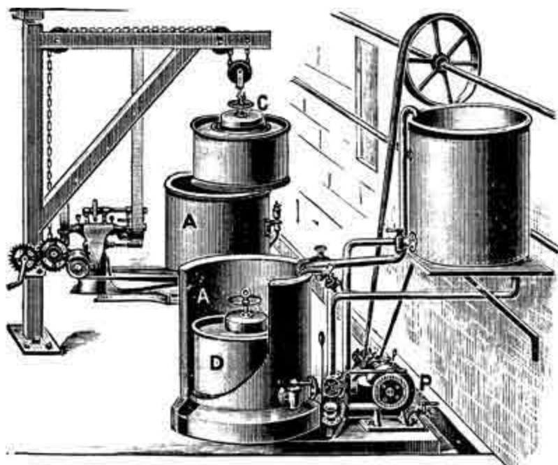
FIG. 10.—Obermaier Dyeing Machine.
