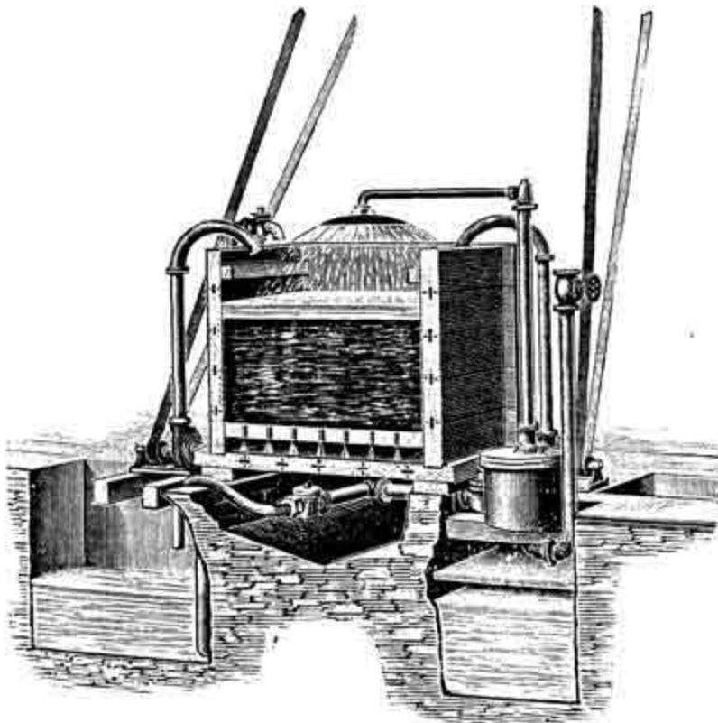
FIG. 5.—Mather & Platt's Yarn-bleaching Kier.
