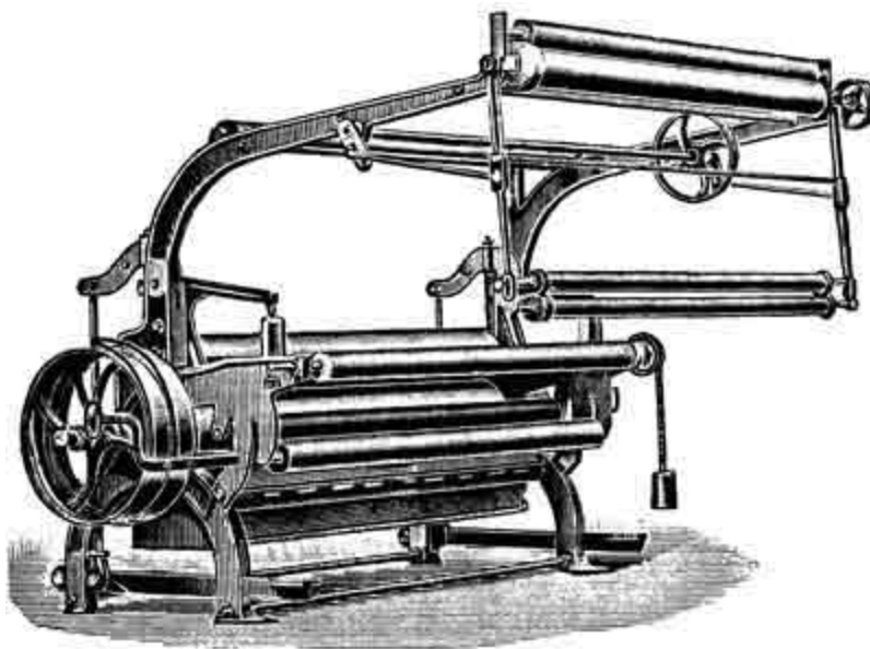
FIG. 28.—Padding Machine for Paranitroaniline Red.
