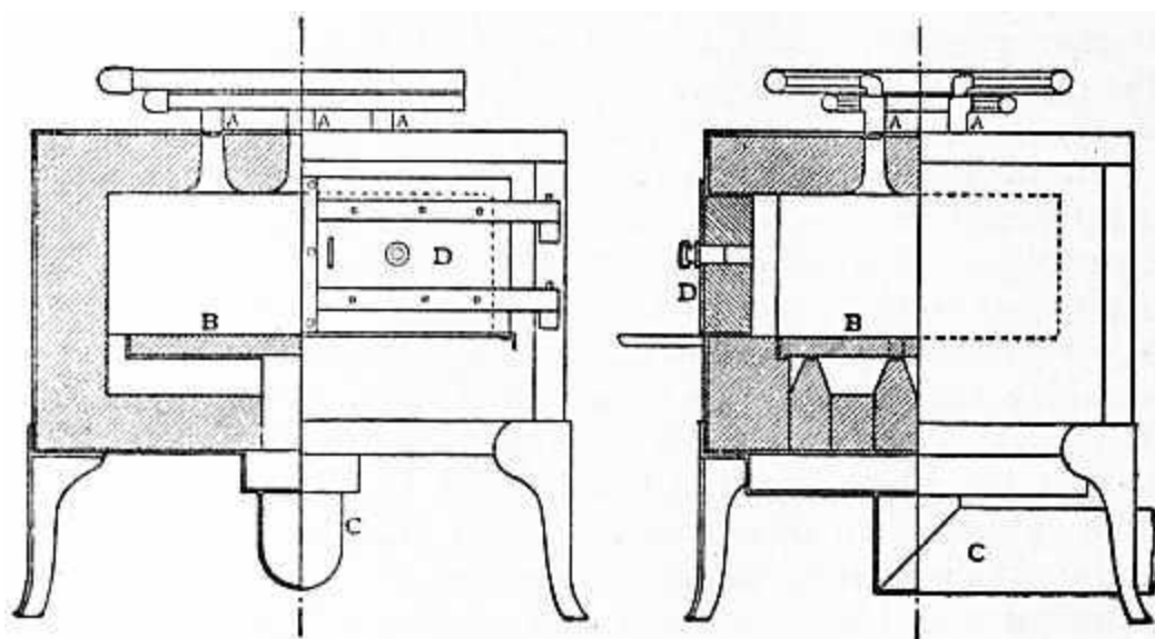
FIG. 2.—Reverberatory Furnace.
