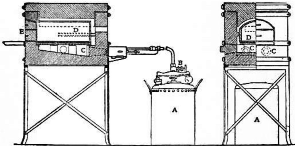
FIG. 1.—Automatic Oil Muffle Furnace.
