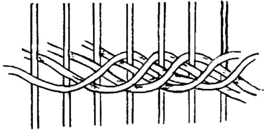
DIAGRAM NO. 8.—FOUR-ROD COIL
