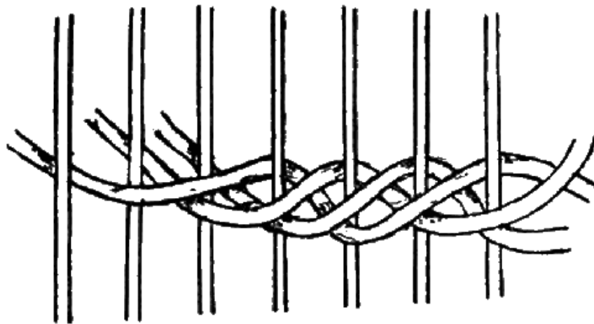
DIAGRAM NO. 7.—TRIPLE TWIST OR THREE-ROD COIL
