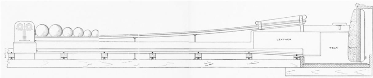
LONGITUDINAL SECTION OF A STANDARD BOWLING ALLEY
