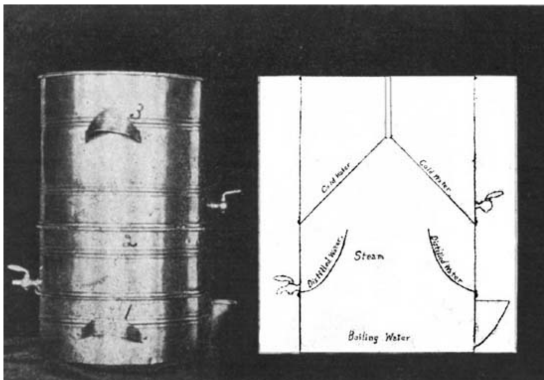
FIG. 63.—WATER STILL.
