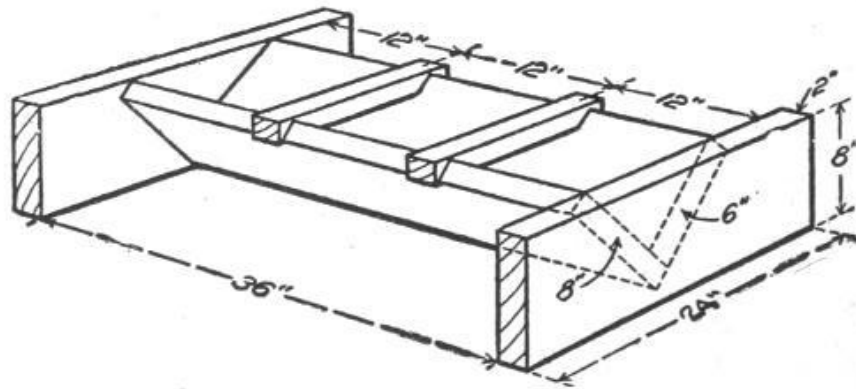
3. TROUGH FOR MATURE HOGS
