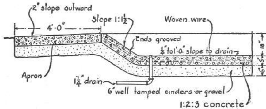
1. SECTIONAL VIEW OF A CONCRETE WALLOW
