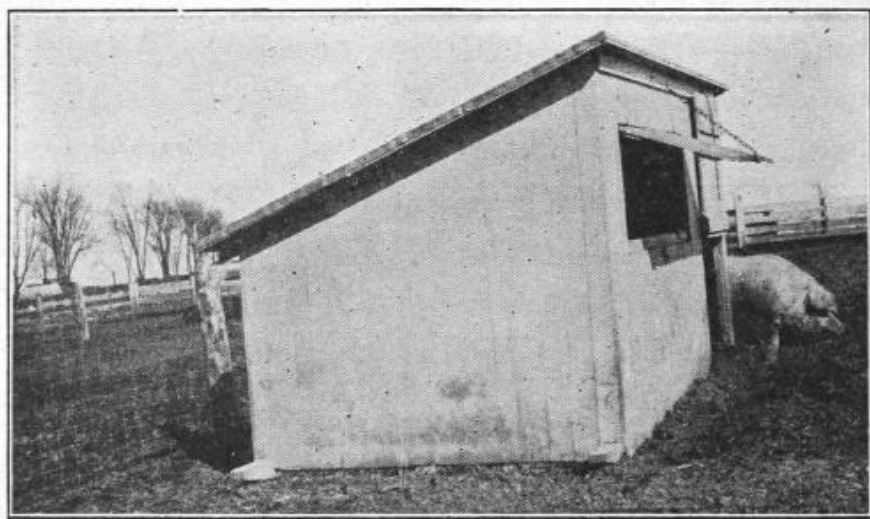
14. A GOOD HOG HOUSE
