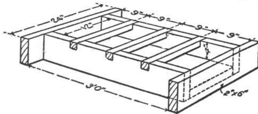
2. TROUGH FOR YOUNG PIGS
