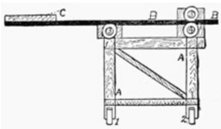
Fig. 68.—Side View of Apparatus
