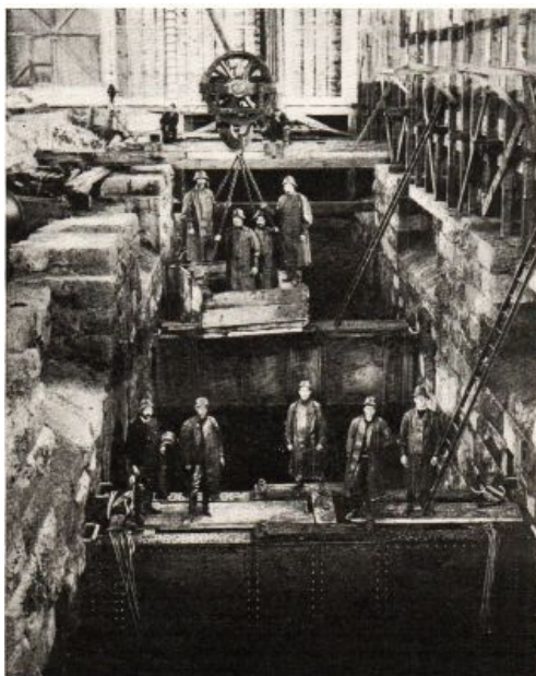
THE WHEEL-PIT IN COURSE OF CONSTRUCTION.
