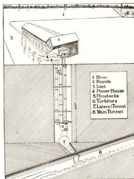
SECTIONAL DIAGRAM OF POWER-HOUSE.
