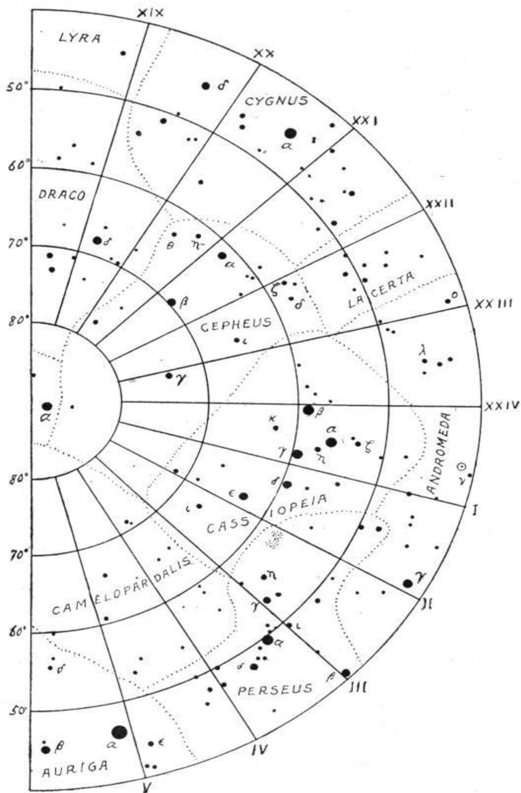
CHART X—POLAR CONSTELLATIONS FROM XVIII H. TO VI H.
