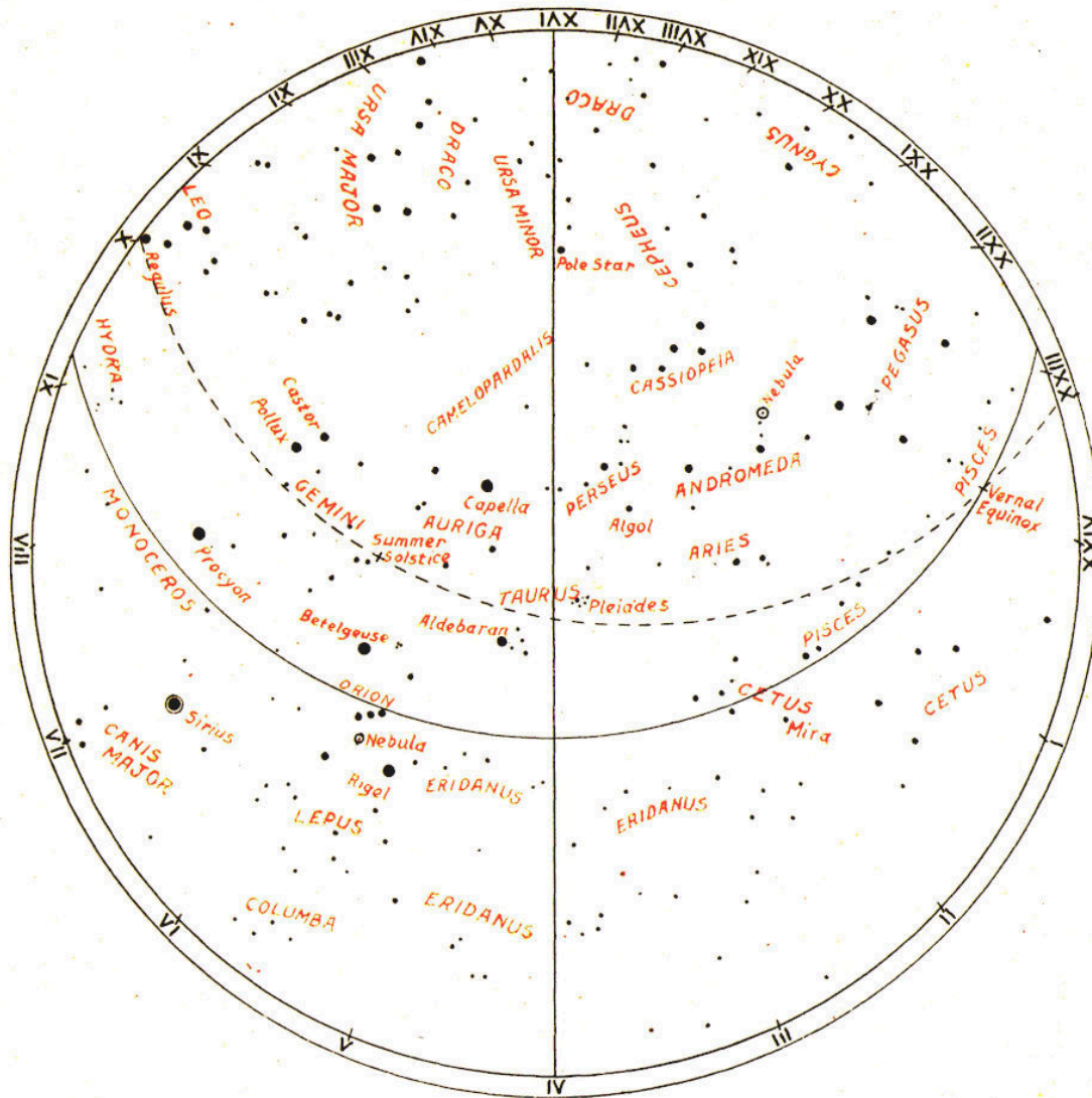
• CHART IV—THE WINTER EVENING SKY
