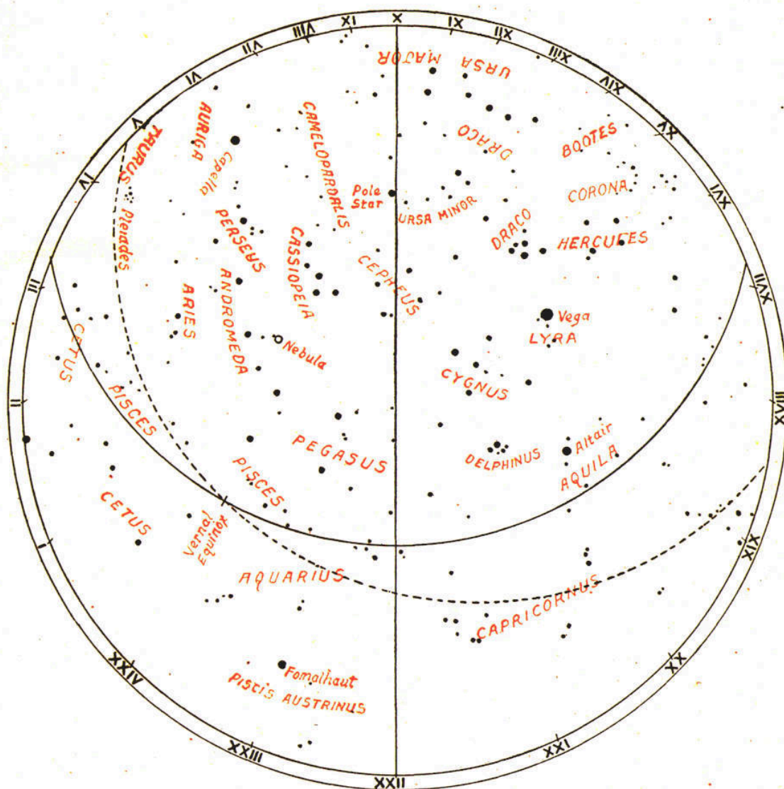
CHART III—THE AUTUMN EVENING SKY
