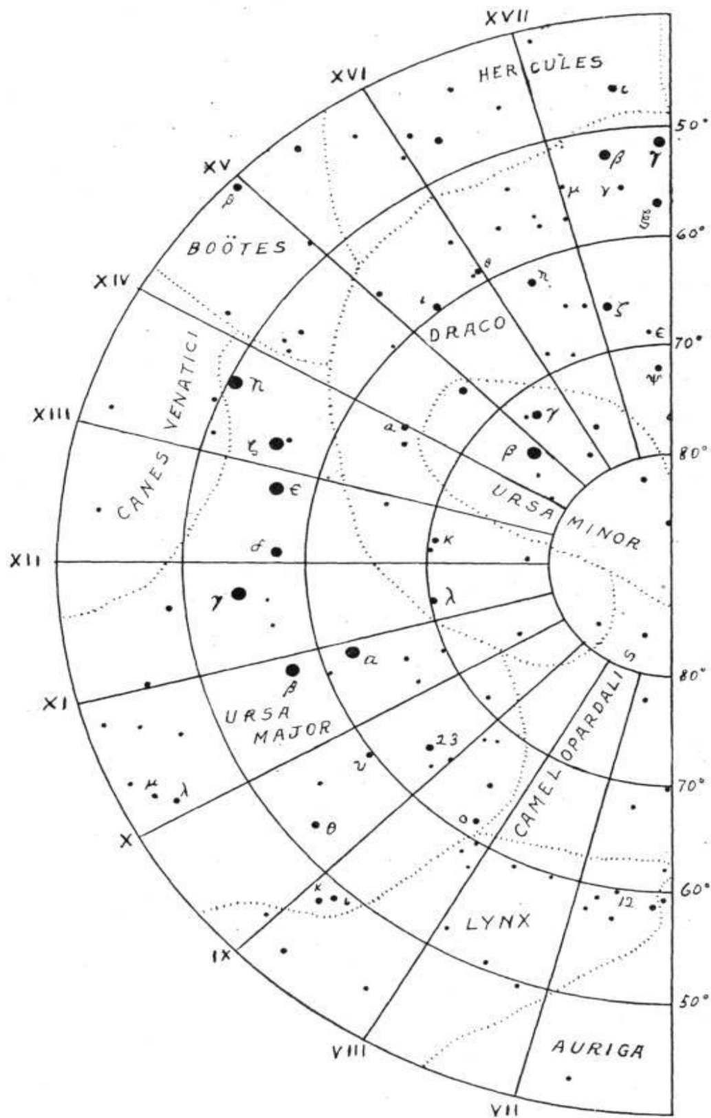
CHART IX—POLAR CONSTELLATIONS FROM VI H. TO XVIII H.
