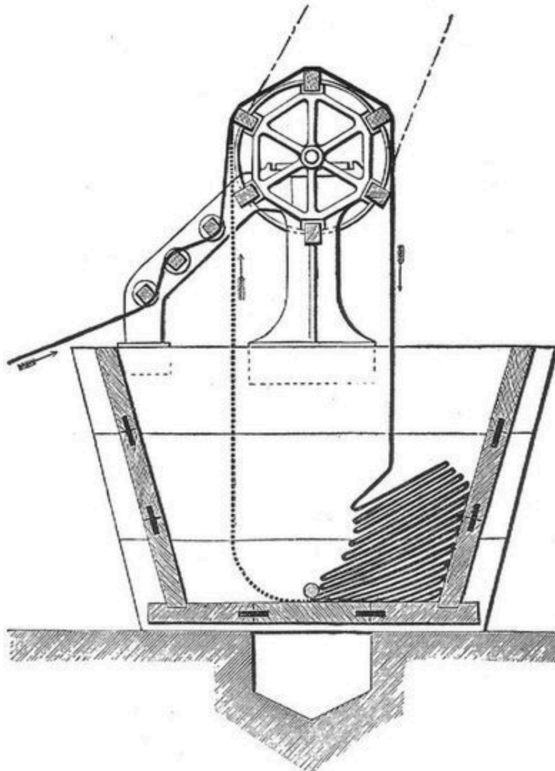
FIG. 19.—Wince Dye Beck.
