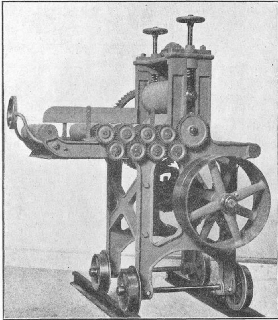
FIG. 24.—Read Holliday's Yarn-squeezing Machine.
