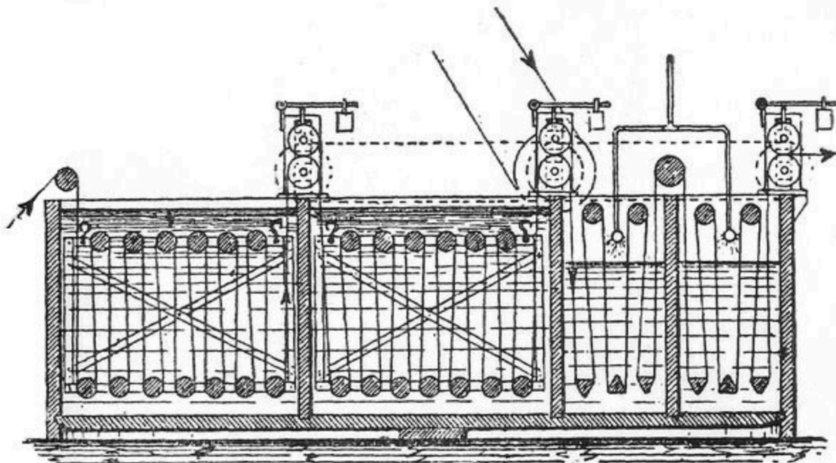
FIG. 28.—Soaping and Washing Machine.
