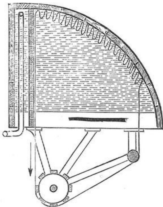
FIG. 20.—Plush Fabric Dyeing Machine.
