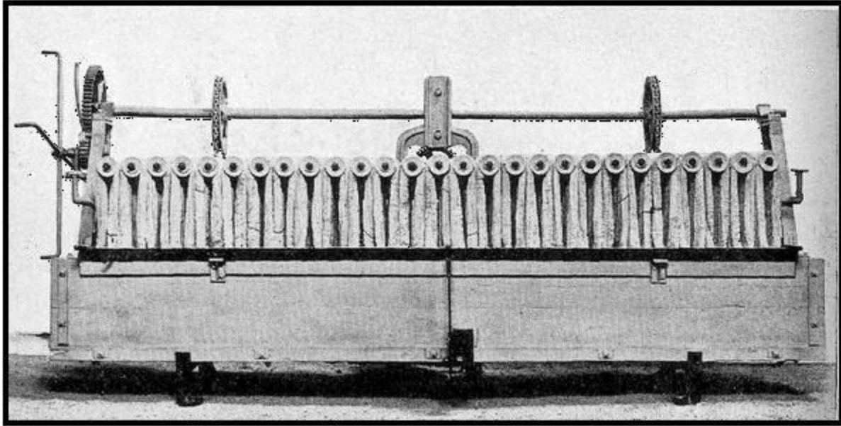
Fig. 14--Read Holliday's Yarn-dyeing Machine.
