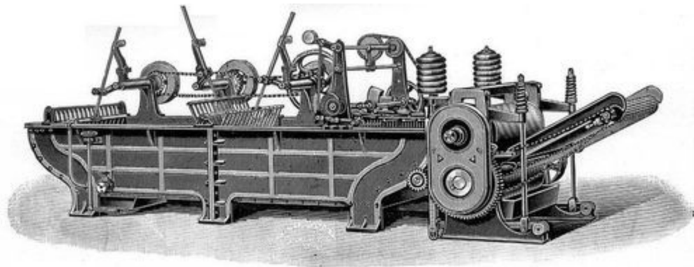
FIG. 6.—Wool-washing Machine.
