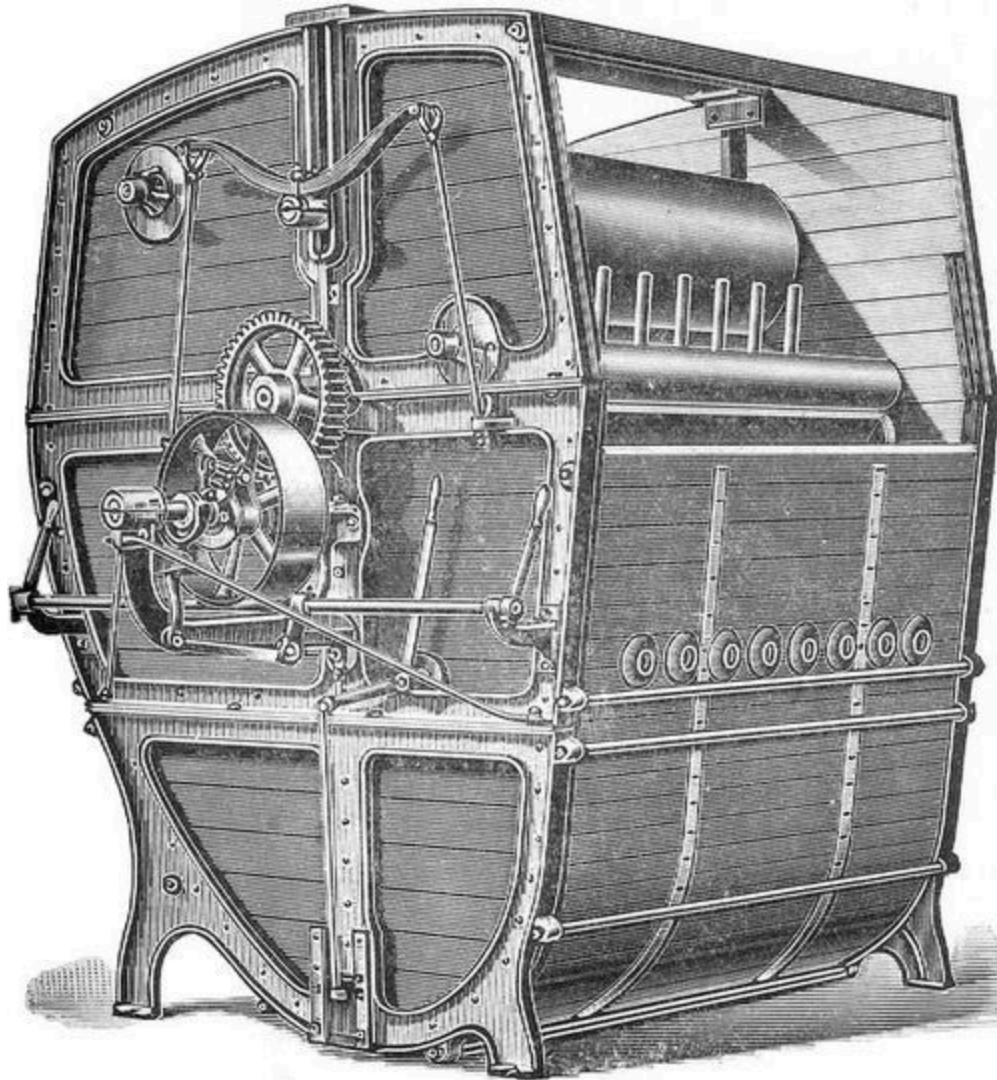
FIG. 27.—Cloth-washing Machine.
