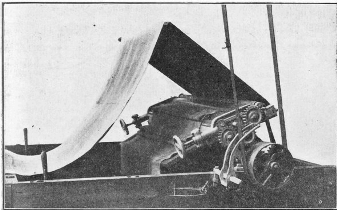
FIG. 22.—Read Holliday's Hawking Machine.
