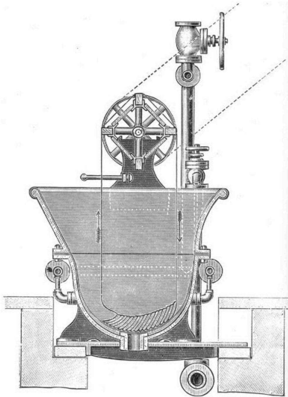
FIG. 21.—Copper Cased Dye Beck. Mather & Platt.
