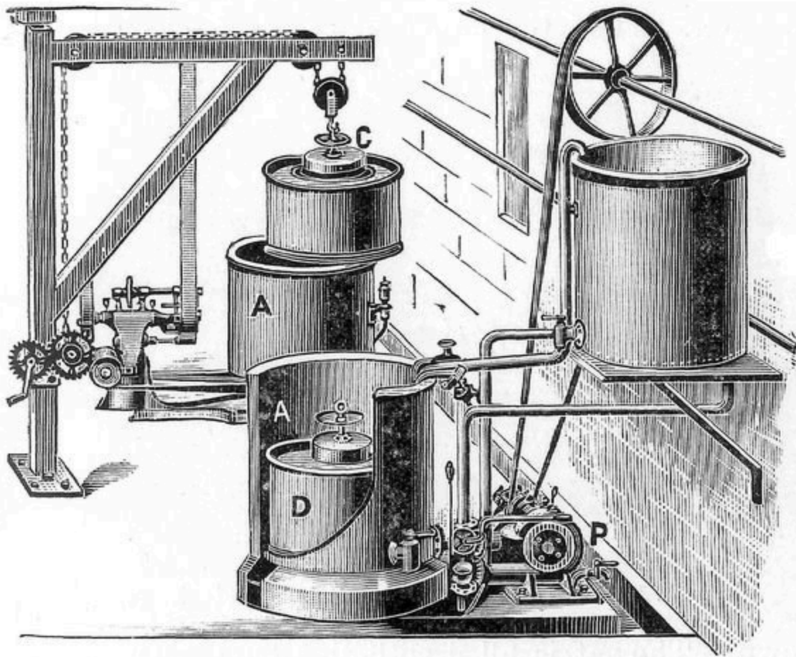
FIG. 13.—Obermaier Dyeing Machine.
