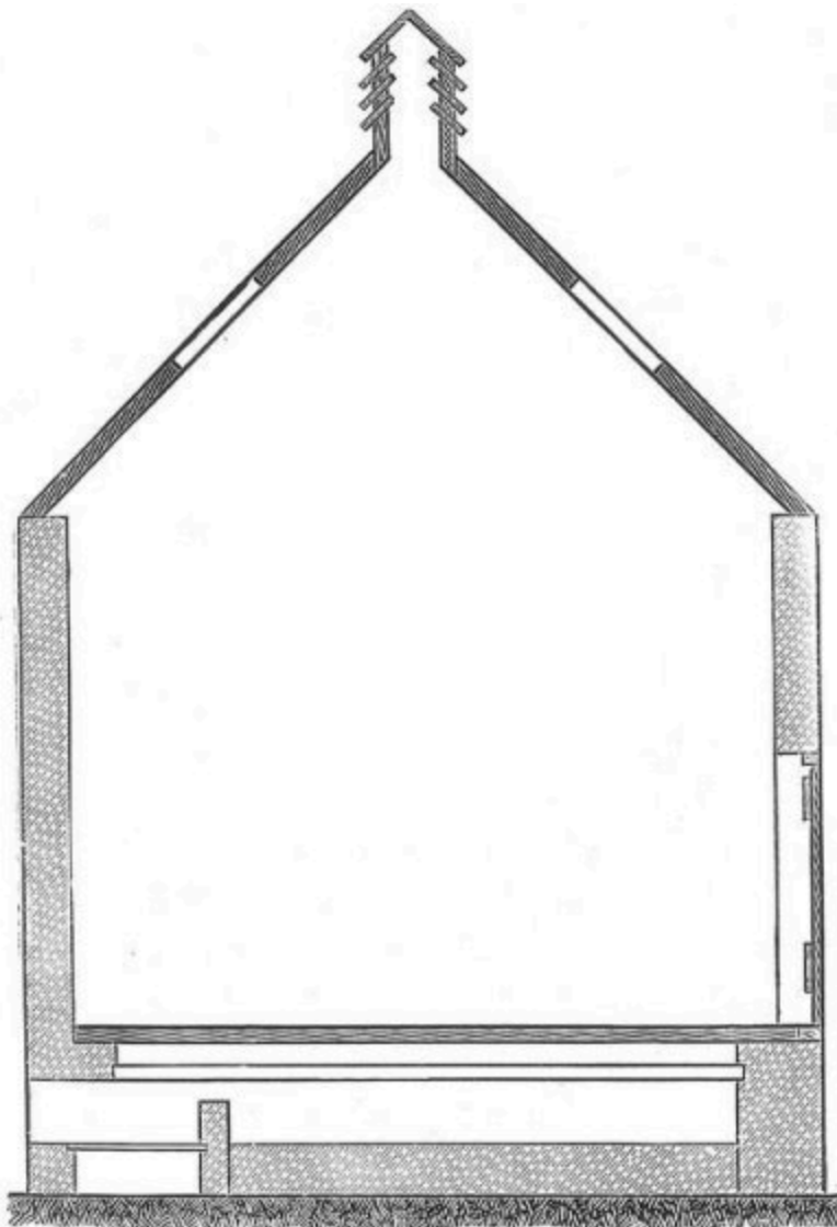
FIG. 9.—Sulphur Bleach House.
