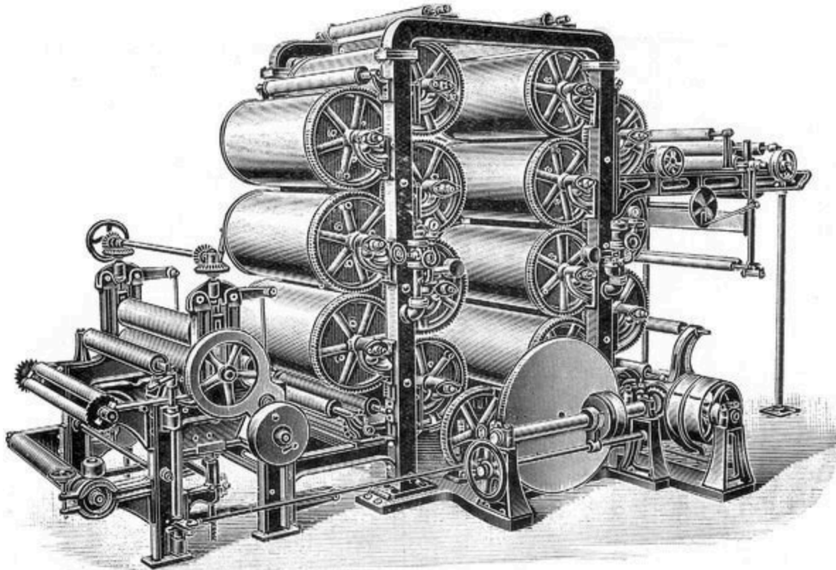
FIG. 32.—Cloth-drying Machine.
