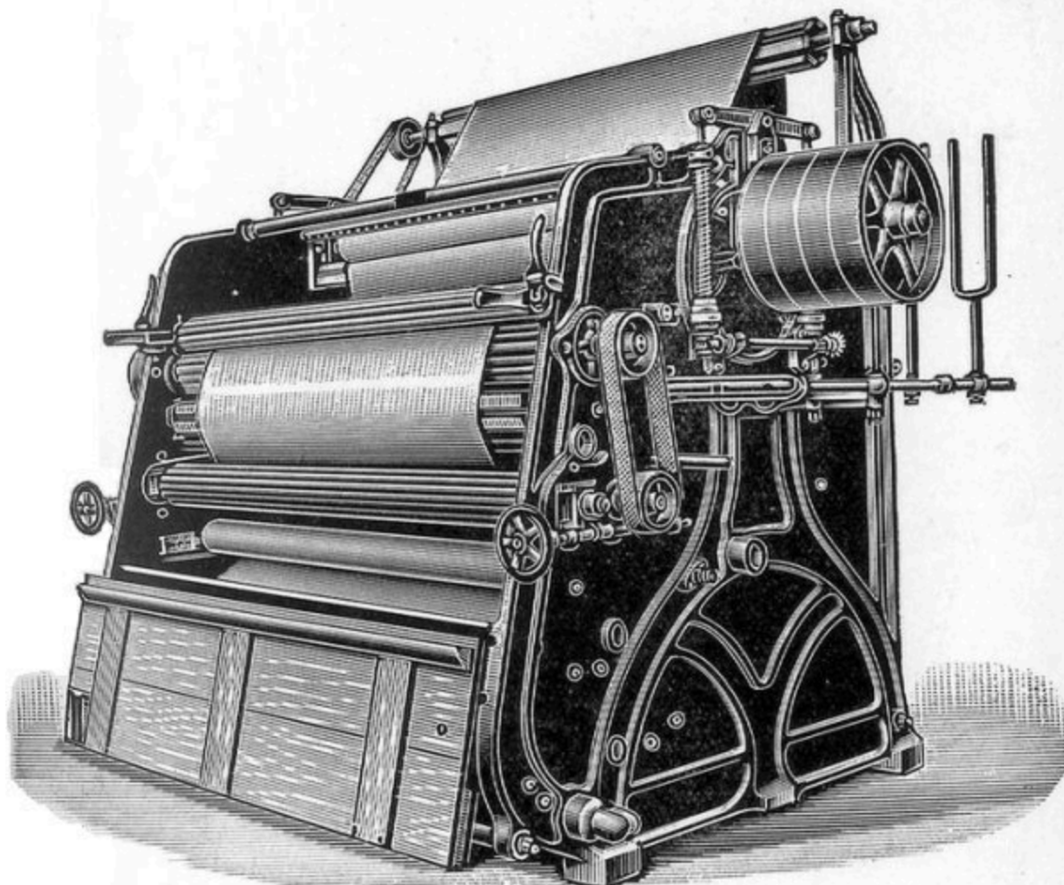
FIG. 7.—Cloth-washing Machine.
