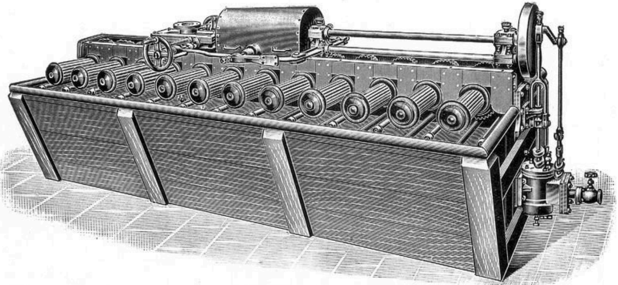
FIG. 25.—Hank-washing Machine.
