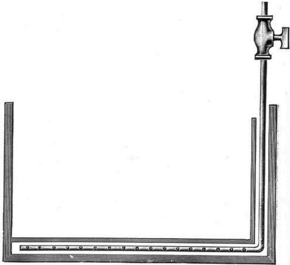
FIG. 11.—Dye-vat with Steam-pipe.
