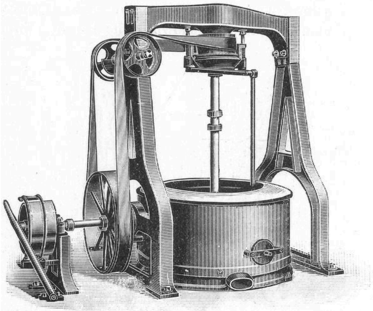
FIG. 29.—Hydro-extractor.
