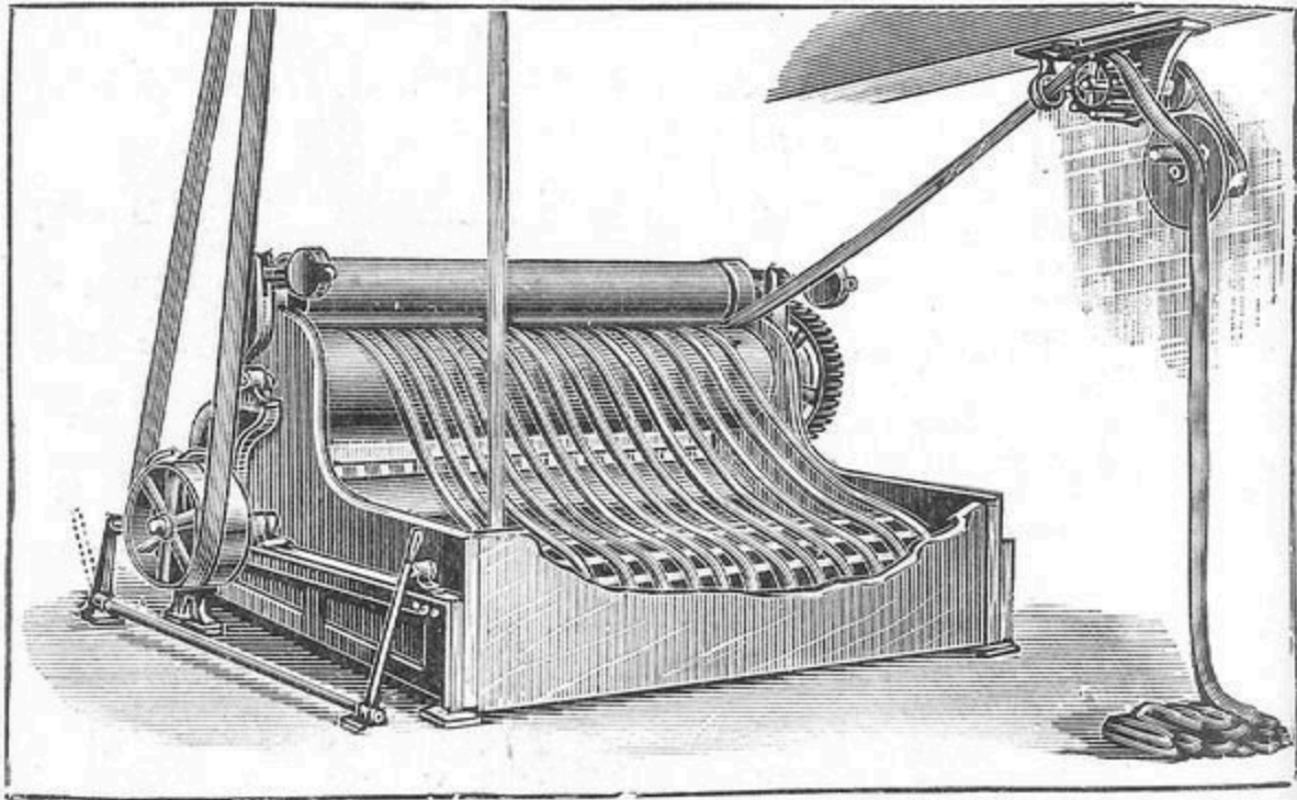
FIG. 26.—Cloth-washing Machine.
