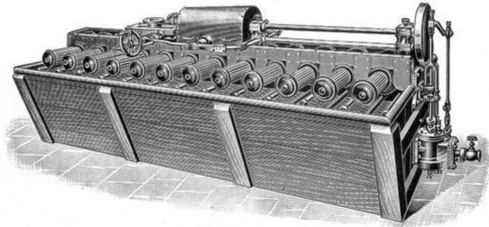
FIG. 25.—Hank-washing Machine.
