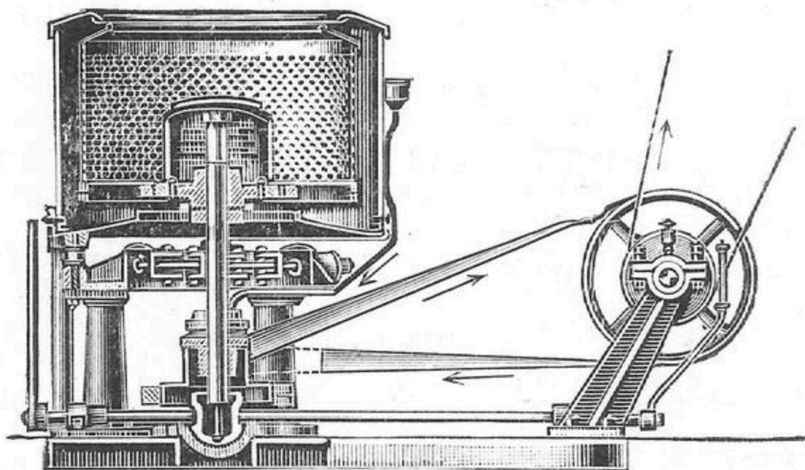
FIG. 30.—Hydro-extractor.
