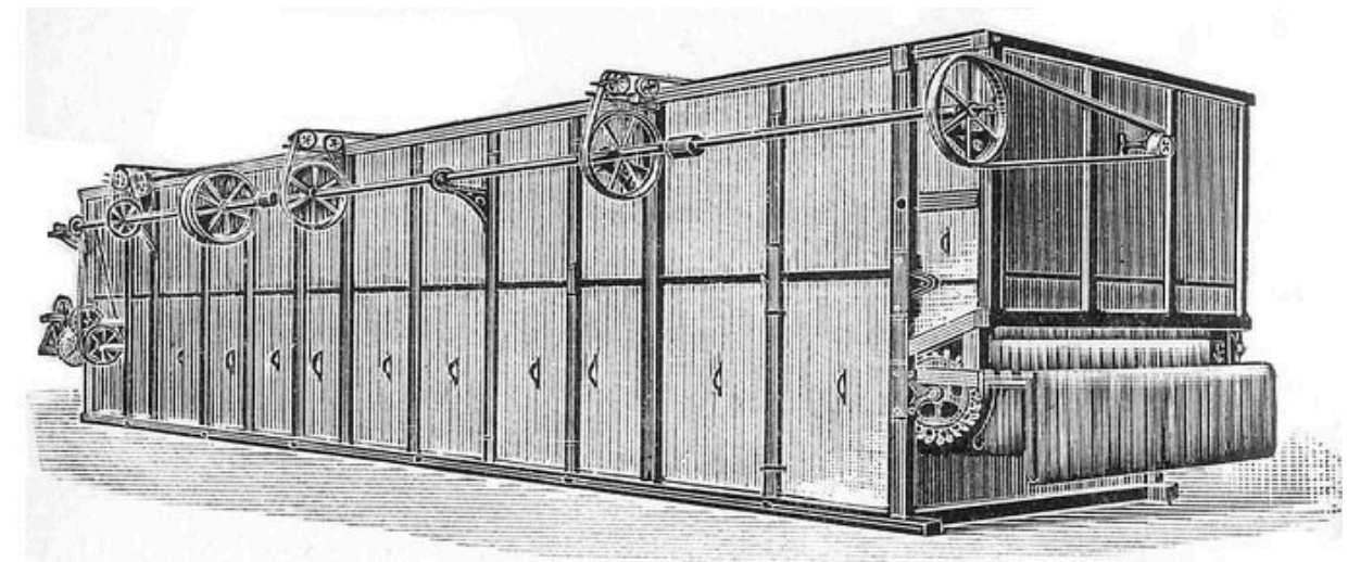
FIG. 31.—Yarn-drying Machine.
