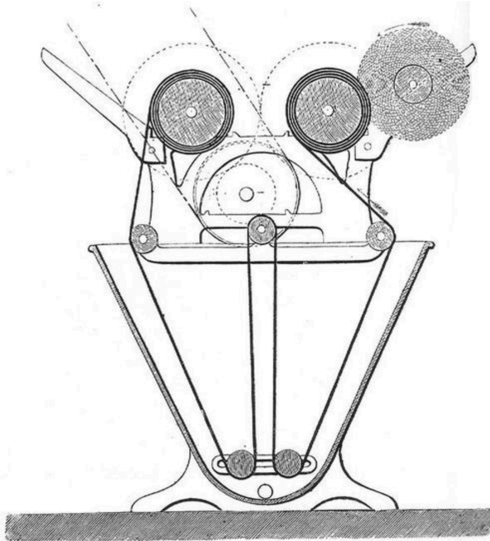
FIG. 17.—Dye-jigger in Section.
