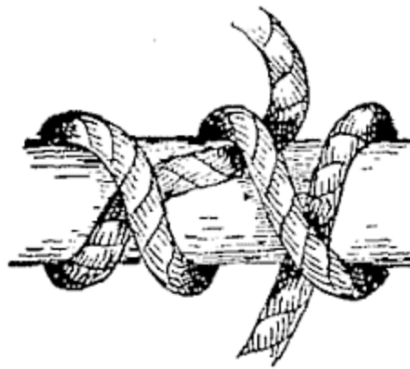
FIG. 48.—Rolling hitch.
