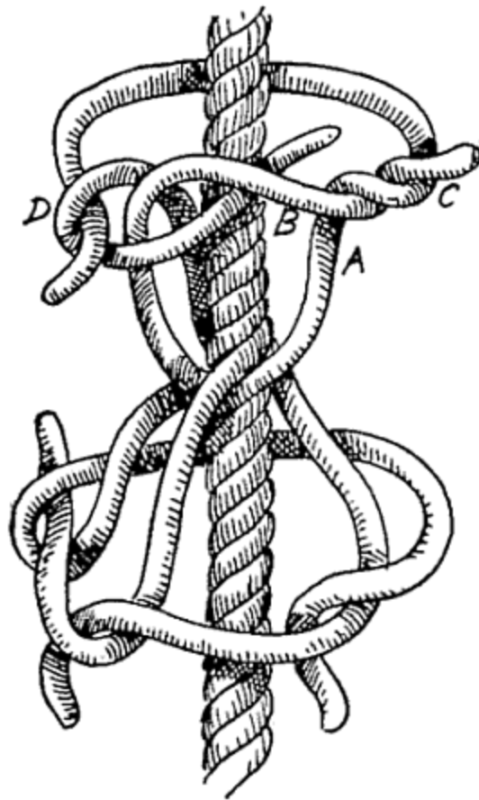
FIG. 119.—French shroud knot (making).
