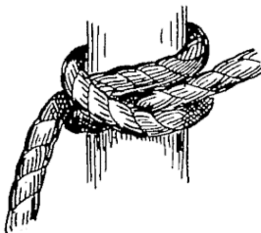
FIG. 36 B.—Clove hitch (complete).
