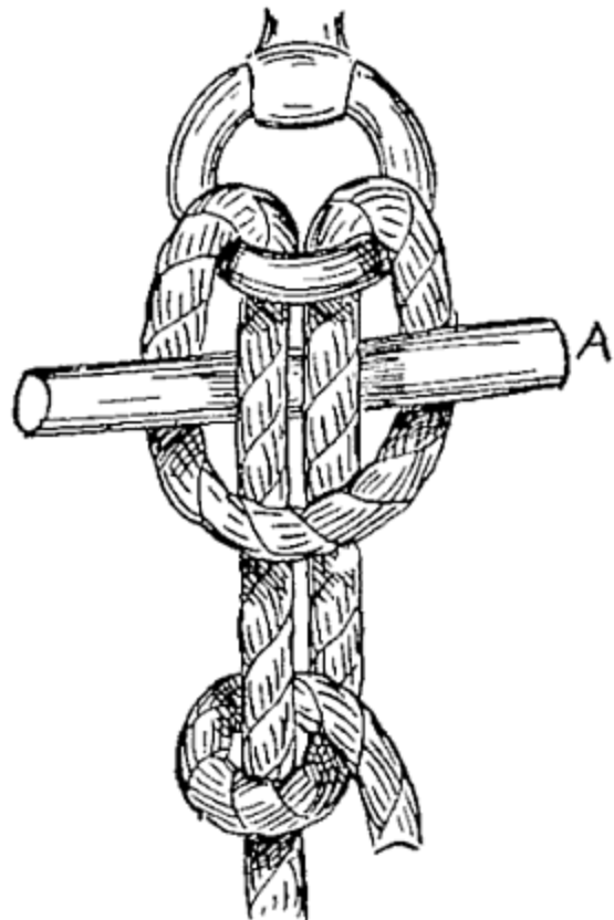
FIG. 30.—Lark's head with toggle (A).
