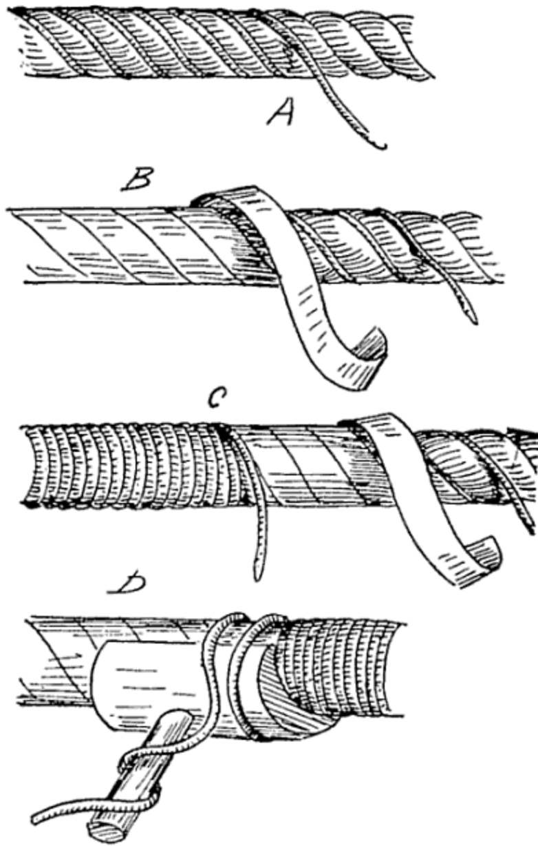
FIG. 138.—Worming, parcelling, and serving.
