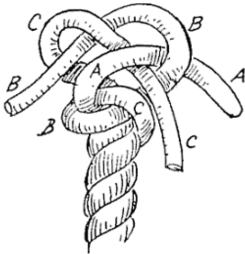
FIG. 124.—Wall crowned (making).
