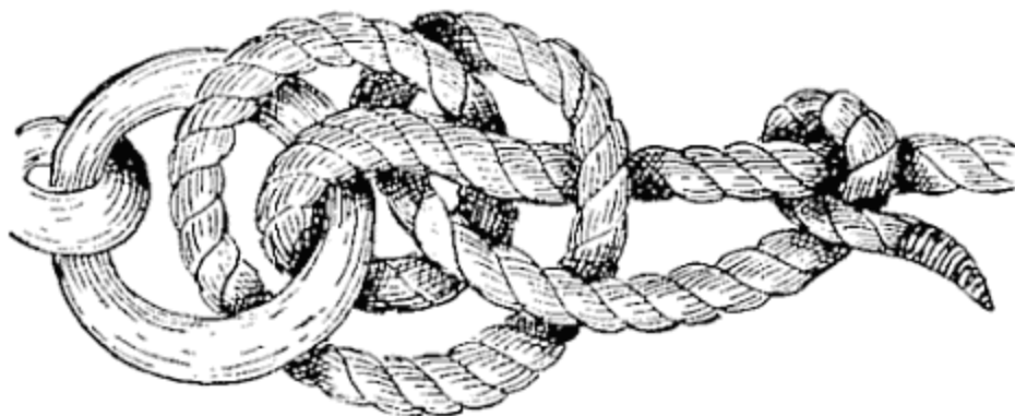
FIG. 53.—Fisherman's hitch.
