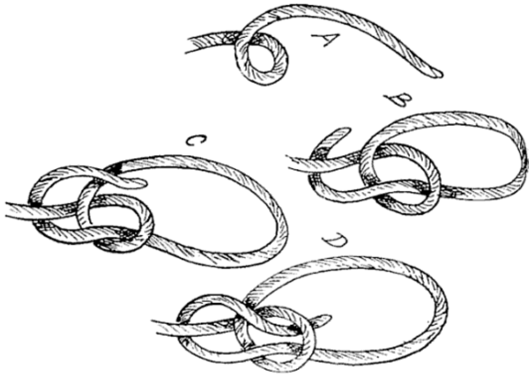
FIG. 59.—Tying bow-line.
