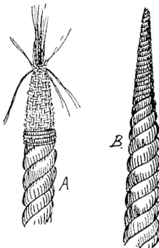
FIG. 103.—Pointing a rope.
