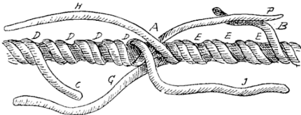
FIG. 107.—Long splice.
