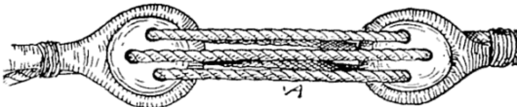
FIG. 98.—Deadeye lashing.
