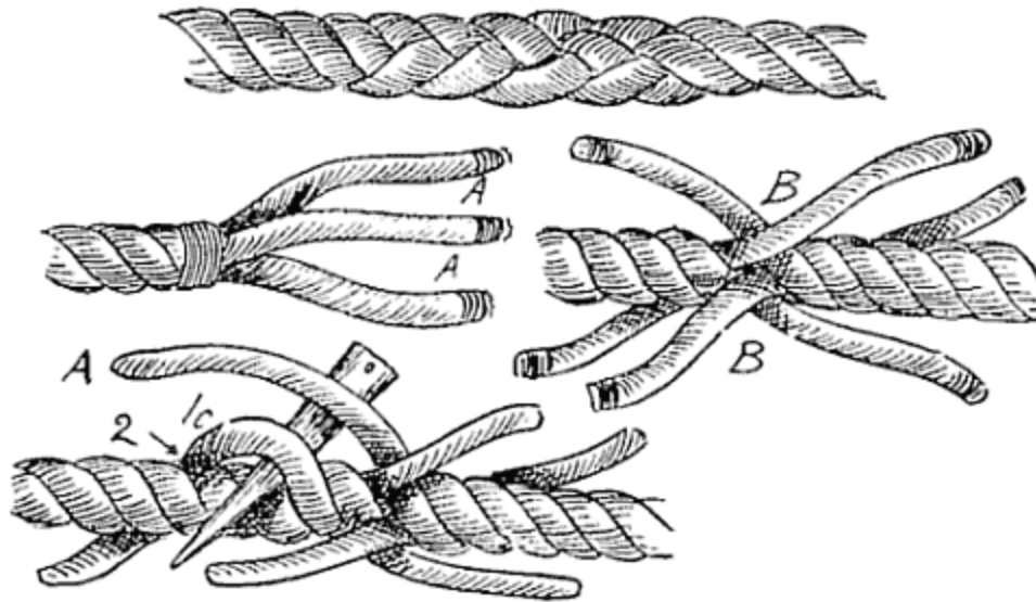
FIG. 106.—Short splice.
