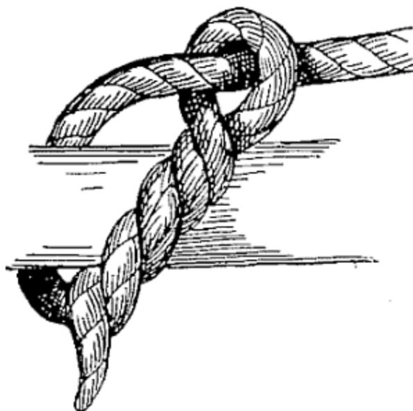
FIG. 38.—Timber hitch.
