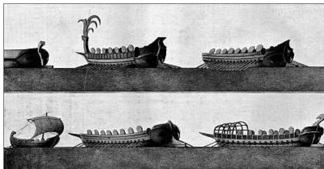
ROMAN WARSHIPS
