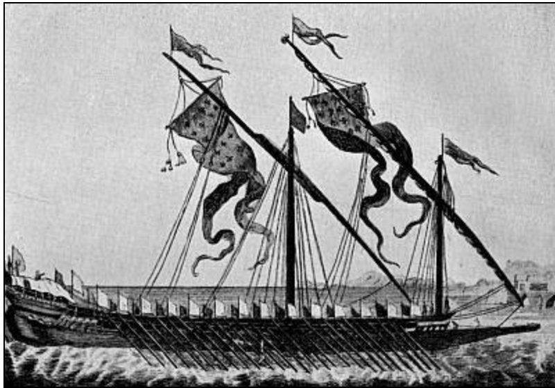
A GALLEY
