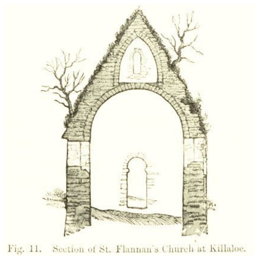
Fig. 11. Section of St. Flannan's Church at Killaloe.
