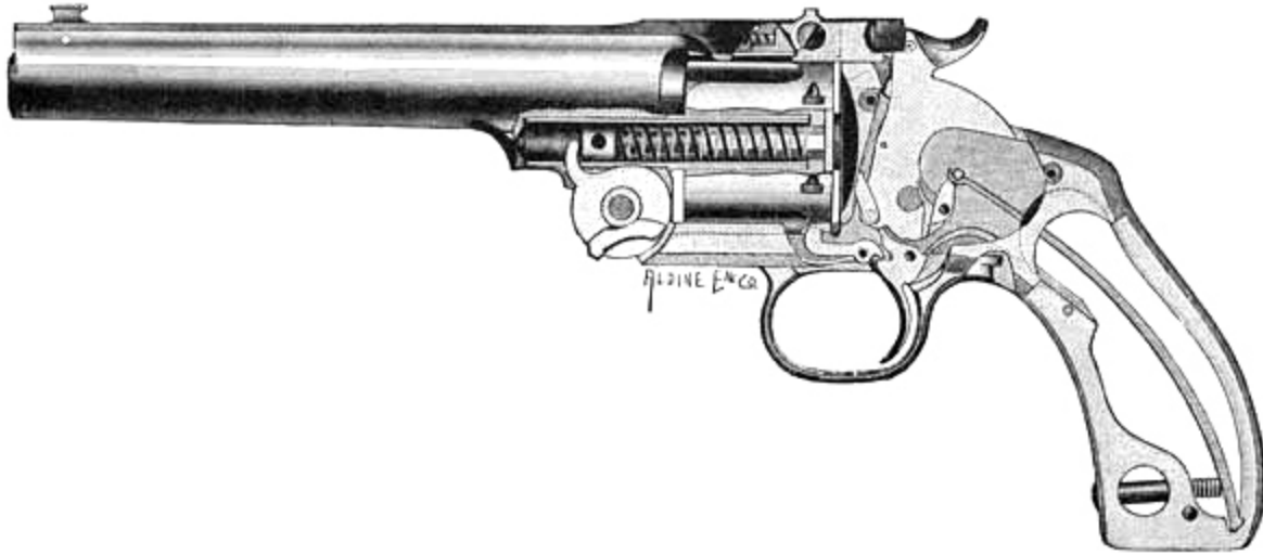
SMITH & WESSON REVOLVER, RUSSIAN MODEL, .44 CALIBRE, SINGLE ACTION.
