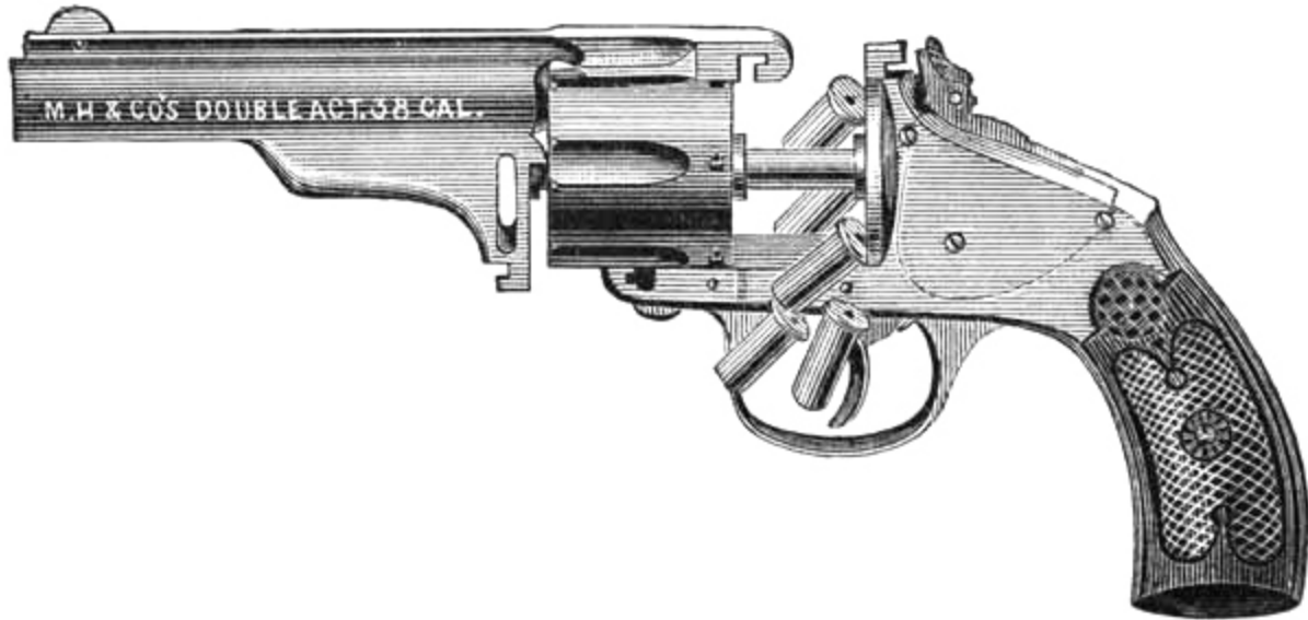
Revolver open, showing manner of ejecting shells.
