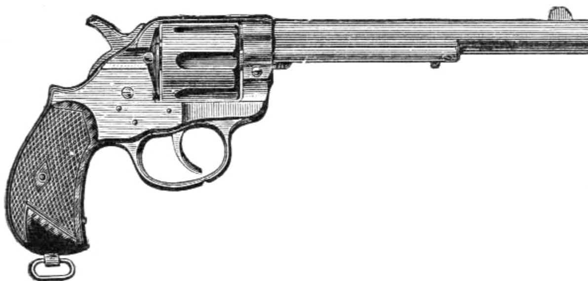
COLT'S FRONTIER MODEL AND ARMY, DOUBLE ACTION.
