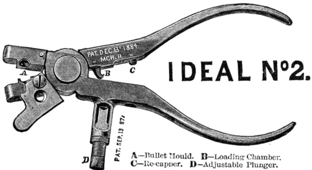
THE IDEAL RELOADING TOOL, FOR PISTOL AND REVOLVER CARTRIDGES.
