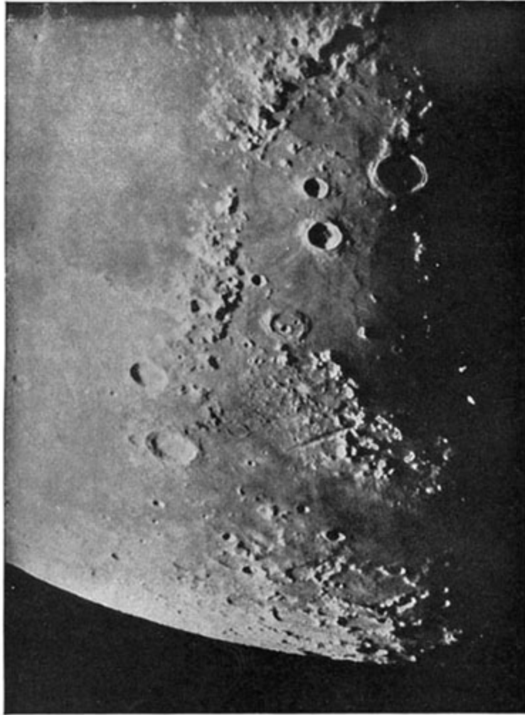
THE LUNAR ALPS, APENNINES, AND CAUCASUS. Photographed with the Lick Telescope.
