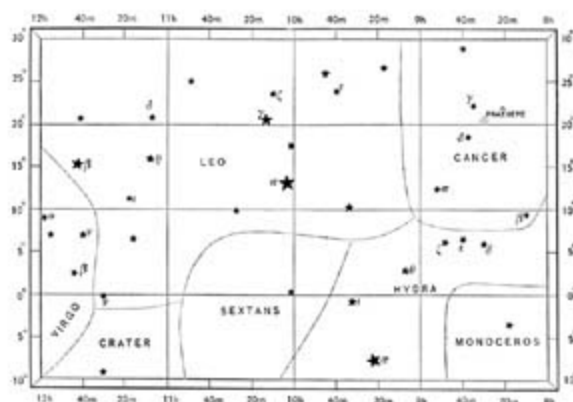
CHART NO. 3.—FROM RIGHT ASCENSION 8 HOURS TO 12 HOURS; DECLINATION 30^{\circ} NORTH TO 10^{\circ} SOUTH.
