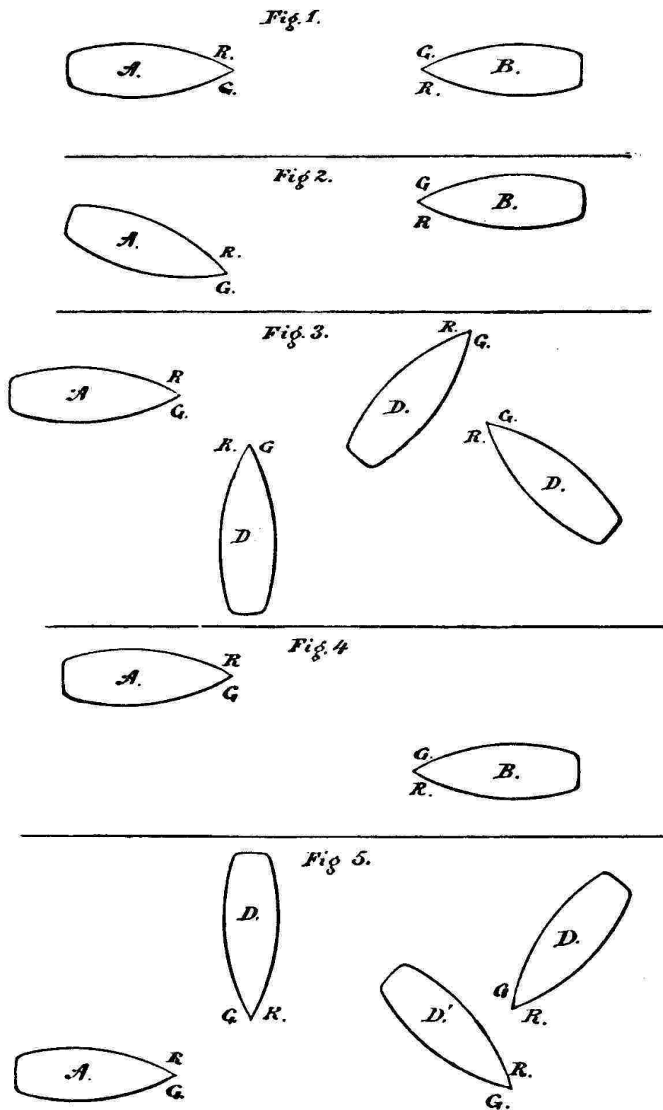
FIG. 1 (when the red and green lights are both seen).—A sees a red and green light ahead. A knows that a vessel is approaching him on a course
