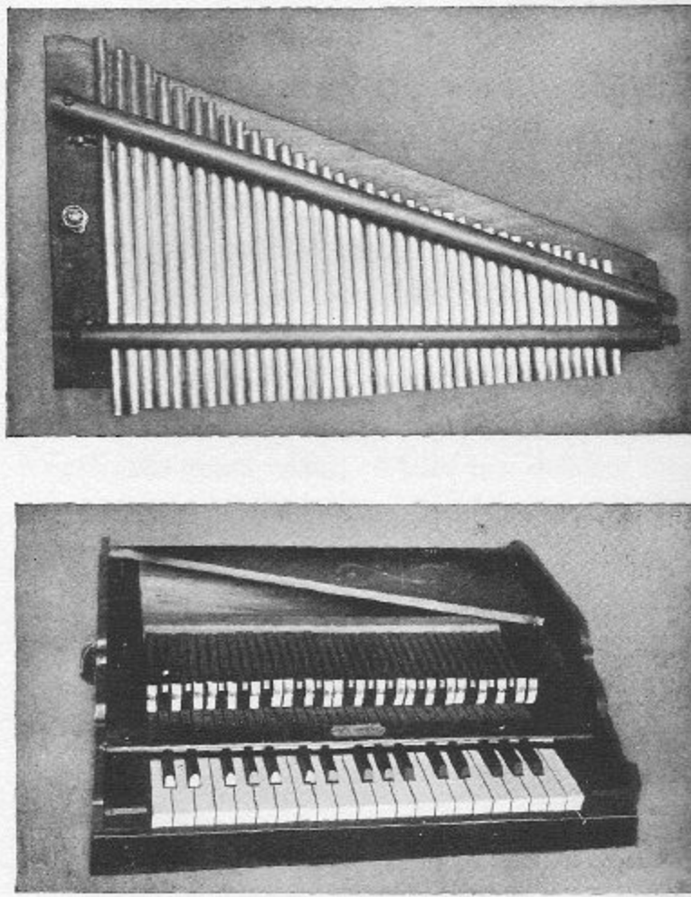
FIG. 39.—DUMB KEYBOARD.
