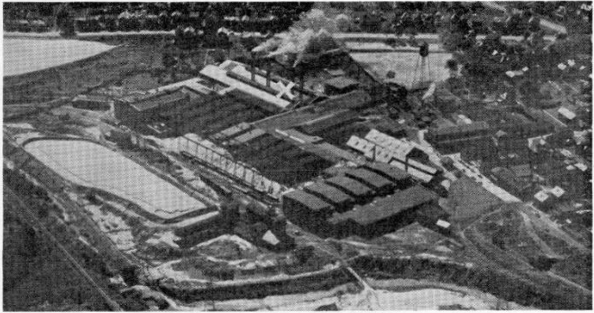
FIGURE 11.—Standard Plate Glass Company, Butler, Pennsylvania, with x marking building where Peate's 62-inch disc was cast. (From Preston, fig. 1.)
