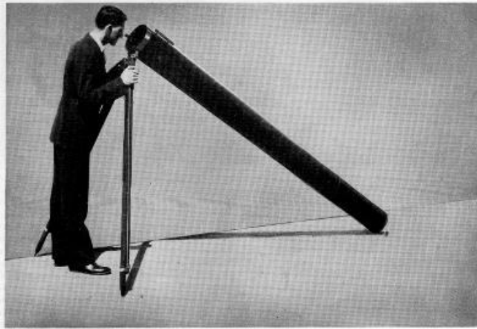
FIGURE 2.—Herschelian reflecting telescope (USNM 310598) built by Amasa Holcomb and shown by him at the Franklin Institute, Philadelphia, in 1835. The Institute's report of the demonstration is given in the appendix (p. 182). ( Smithsonian photo 11000-a )
