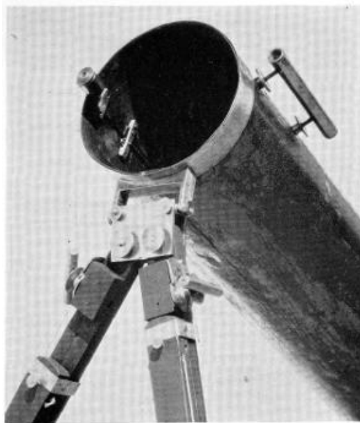
FIGURE 3.—Eyepiece and tripod head of the Holcomb reflecting telescope shown in figure 2. ( Smithsonian photo 11000 )
