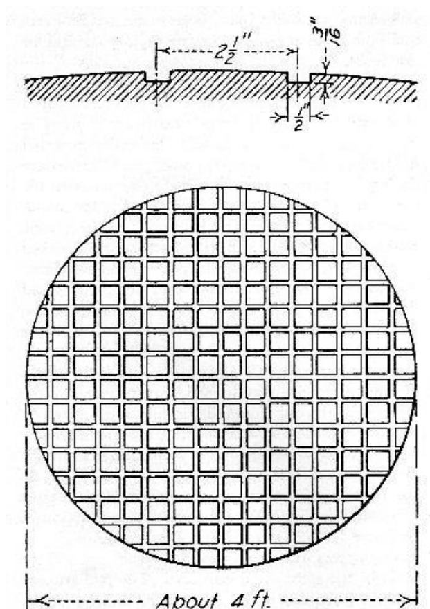
FIGURE 13.—Face of largest grinding tool made by Hodge for Peate. (From Preston, fig. 5b.)
