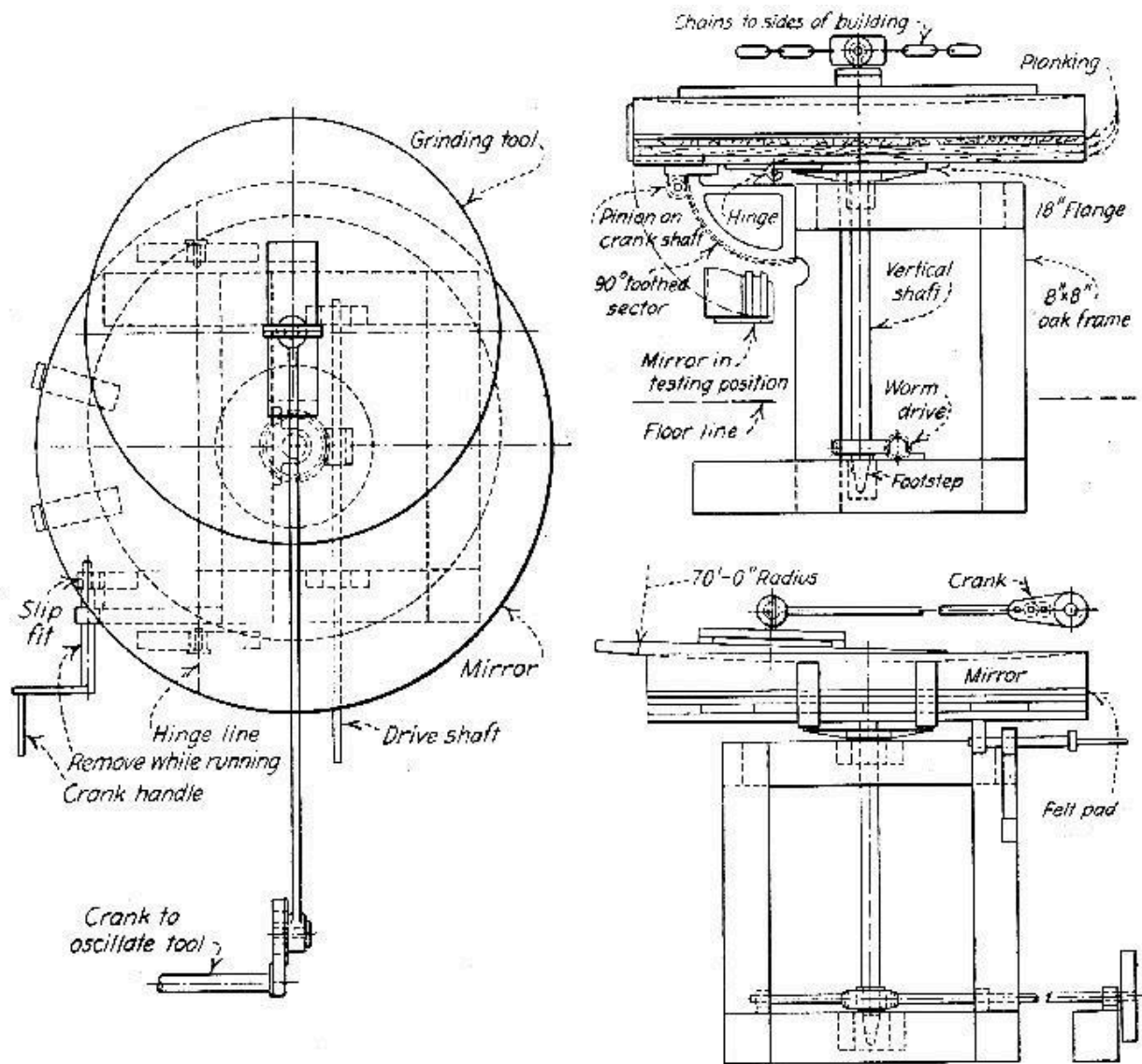
FIGURE 14.—Surfacing machine used by Peate. (From Preston, fig. 4.)
