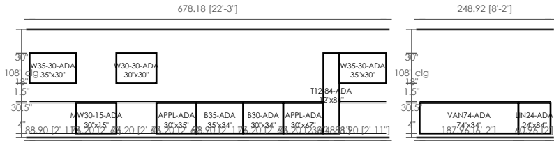
FRONT ELEVATION VIEW
