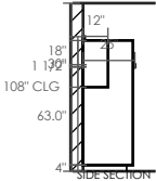
SIDE SECTION VIEW
