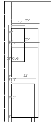
SIDE SECTION SIDE SECTION VIEW
