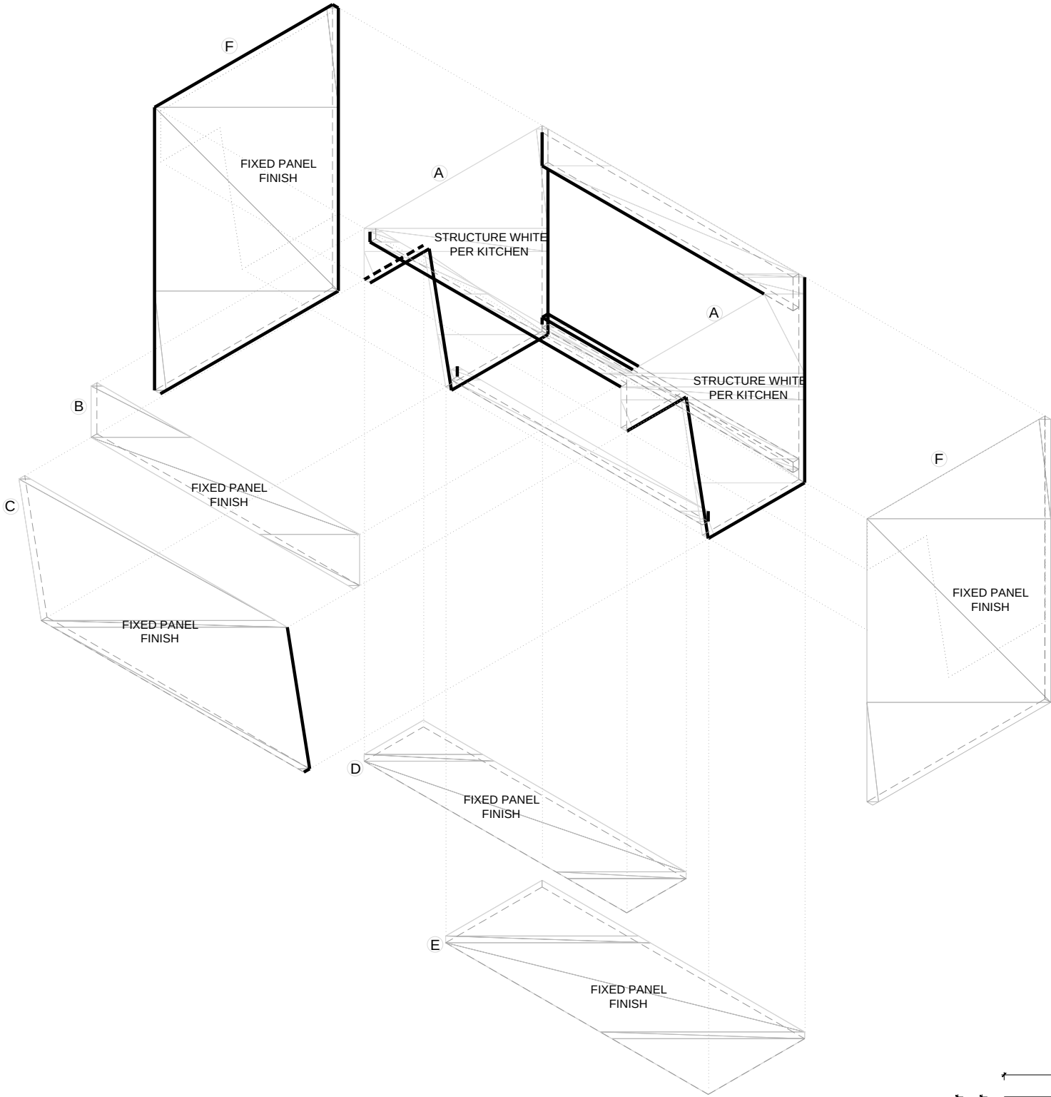
PARTS BY KITCHEN SCALE 1/2"=1'-0" KITCHEN ADA SINK
