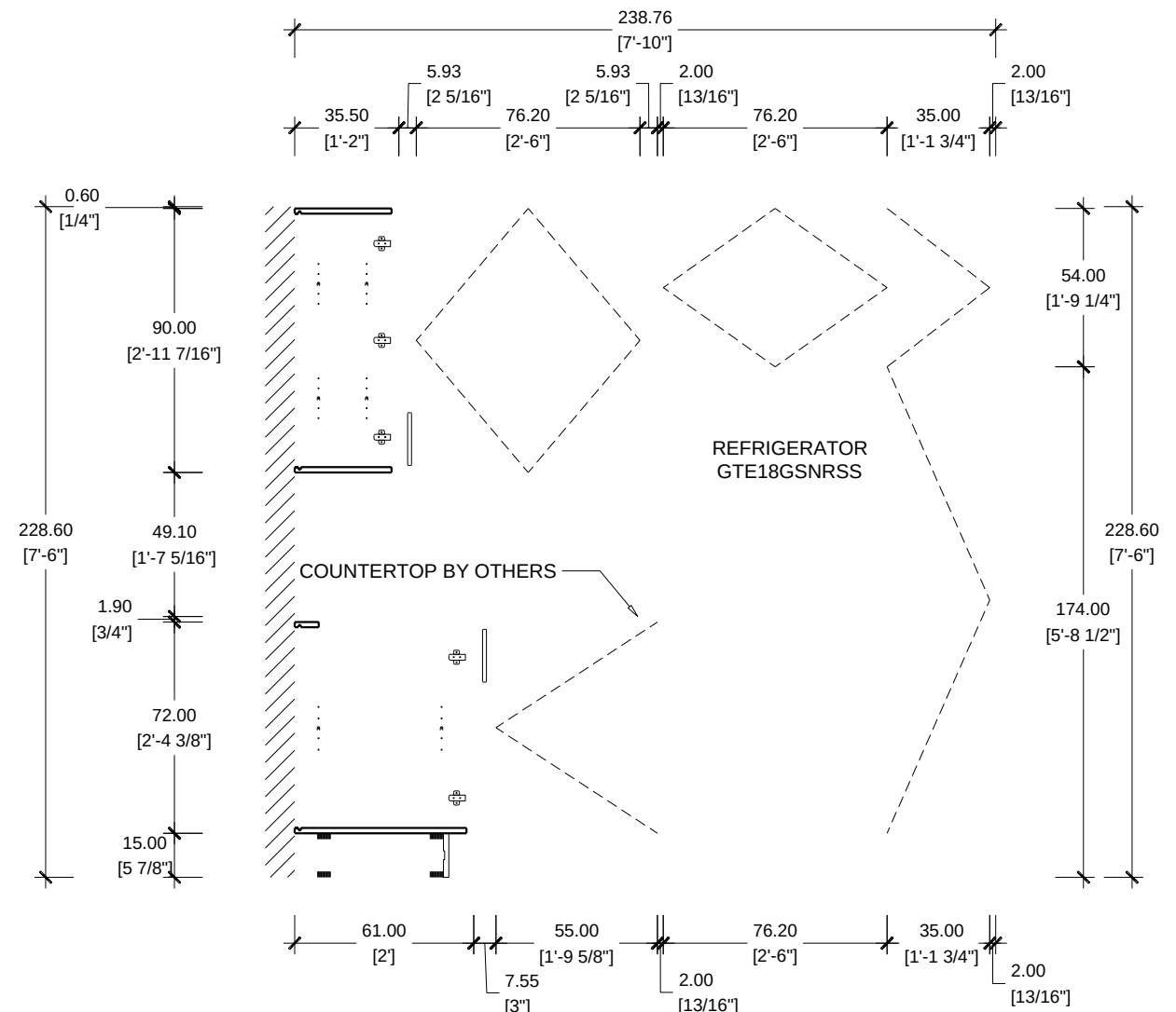
ELEVATION B CASA FAMILIA UNIT A1 / KITCHEN TYPE K1
