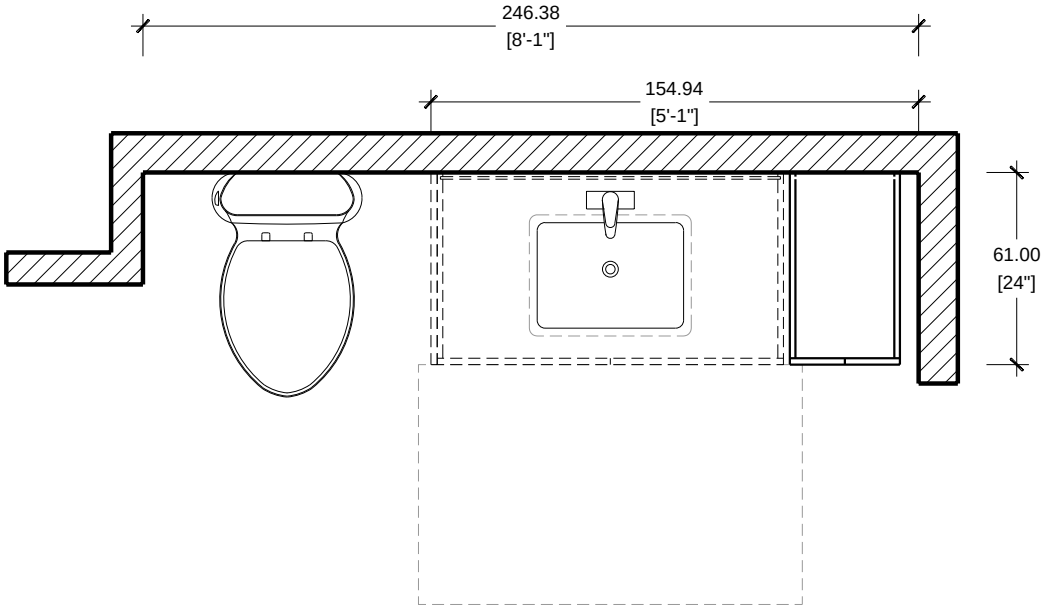
FLOOR PLAN SCALE 1/2"=1'-0" CASA FAMILIA UNIT A1 /VANITY TYPE V1
