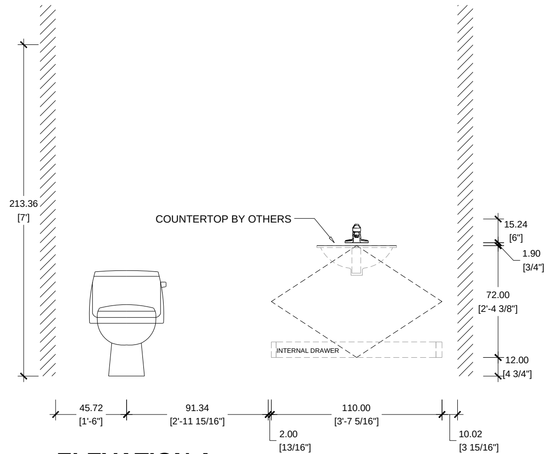
ELEVATION A CASA FAMILIA UNIT B1 / VANITY TYPE V4
