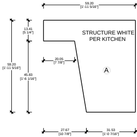
PARTS BY KITCHEN SCALE 1/2"=1'-0" KITCHEN | BASE 90 CM
