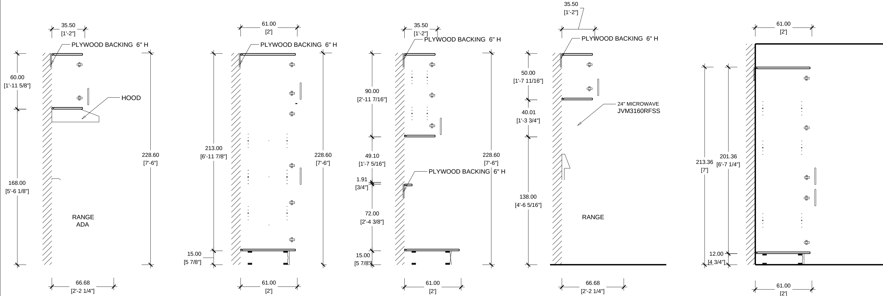
SECTION MICROWAVE KITCHEN
