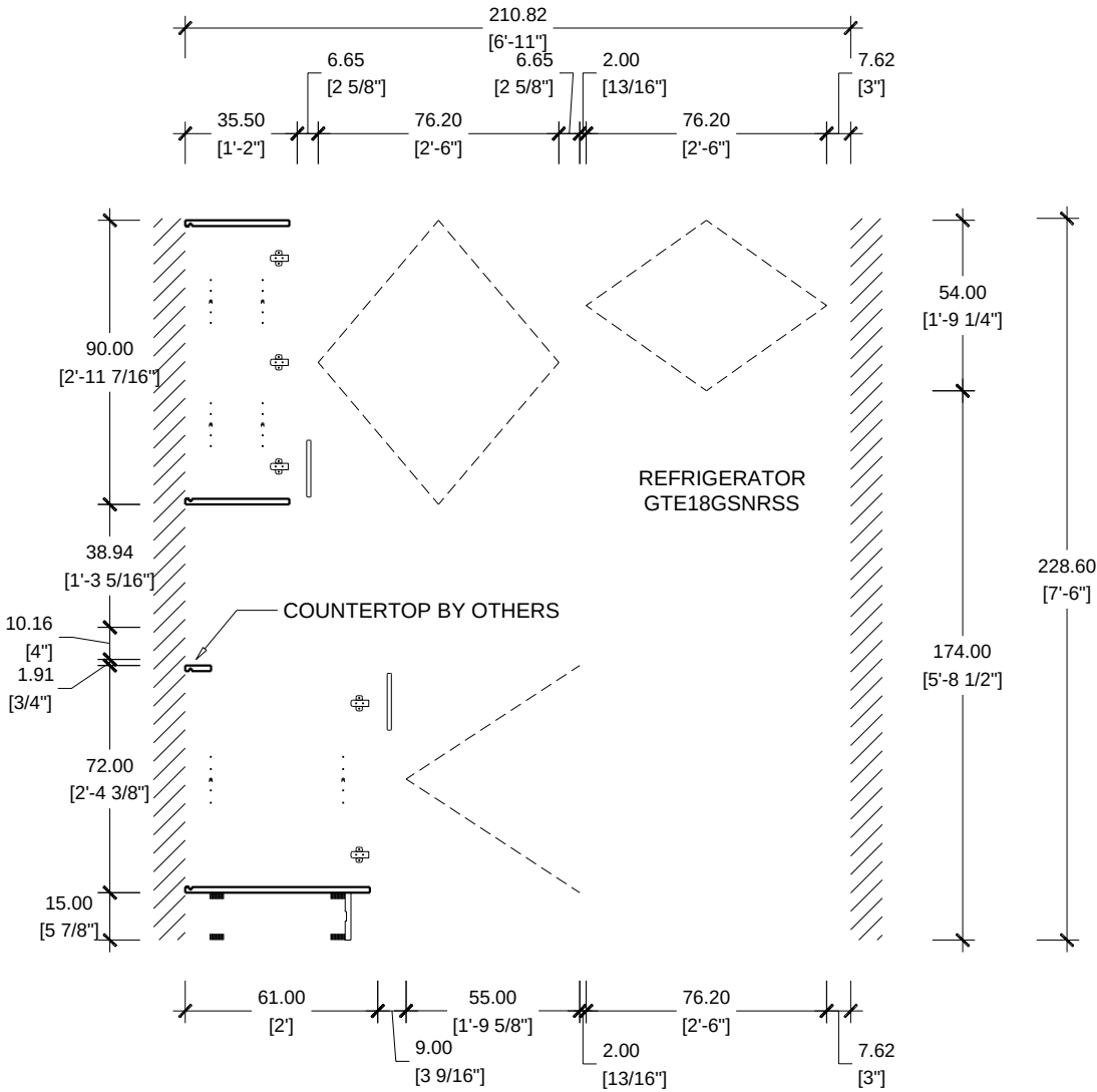
ELEVATION B CASA FAMILIA UNIT B1 / KITCHEN TYPE K3
