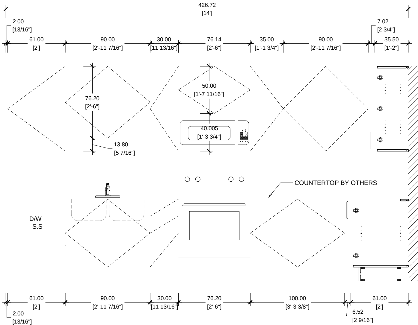
ELEVATION A CASA FAMILIA UNIT A3 / KITCHEN TYPE K1
