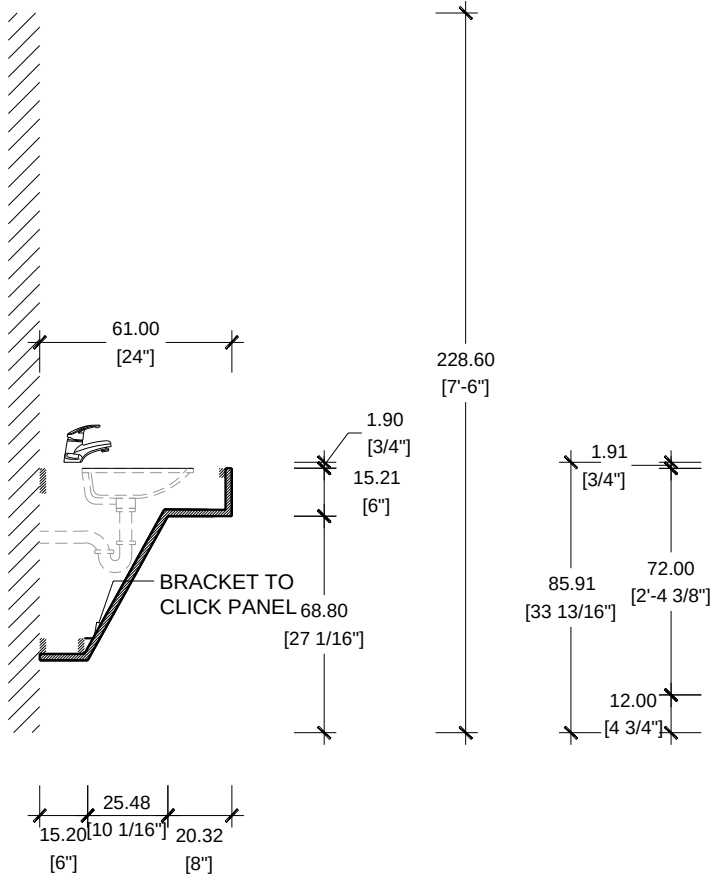
SECTION SCALE 1/2"=1'-0" VANITY ADA
