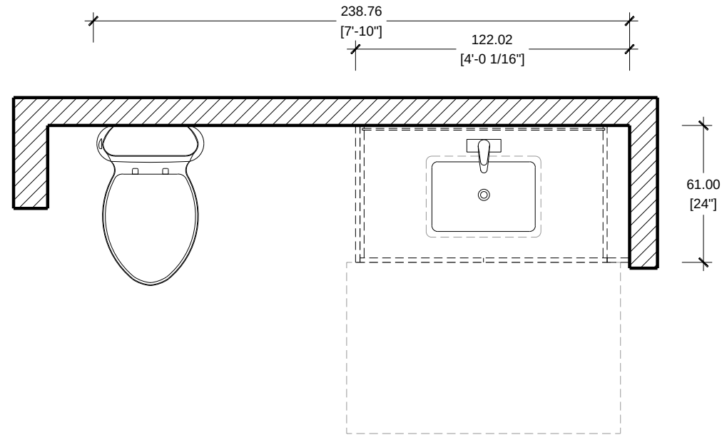
FLOOR PLAN SCALE 1/2"=1'-0" CASA FAMILIA / VANITY TYPE V4
