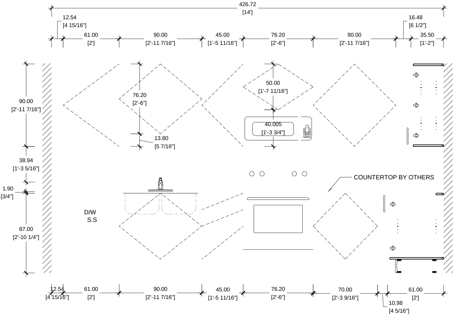
ELEVATION A CASA FAMILIA UNIT B1 / KITCHEN TYPE K3
