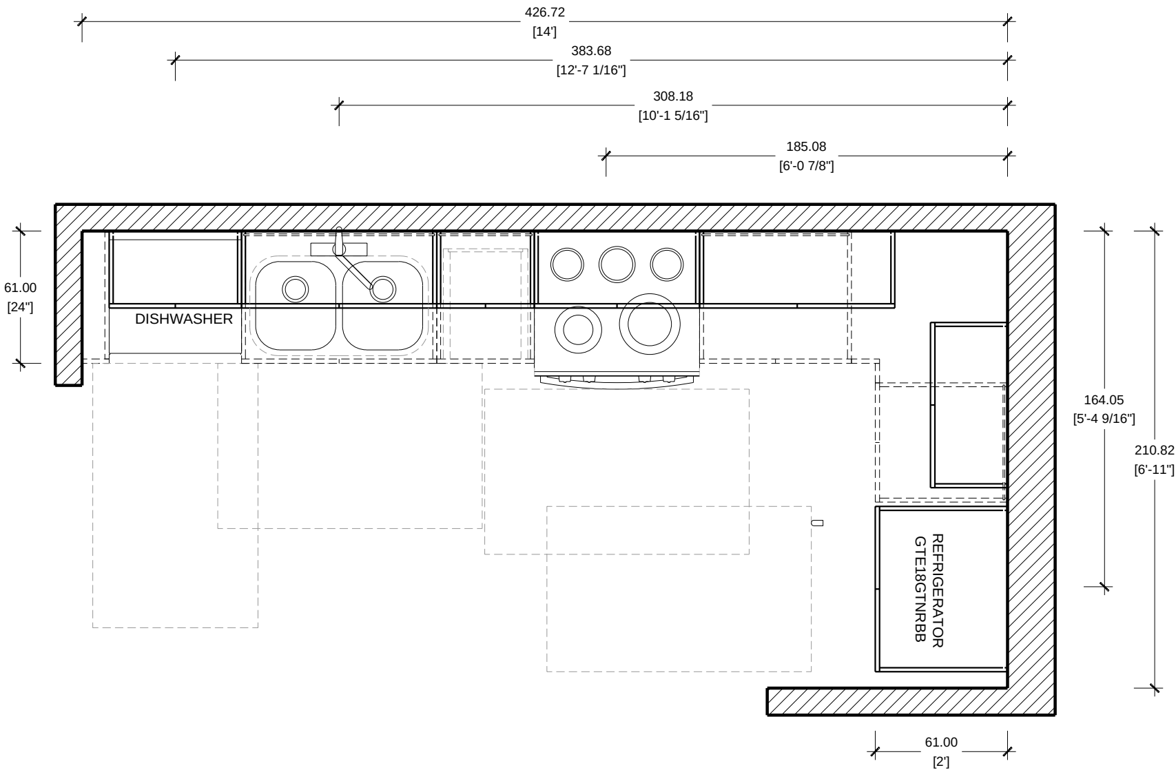
FLOOR PLAN SCALE 1/2"=1'-0" CASA FAMILIA UNIT B1/ KITCHEN TYPE K3
