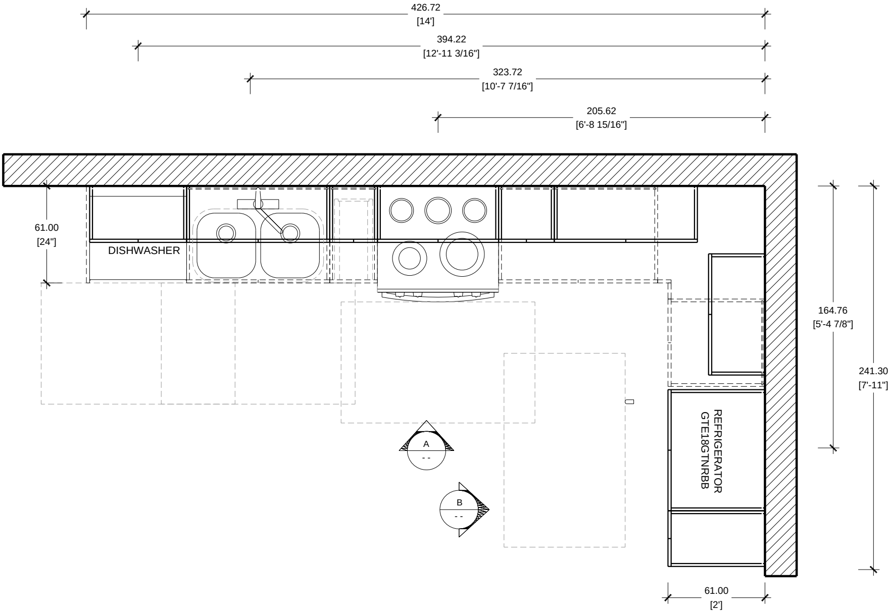
FLOOR PLAN SCALE 1/2"=1'-0" CASA FAMILIA UNIT A3/ KITCHEN TYPE K1
