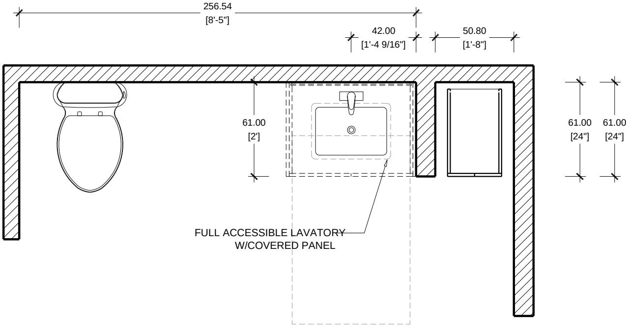
FLOOR PLAN SCALE 1/2"=1'-0" CASA FAMILIA /VANITY TYPE RV2
