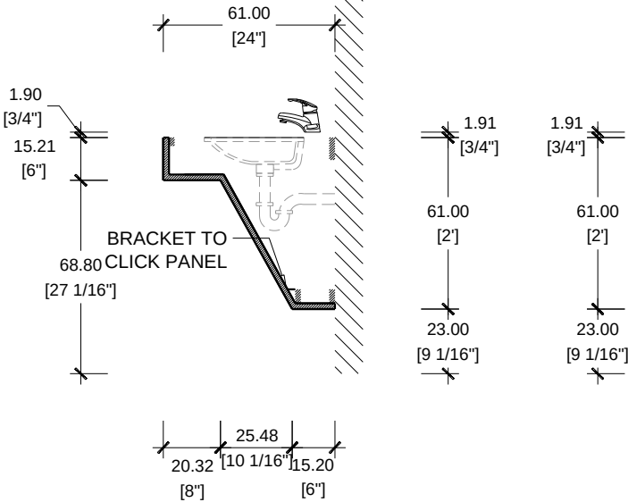
SECTION SCALE 1/2"=1'-0" CASA FAMILIA / VANITY TYPE RV2
