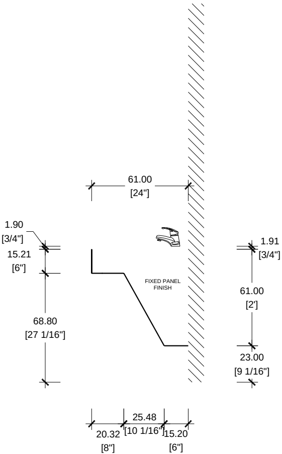
SIDE VIEW SCALE 1/2"=1'-0" CASA FAMILIA / VANITY TYPE V2
