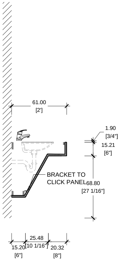
SECTION SCALE 1/2"=1'-0" CASA FAMILIA UNIT A2 FA/ VANITY TYPE V2
