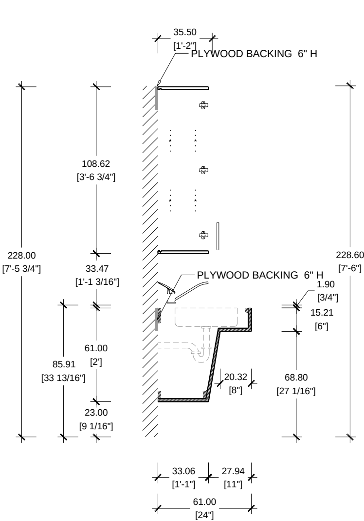
SECTION SCALE 1/2"=1'-0" KITCHEN ADA
