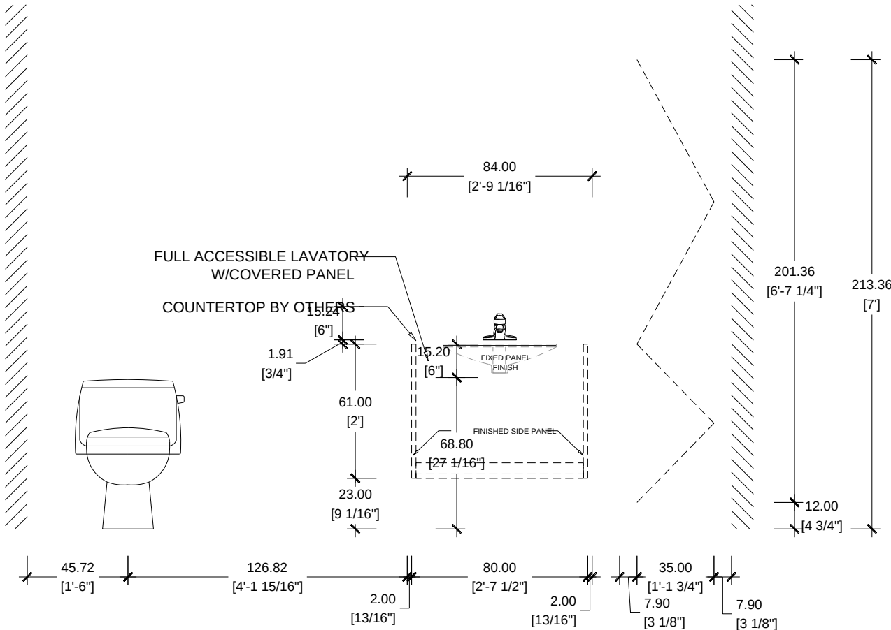
ELEVATION A CASA FAMILIA / VANITY TYPE RV2
