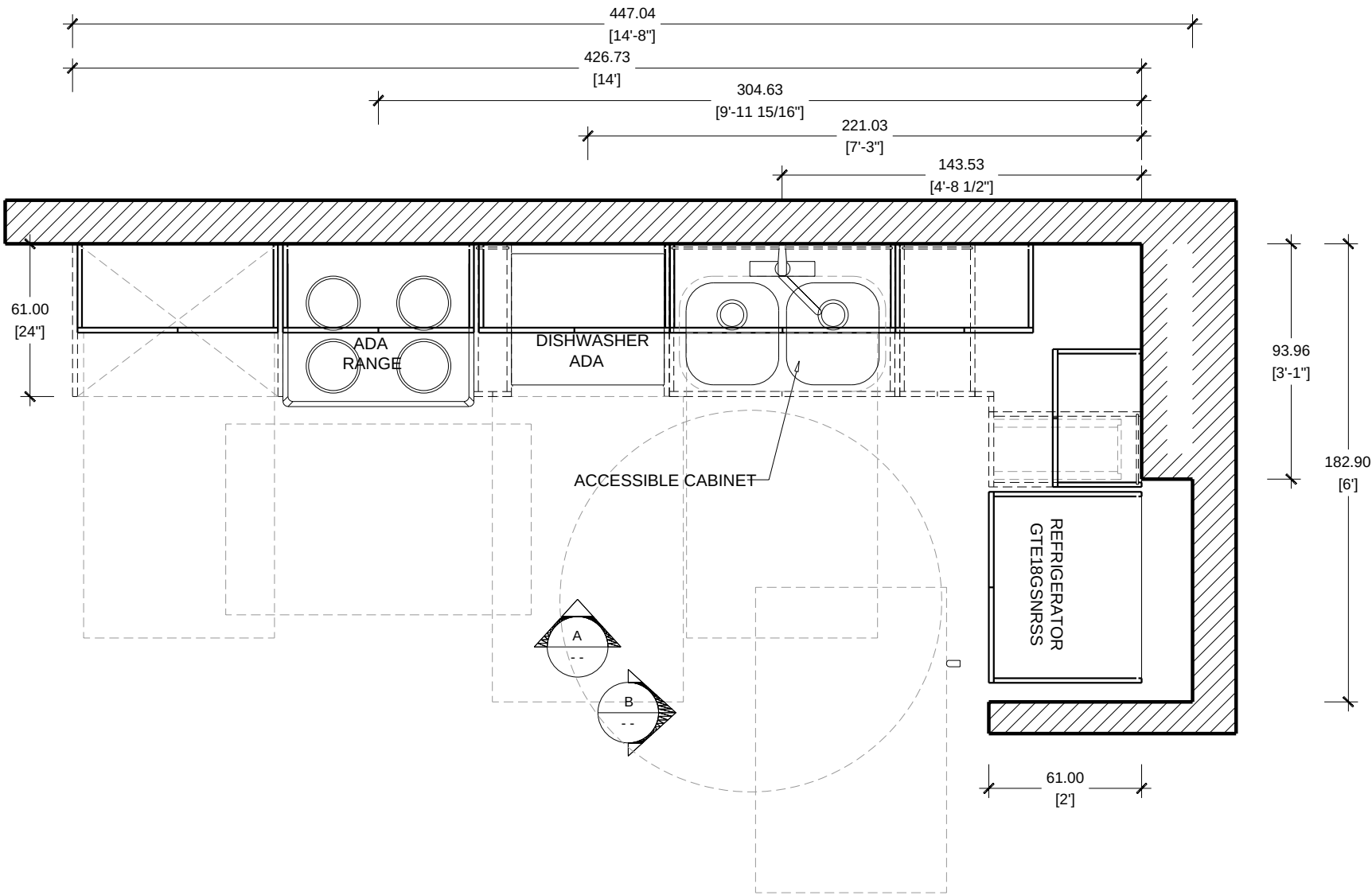
FLOOR PLAN SCALE 1/2"=1'-0" CASA FAMILIA UNIT A2 FA / KITCHEN TYPE K2 ADA
