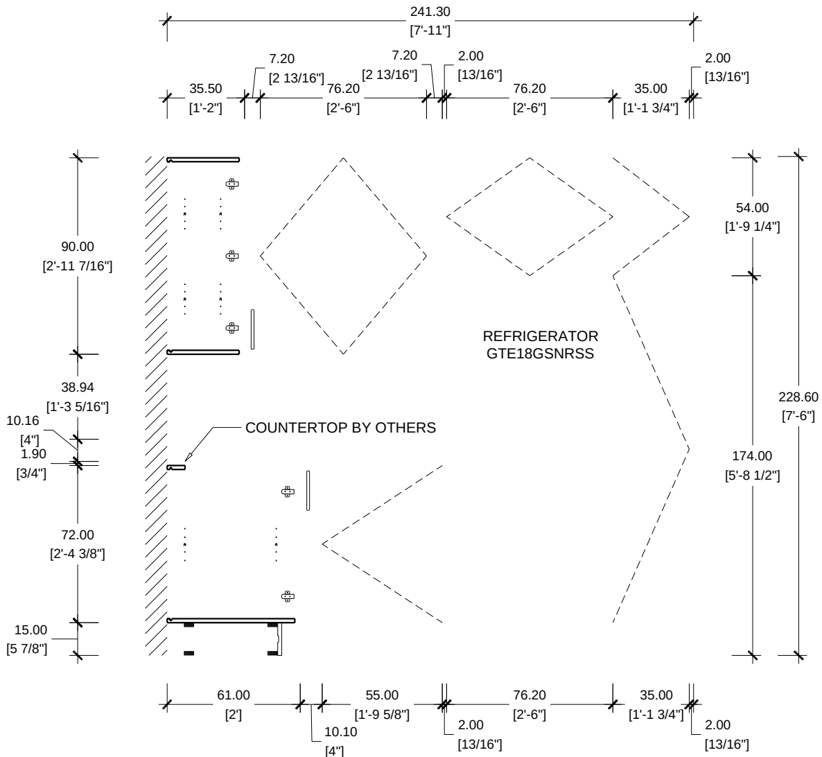
ELEVATION B CASA FAMILIA UNIT A3 / KITCHEN TYPE K1
