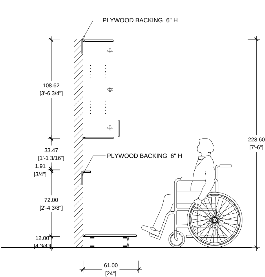
SECTION SCALE 1/2"=1'-0" KITCHEN ADA DRAWER
