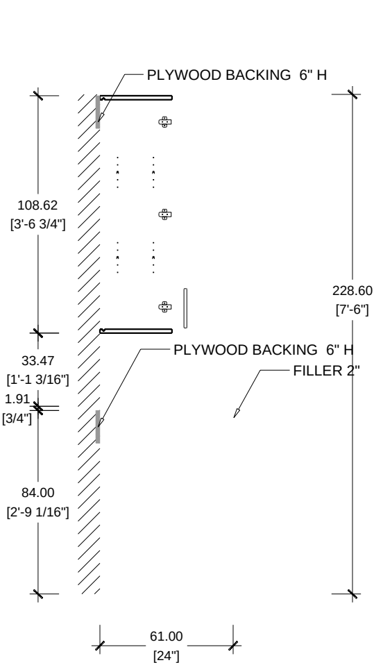
SECTION SCALE 1/2"=1'-0" KITCHEN ADA
