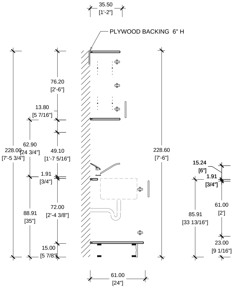
SECTION SCALE 1/2"=1'-0" KITCHEN
