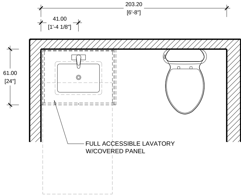
FLOOR PLAN SCALE 1/2"=1'-0" CASA FAMILIA UNIT A2 FA /VANITY TYPE V2
