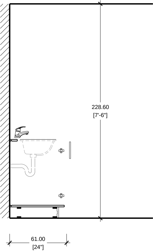
SECTION SCALE 1/2"=1'-0" VANITY
