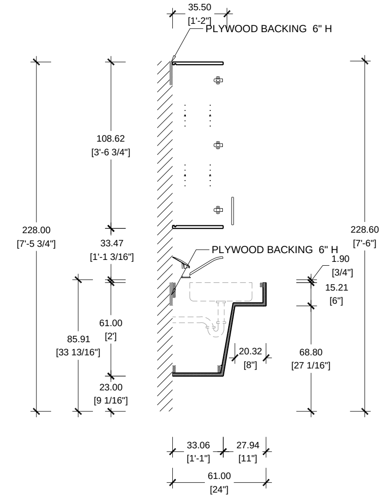
SECTION SCALE 1/2"=1'-0" KITCHEN ADA
