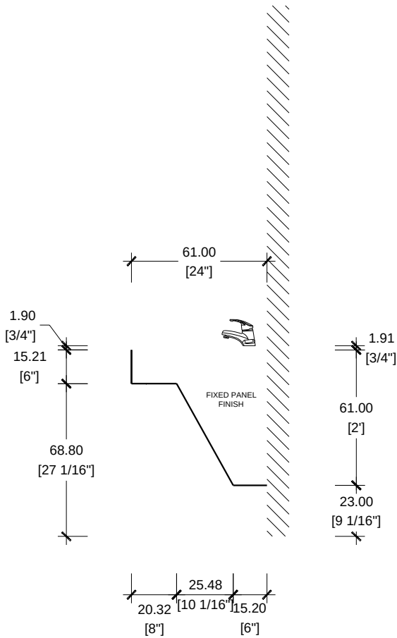
SIDE VIEW SCALE 1/2"=1'-0" CASA FAMILIA / VANITY TYPE V2
