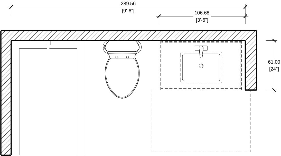
FLOOR PLAN SCALE 1/2"=1'-0" CASA FAMILIA /VANITY TYPE V3
