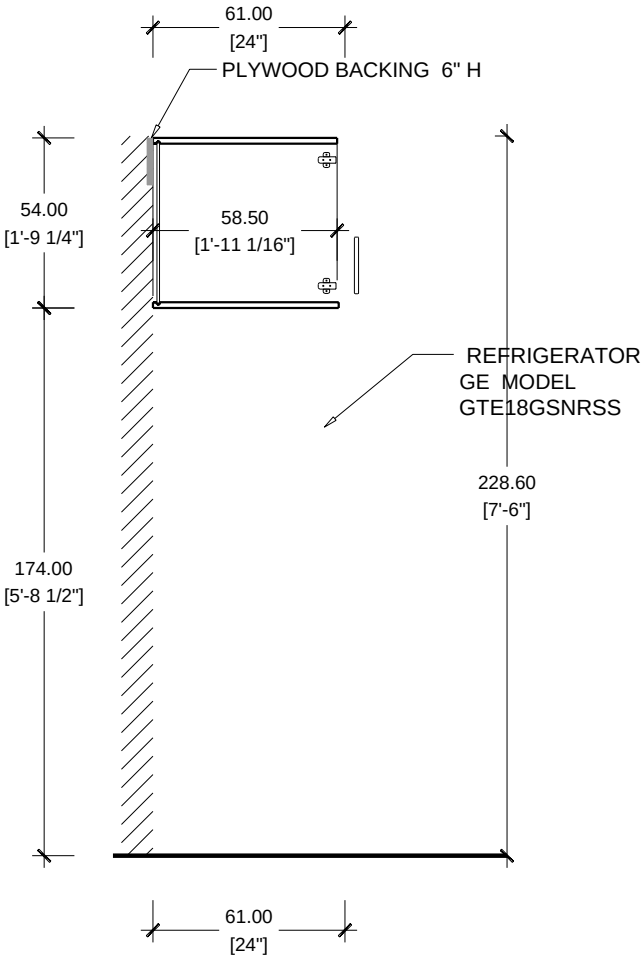
SECTION REFRIGERATOR SCALE 1/2"=1'-0" KITCHEN
