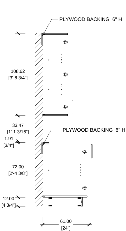
SECTION SCALE 1/2"=1'-0" KITCHEN ADA
