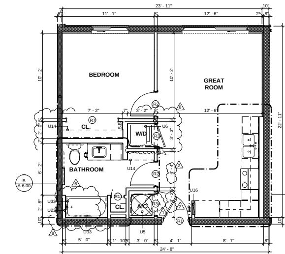
UNIT A-1 FLOOR PLAN SCALE: 1/4" = 1'-0"
