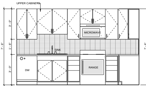
UNIT A-1 KITCHEN ELEV. SCALE: 1/2" = 1'-0"
