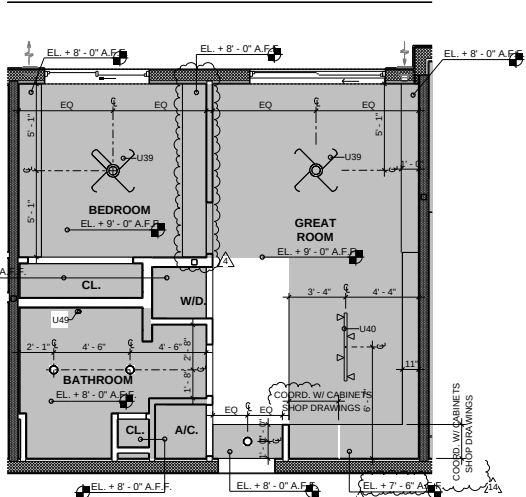
UNIT A-1 TYPICAL RCP SCALE: 1/4" = 1'-0"
