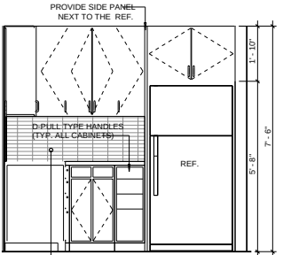
UNIT A-1 KITCHEN ELEV. SCALE: 1/2" = 1'-0"
