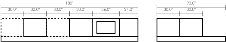
COUNTERTOP PLAN VIEW
