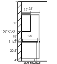
SIDE SECTION VIEW
