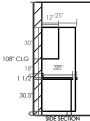
SIDE SECTION VIEW
