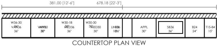
COUNTERTOP PLAN VIEW
