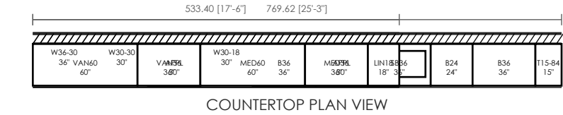
COUNTERTOP PLAN VIEW
