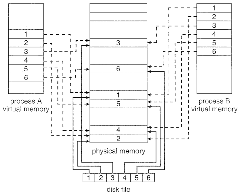
Figure 9.23 Memory-mapped files.
