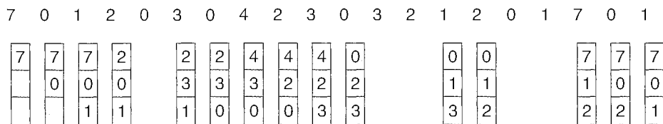
Figure 9.12 FIFO page-replacement algorithm.
