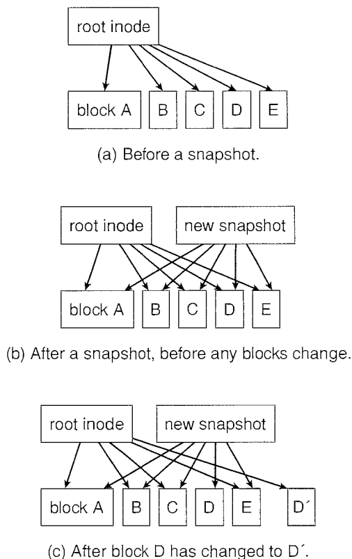
Figure 11.17 Snapshots in WAFL.
