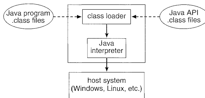
Figure 2.20 The Java virtual machine.
