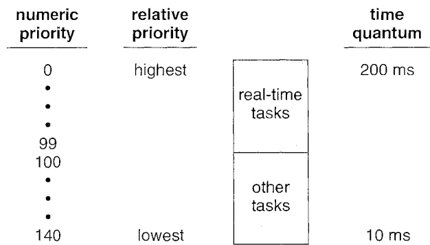
Figure 21.2 The relationship between priorities and time-slice length.
