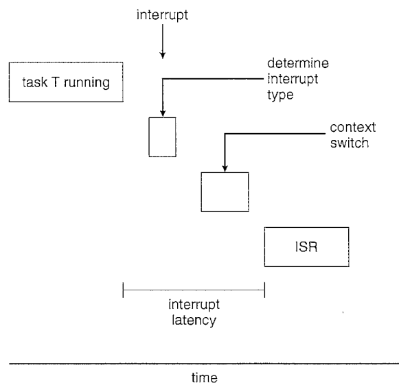
Figure 19.4 Interrupt latency.
