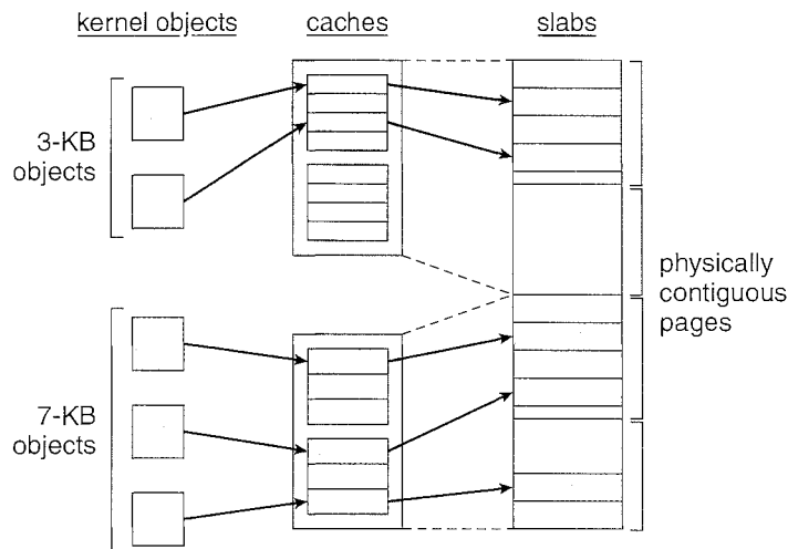
Figure 9.28 Slab allocation.
