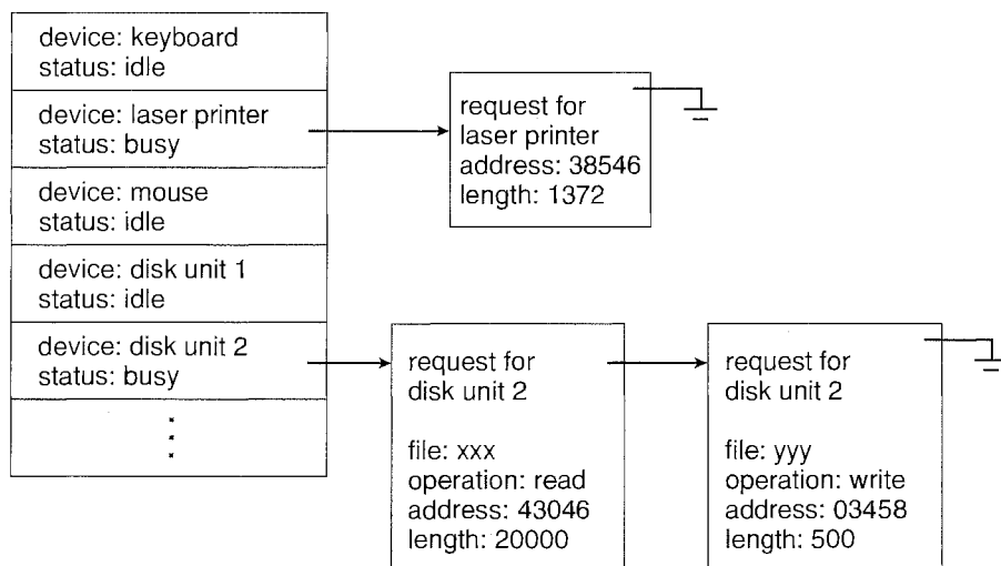
Figure 13.9 Device-status table.
