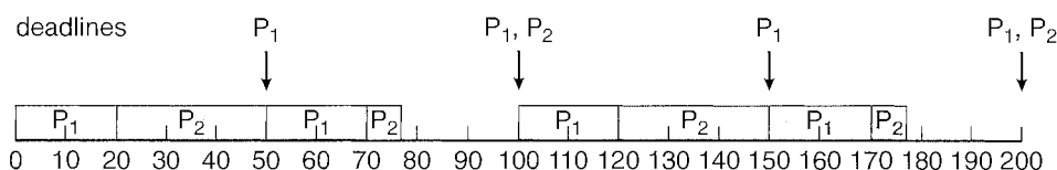
Figure 19.8 Rate-monotonic scheduling.
