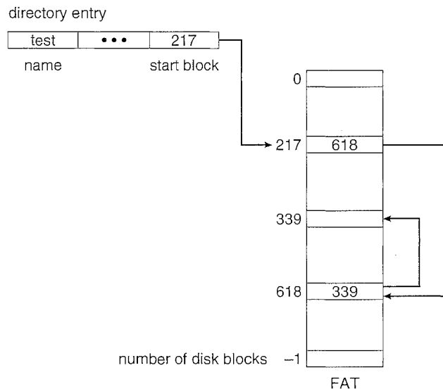
Figure 11.7 File-allocation table.
