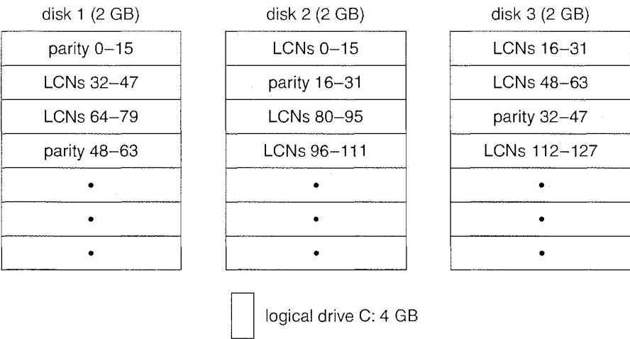
Figure 22.9 Stripe set with parity on three drives.
