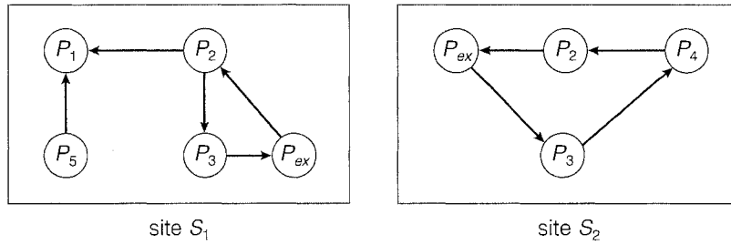
Figure 18.6 Augmented local wait-for graphs from Figure 18.3.
