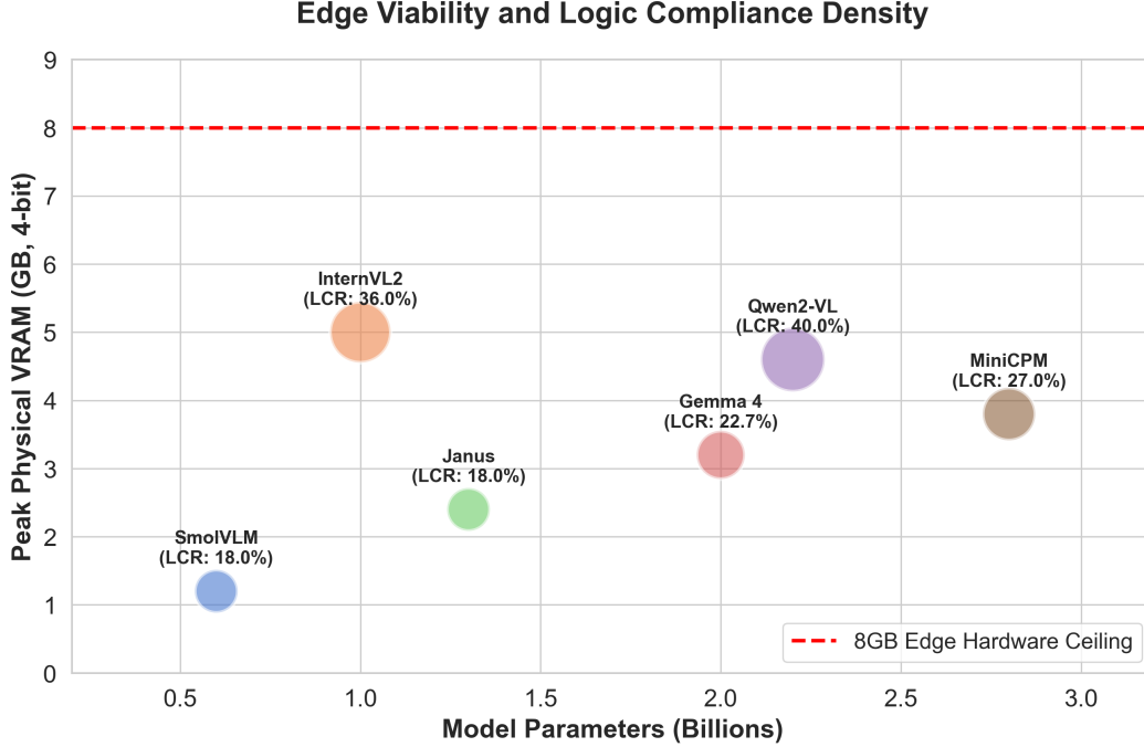
Figure 6: Edge hardware viability and memory footprint envelope. All six sub-3B architectures operate reliably beneath the 8 GB VRAM edge deployment threshold under 4-bit quantization, with Qwen2-VL and InternVL2 providing the strongest operational balance between footprint and reasoning capability.
