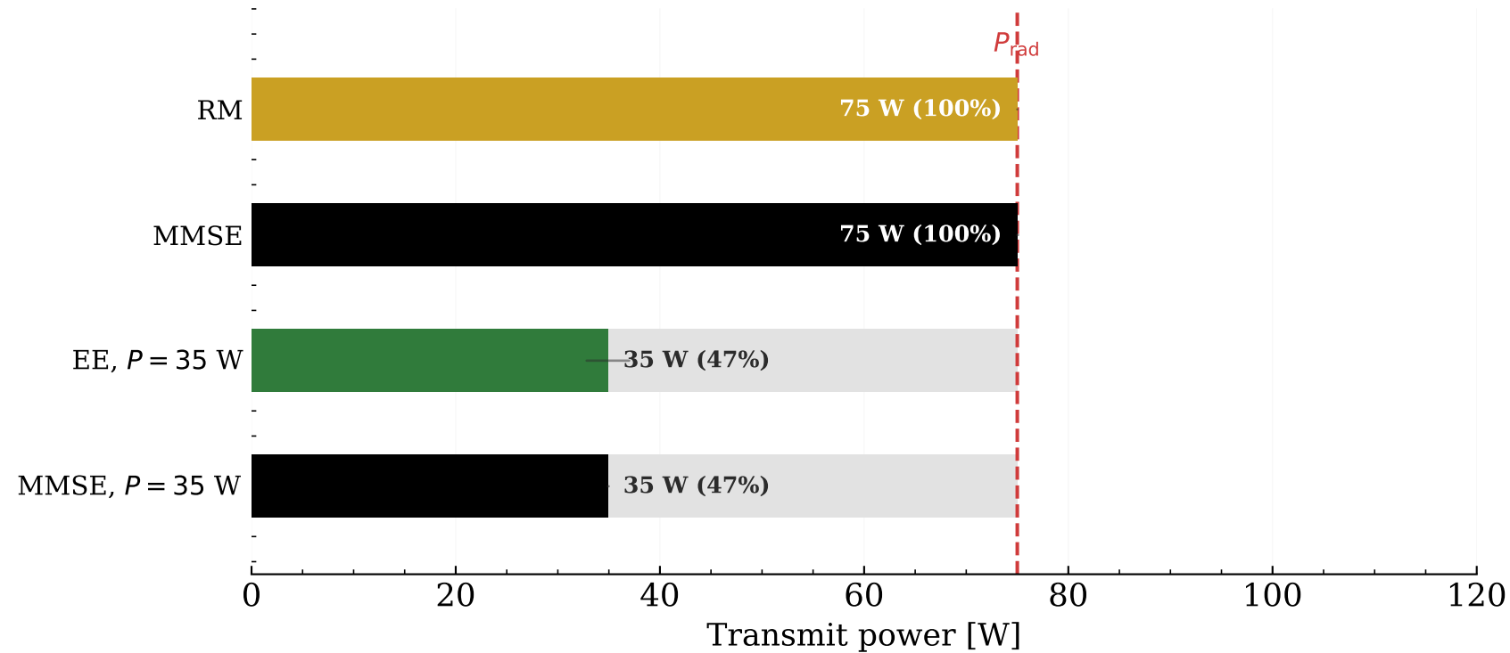
transmit power used vs. budget
