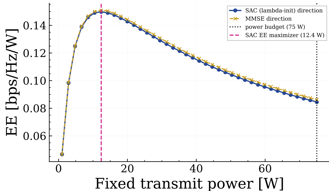
SAC (lambda-init) vs. MMSE direction, perfect CSIT
